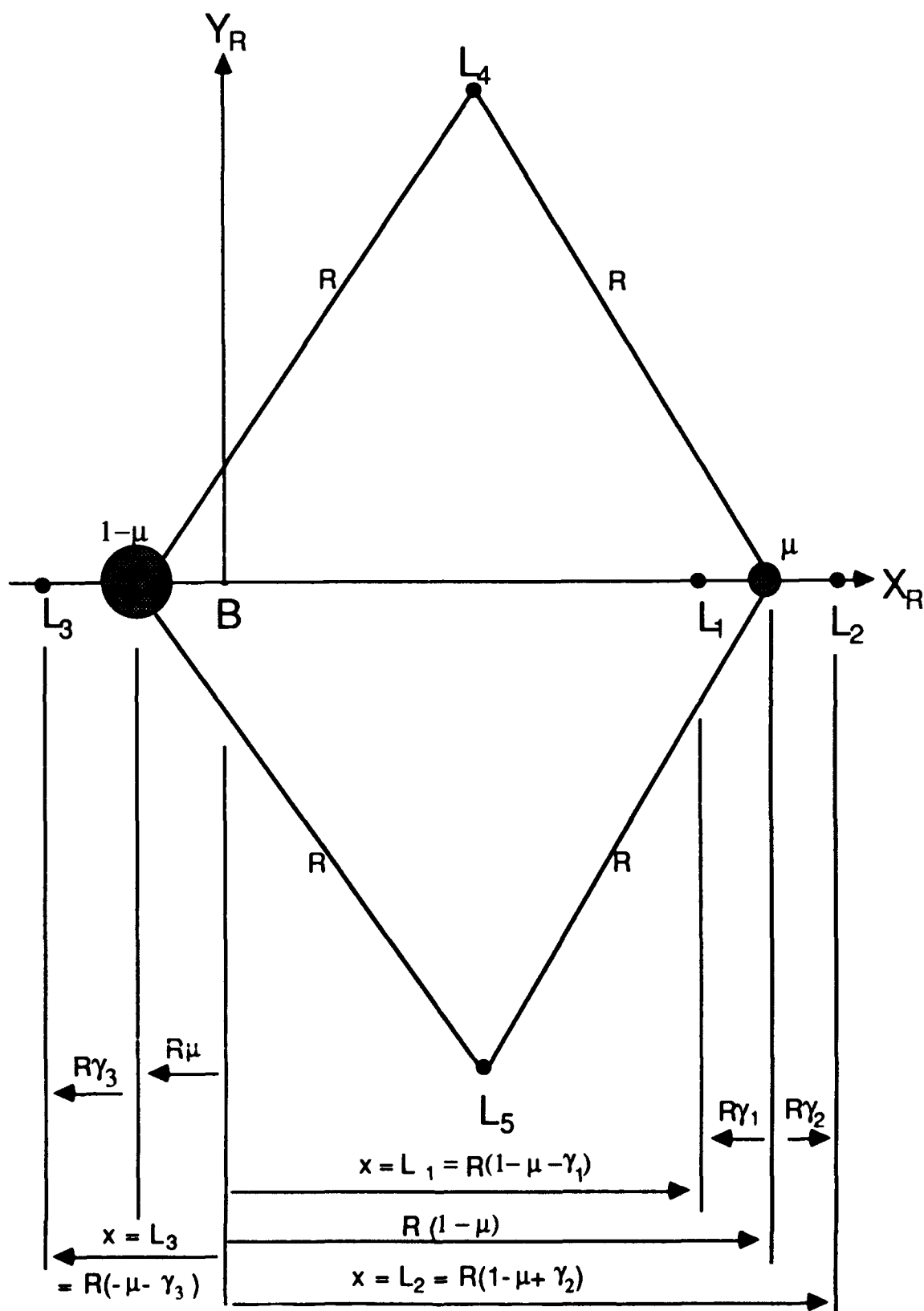
Figure 1-3. Lagrange Point Locations in the Scaled ER3BP.
