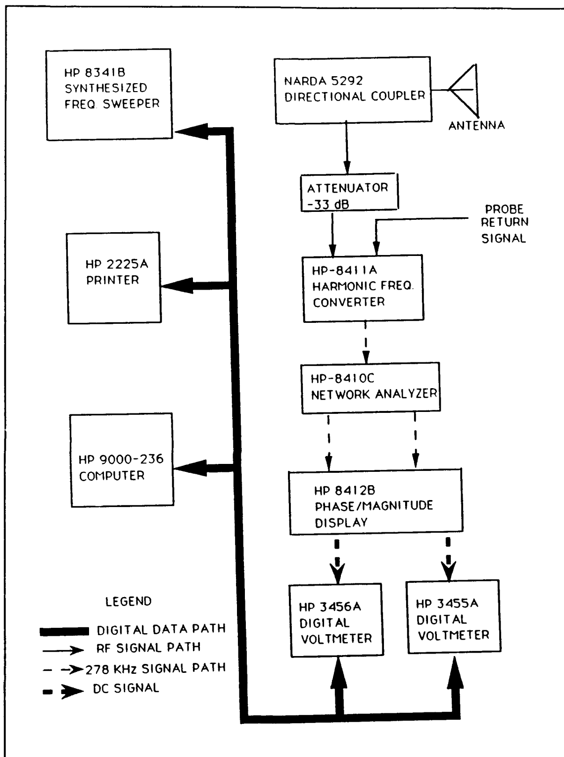
Figure 2.1 Measurement Flow Diagram
