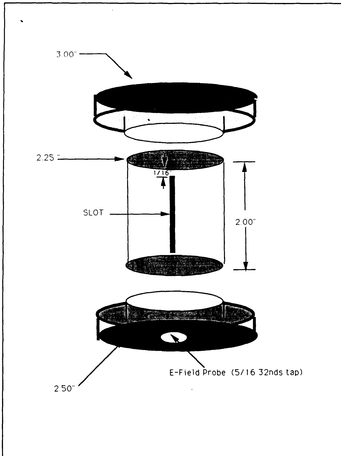
Figure 2.3 Cylinder Geometry
