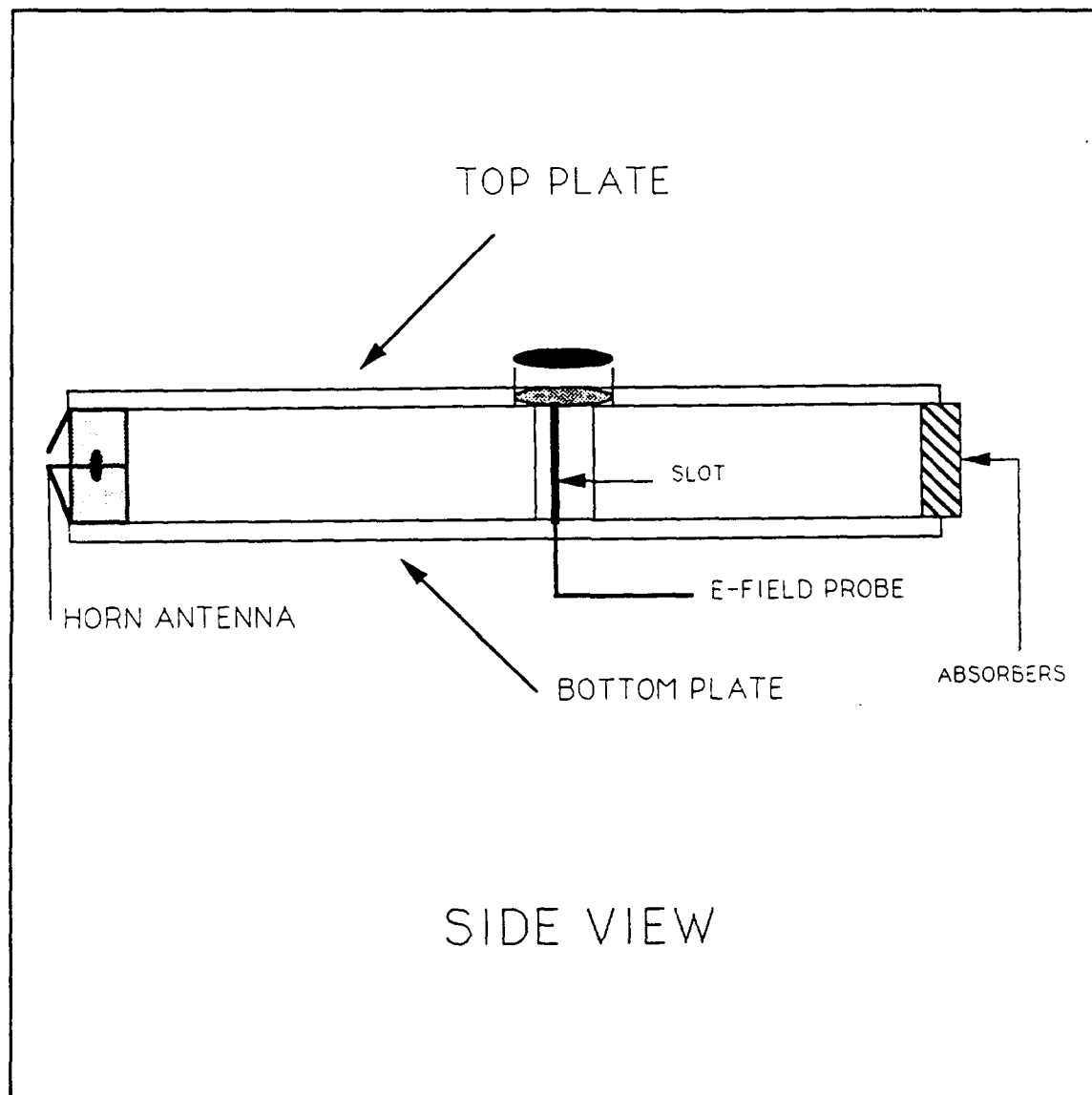
Figure 2.10 Measurement Configuration
