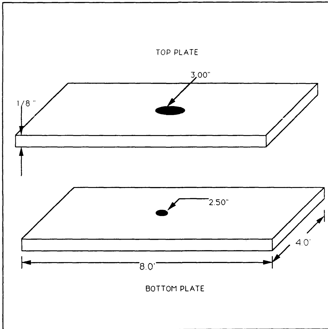
Figure 2.4 Plate Geometry
