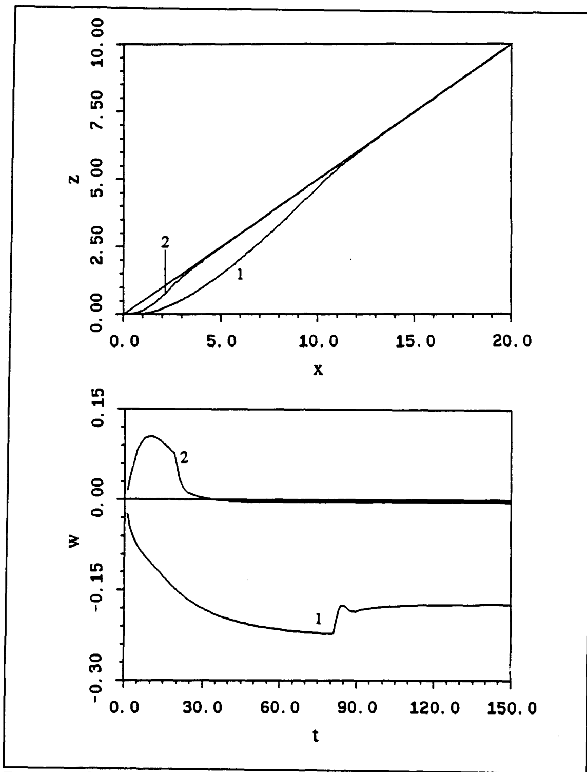
Figure 61. Runs 29 and 30 - Comparison of Path Keeping in the Vertical Plane with Stern Planes Only (Curves 1) and Stern & Bow Planes (Curves 2)
