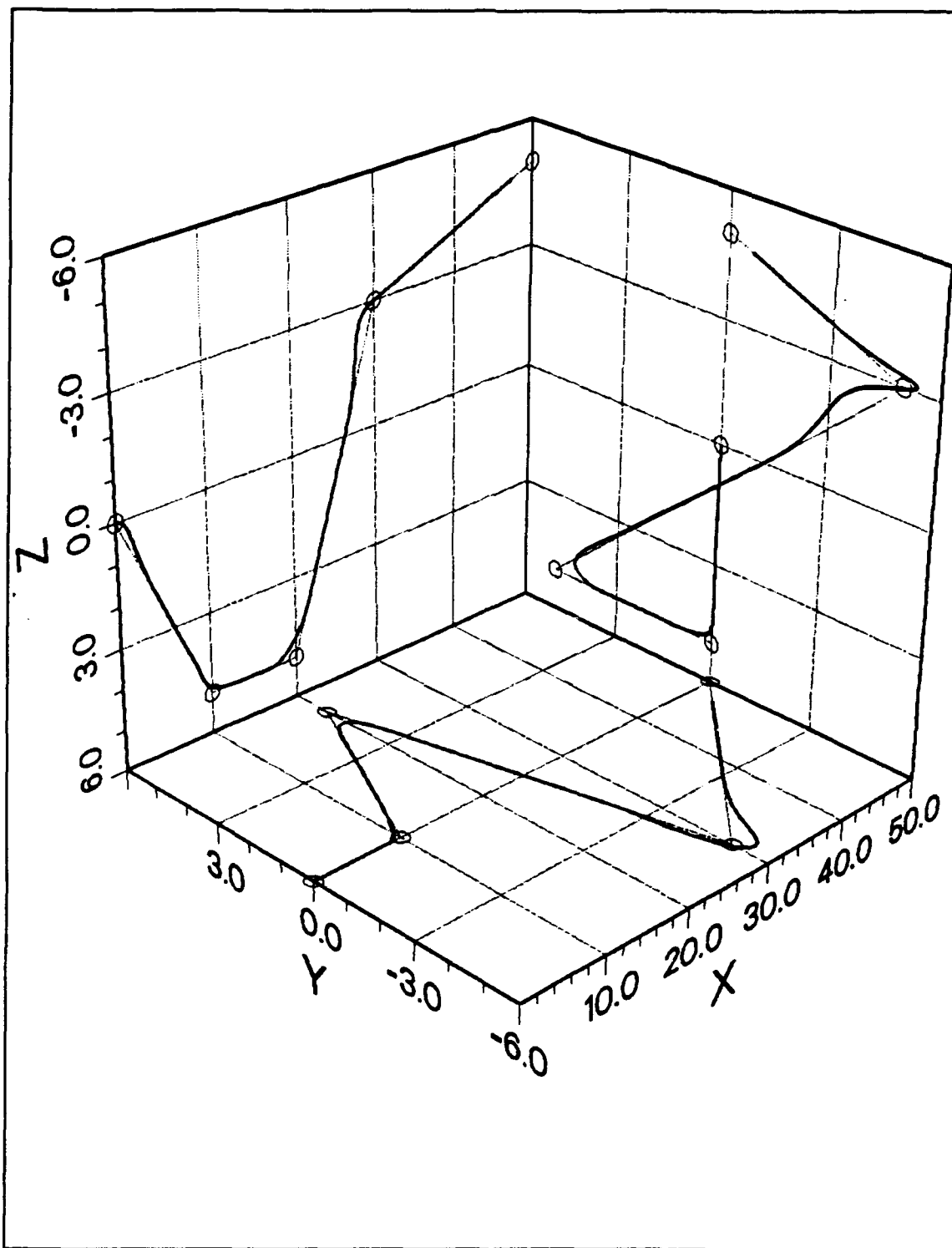
Figure 65. Run 31 - Three Dimensional Path Keeping at u = 3.0 ft/s
