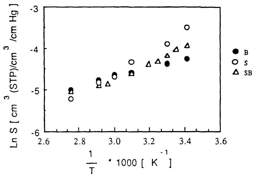
Figure 2-2. Temperature dependence of the equilibrium CO 2 solubility coefficients for S, B, and SB
