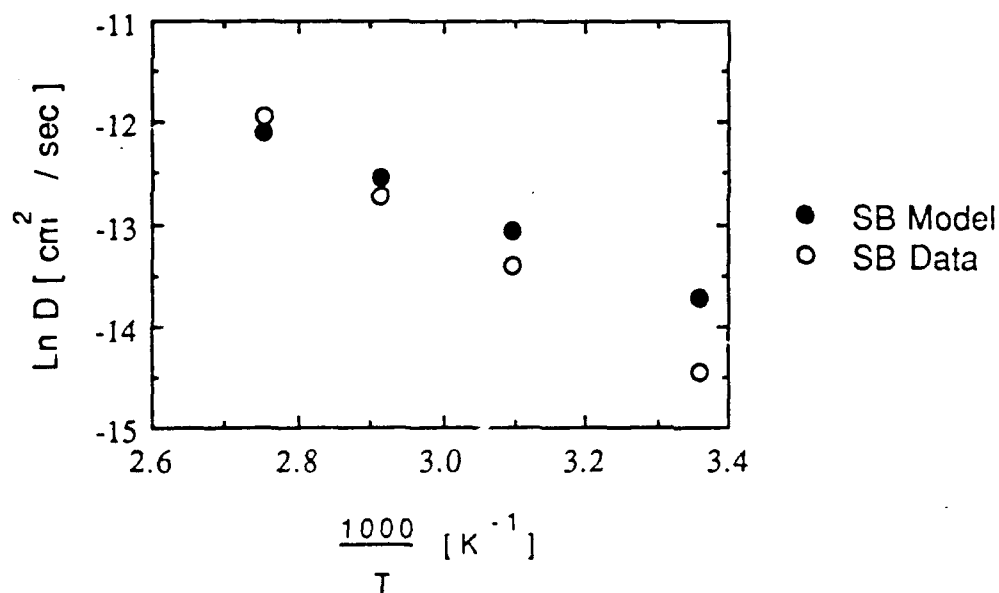
Figure 2-4b. Comparison of Arrhenius plots for measured and model generated Ar diffusion coefficients
