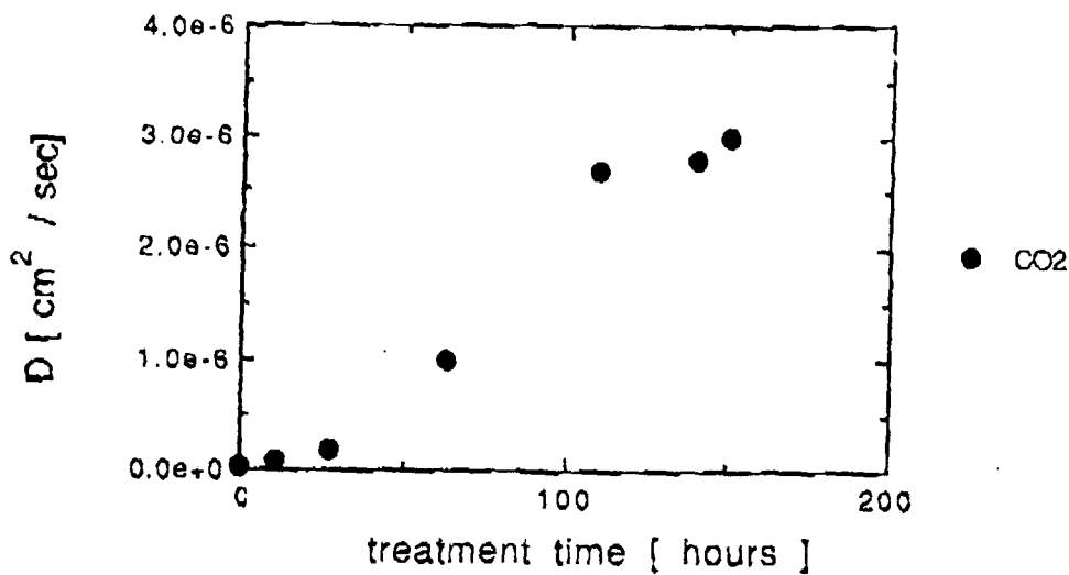
Figure 5.6 \text{CO}_2 diffusion in PSPMMA as a function of solvent treatment
