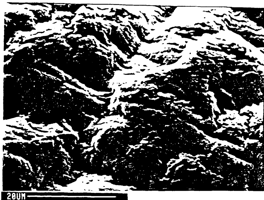
Figure 4-5a. SEM top view of PB film brominated to 14.3% extent of reaction
