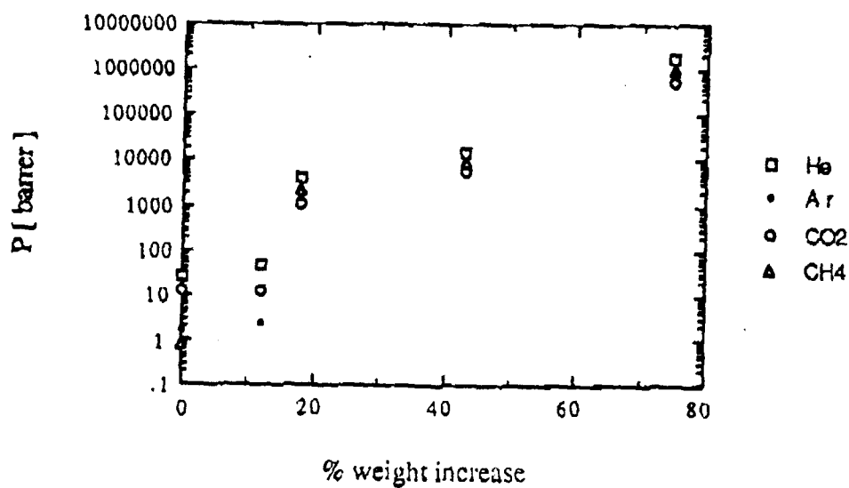
Figure 5.6 Gas permeability in PSPMMA as a function of solvent treatment
