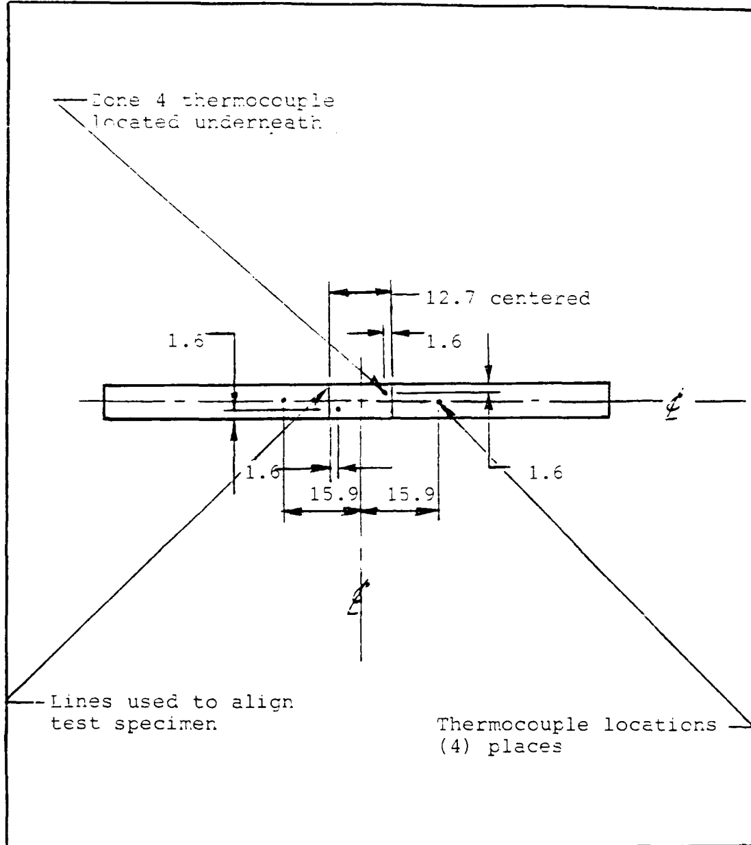
Figure 6 Test Specimen
