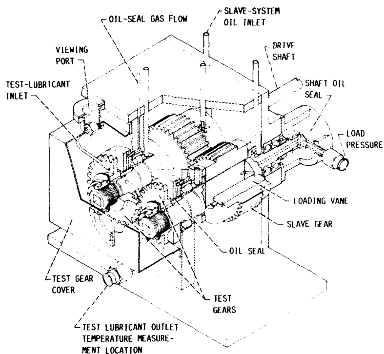
FIGURE 13. - SPUR GEAR TEST RIG.
