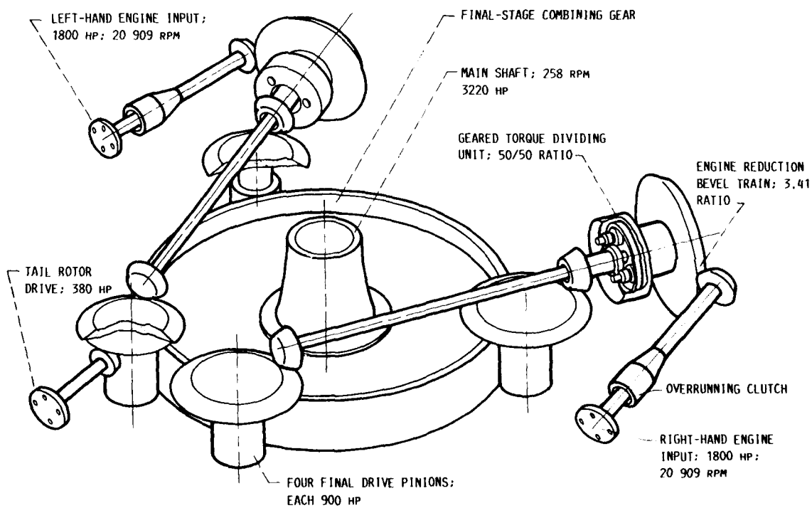
FIGURE 10. - SPLIT-TORQUE TRANSMISSION.
