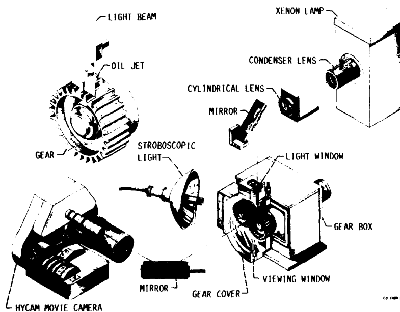
FIGURE 14. - TEST APPARATUS FOR OIL JET PENETRATION STUDIES.
