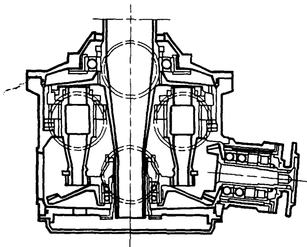
FIGURE 9. - SELF-ALIGNING, BEARINGLESS PLANETARY TRANSMISSION.
