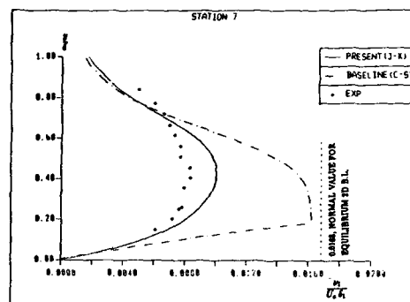
Fig. 4) Comparison of the eddy-viscosity profiles at Station 7.
