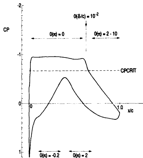
Fig. 5 Typical pressure distribution on a modern airfoil section and associated levels of the B.L. pressure gradient parameter, \pi = (\delta^*/r_w) (dp/dx)
