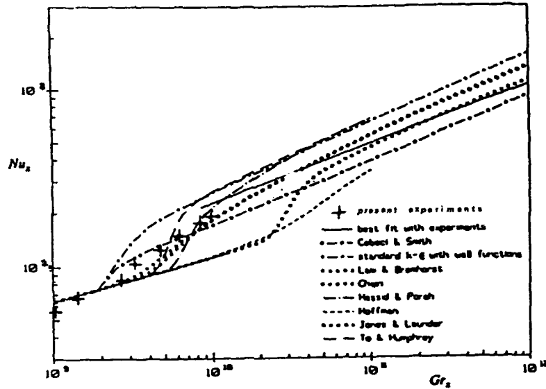
Fig. 1. Computed and measured wall heat transfer for air. Henkes and Hoogendoorn ref. (28)
