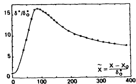
Figure 22a : Calculations of a boundary layer/shock-wave interaction with an inverse boundary layer method - M_{\infty} = 1.36 The experimental displacement thickness distribution is used as an input of the method From BENAY et al.
