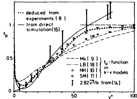
Fig. 1: f_\mu -function in low-Re k- \epsilon models
