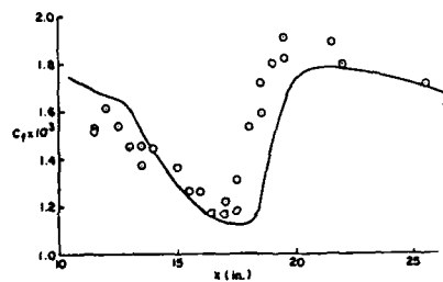
Figure 15 : Calculations of COLEMAN et al. experiments taking into account the transition region from ARNAL
