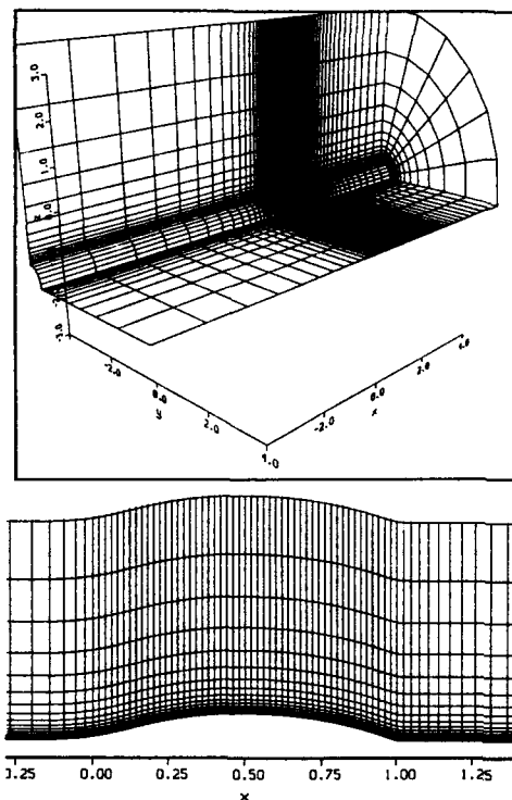
Fig. 7) The finite-difference grid ( 61 \times 7 \times 41 ) for simulating the Bachalo and Johnson 2 axisymmetric bump experiment.
