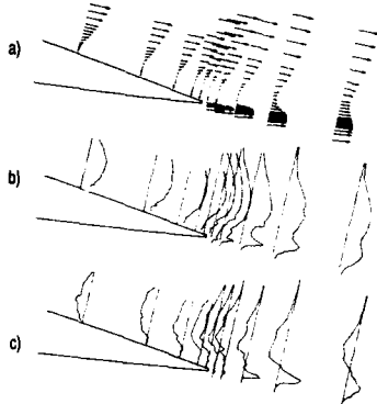
Fig. 4 Some hot-wire measurement results near an oscillating airfoil in the Brussel Free University 1 \times 2 \text{ m}^2 wind tunnel
