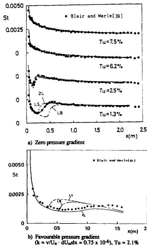
Fig. 8: Stanton number St in transitional boundary layers, from [25, 26], key to models see Fig. 4
