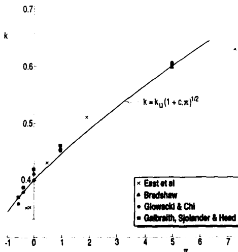
Fig. 7 Effect of pressure gradient on value of k in l = k \cdot y for equilibrium boundary layers
