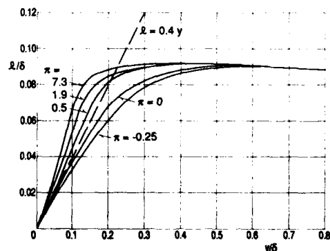
Fig. 6 Mixing lengths deduced from turbulent shear stress measurements in equilibrium boundary layers at various pressure gradients (East et al, 1979)
