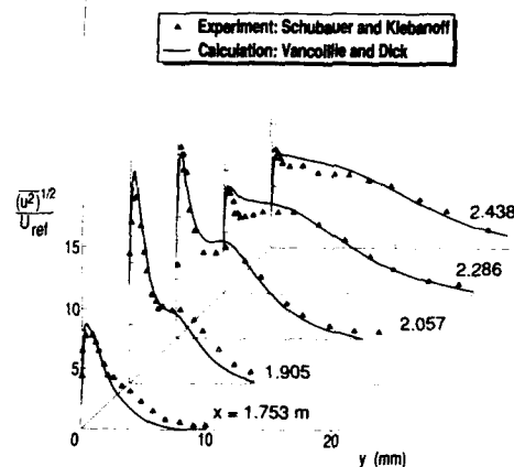
Fig. 3 Turbulence intensity in a boundary layer transition region. Comparison between experiment and calculations at Ghent University based on a turbulence model with an allowance for intermittency
