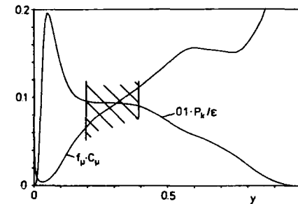
Fig. 2: Distribution of c_\mu f_\mu and P_k/\epsilon in channel from direct simulation [15]
