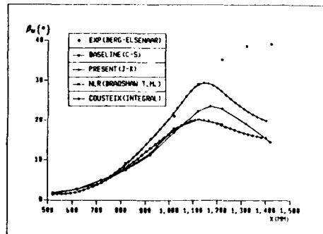
Fig. 2) The wall streamline angle relative to the boundary-layer edge streamline.
