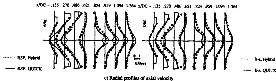
Fig. 9: 3D flow in combustor model, lines are calculations [46], o experiments [45]
