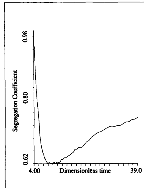
Figure 8. Evolution of the segregation coefficient. The approximate experimental value 5 is 0.7. ( Kc = 47.5 l/mol s).
