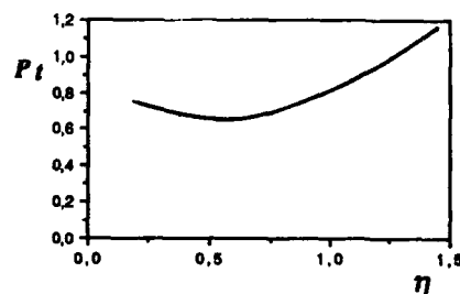
Figure 8b : Prandtl number in a plane jet From FULACHIER-ANTONIA
