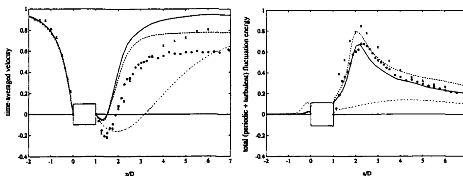
b) Distribution of time-averaged velocity and total kinetic energy of fluctuations (periodic + turbulent) along centre line. Calculations [47]: --- 2 layer k- \epsilon model, — RSE model with wall functions, --- 2 layer RSE model; experiments: o Lyn [48] Re = 22000 , x Durao et al. [49] Re = 14000
