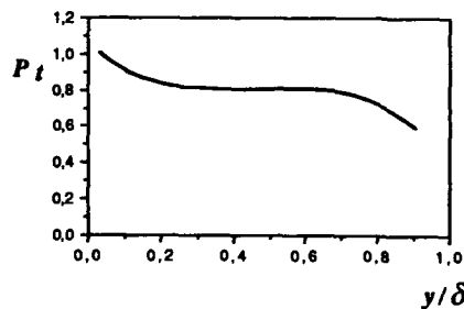
Figure 8a : Prandtl number in a boundary layer From MEIER-ROTTA
