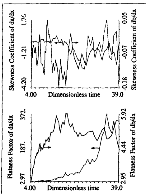
Figure 10. Evolution of the skewness coefficients and flatness factor of two reactive scalar gradients (downstream direction derivative) ( Kc = 47.5 l/mol s).
