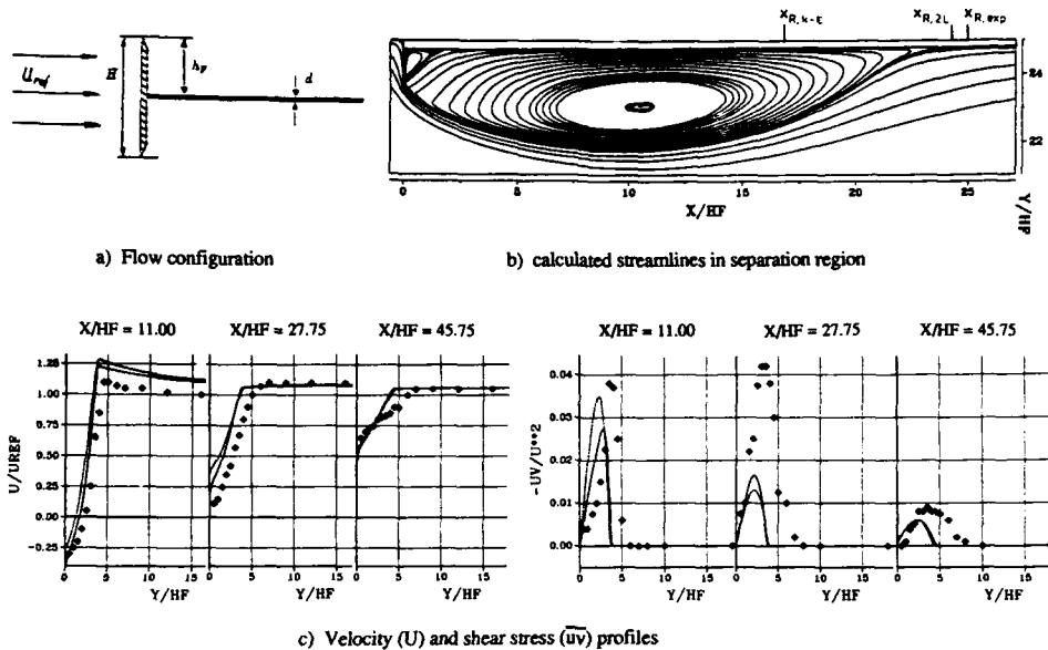
Fig. 6: Flow over T-configuration; — Calculations with 2-layer model [32], --- Calculations with standard k- \epsilon model [32], \diamond experiments [33]
