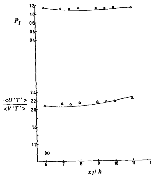
Figure 21 : Scalar turbulence in a nearly homogeneous shear flow with a linear mean temperature gradient Experiment : TAVOULARIS-CORRSIN Calculations : JONES-MUSONGE
