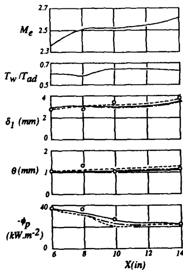
Figure 16 : Calculation of CLUTTER-KAUPS experiments - integral method --- mixing length ... k - ε model (JONES-LAUENDER)
