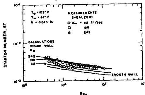
Figure 20 : Calculations of the heat transfer coefficient on a roughened flat plate By FINSON-WU
