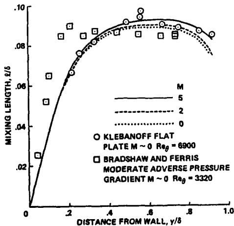
Figure 2 : Effect of Mach number on the mixing length distribution from MAISE and McDonald. Figure taken from MARVIN-COAKLEY
