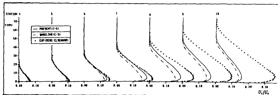
Fig. 6) The crossflow velocity profiles of the computation and measurement.
