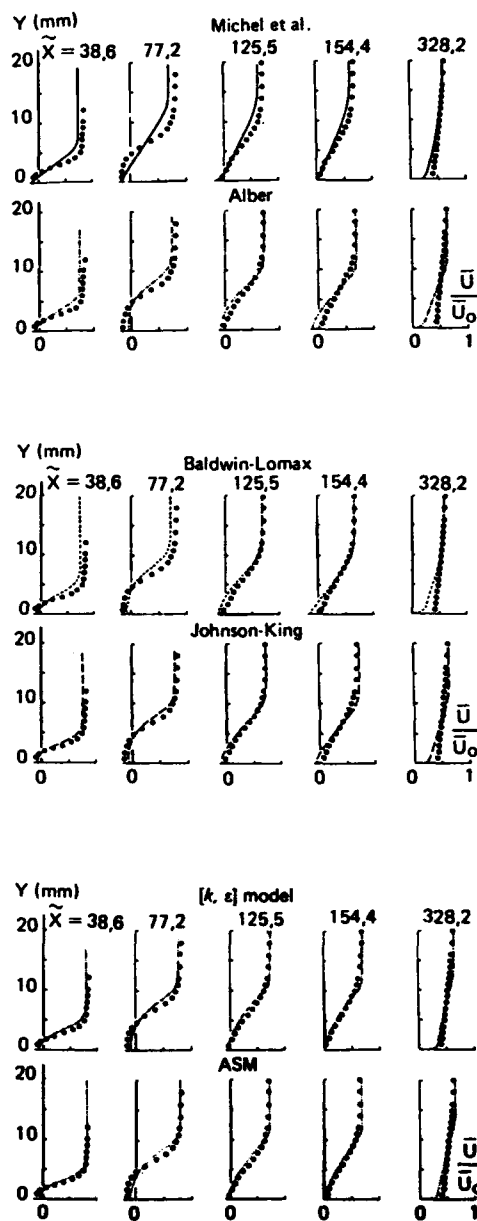
Figure 22c : Comparison between calculated and experimental boundary layer velocity profiles
