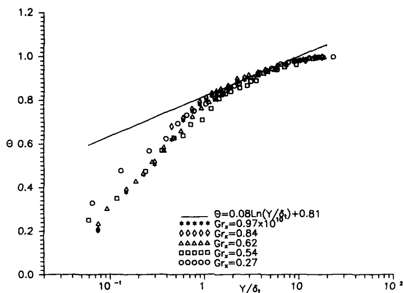
Fig. 3 Temperature profiles in a developing turbulent natural convection boundary layer along a vertical surface - outer part.
