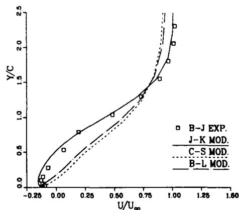
Fig. 11) The boundary-layer mean velocity profiles at the trailing-edge s/c = 1.0 .
