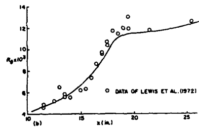
Figure 17 : Calculations of LEWIS et al. experiments by CEBECI-SMITH
