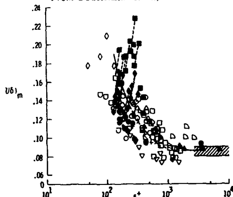
Figure 5a : Variation of the outer level of the mixing length downstream of natural transition on plates, cones and cylinders From BUSHNELL et al.
