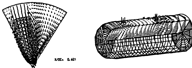
a) Geometry and velocity field predicted with RSE model
