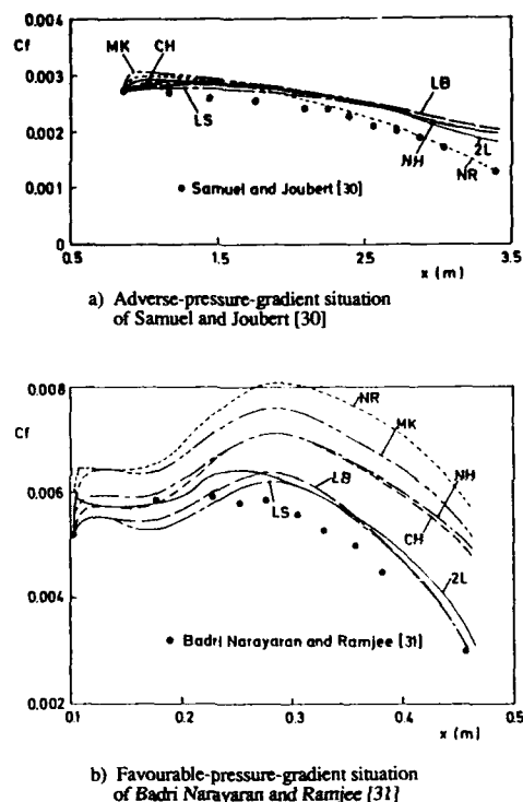
Fig. 4: Friction coefficient in boundary layers with streamwise pressure gradient, from [25, 26]; NR = Norris-Reynolds [24] one-equation model, LB = Lam-Bremhorst [18], LS = Launder-Sharma [36], CH = Chien [21], NH = Nagano-Hishida [10], MK = Myong-Kasagi [9] low-Re- k - \epsilon models, 2L = two-layer model.
