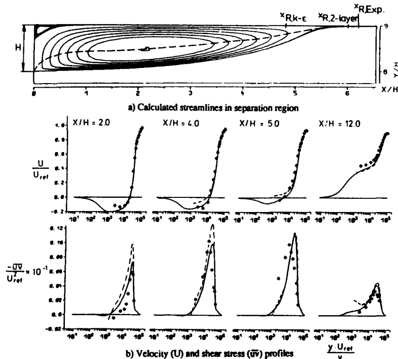
Fig. 5: Flow over backward-facing step with aspect ratio of 1.125 — Calculations with 2-layer model [28], --- Calculations with standard k - \epsilon model [28], \circ experiments [29]
