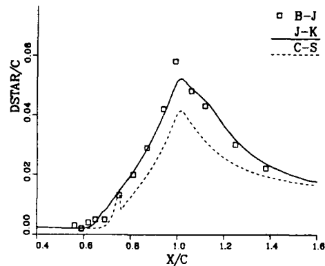
Fig. 9) The displacement thicknesses.
