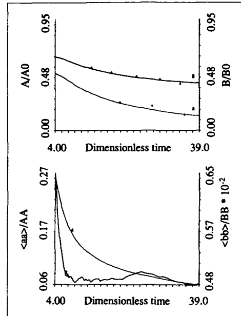
Figure 7. Evolution of means and variances of two reactive scalars. Comparison with Benanni et al. 5 experimental data ( Kc = 47.5 l/mol s).
