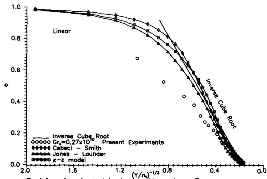
Fig. 4 Comparison of computed and measured temperature profiles. Non-fully developed flow.
