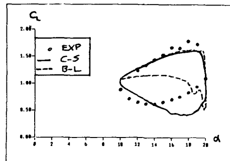
Fig. 14) Coefficient of lift hysteresis using the Baldwin-Lomax and Cebeci-Smith turbulence models, deep stall: \alpha(t) = 15^\circ + 5^\circ \sin(2M_\infty kt) ( k = 0.5 , M_\infty = 0.3 , Re_\infty = 4 \times 10^6 ).
