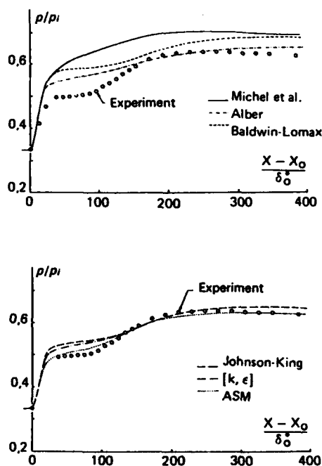
Figure 22b : Comparison between calculated and experimental pressure distribution
