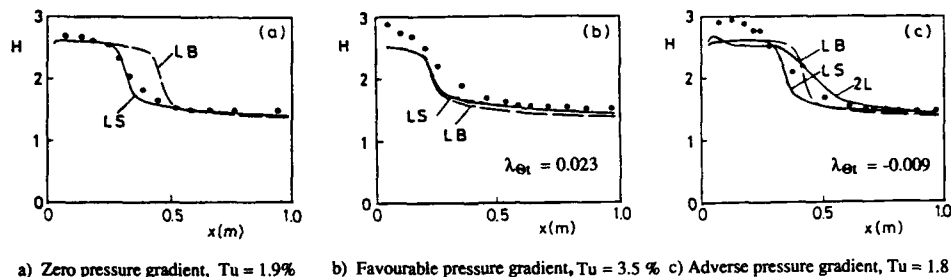
Fig. 7: Shape factor H in transitional boundary layers, from [25, 26], • experiments [37], key to model see Fig. 4
