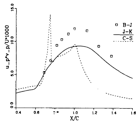
Fig. 10) The streamwise variation of the maximum shear stress.
