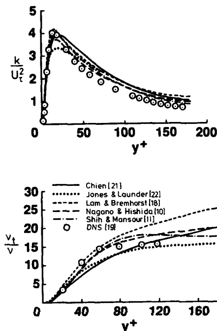
Fig. 3: Near-wall kinetic energy ( k ) and eddy-viscosity ( v_t ) distributions in low Re channel flow, from [20]
