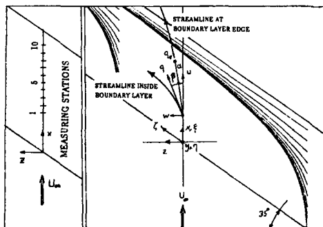
Fig. 1) The wall streamlines and related angles for the infinite swept wing experiment of Berg and Elsenaar.
