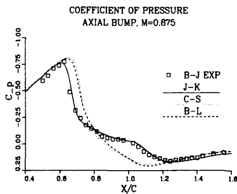
Fig. 8) The coefficient of pressure: M_\infty = 0.875 , Re_\infty = 13.6 \times 10^6/m (B-L, Baldwin-Lomax, C-S, Cebeci-Smith, J-K Johnson-King models).
