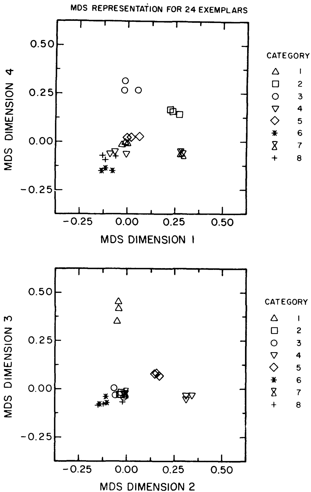
Figure 1. SINDSCAL representation for the twenty-four exemplars. Fig. 1a plots values on Dimension 4 vs. values on Dimension 1; Fig. 1b plots values on Dimension 3 vs. values on Dimension 2. The different symbols represent the eight different stimulus categories. Three exemplars from each category are shown.
