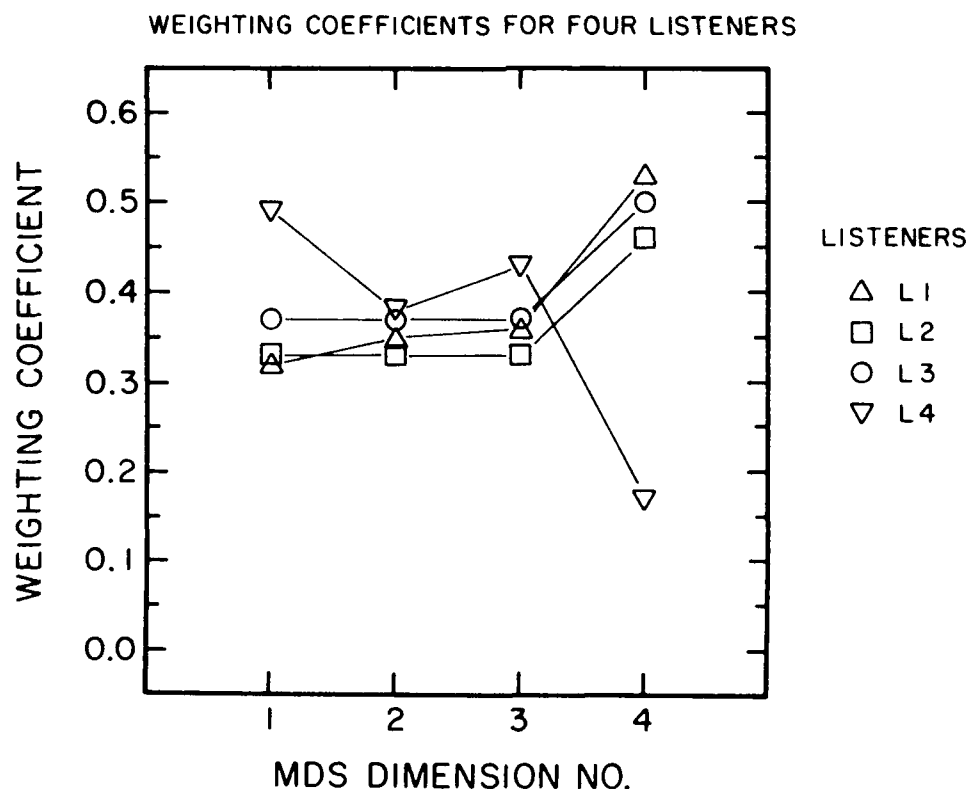
Figure 2. Dimensional weighting coefficients for the classification of the original signals. The different symbols represent the four listeners.
