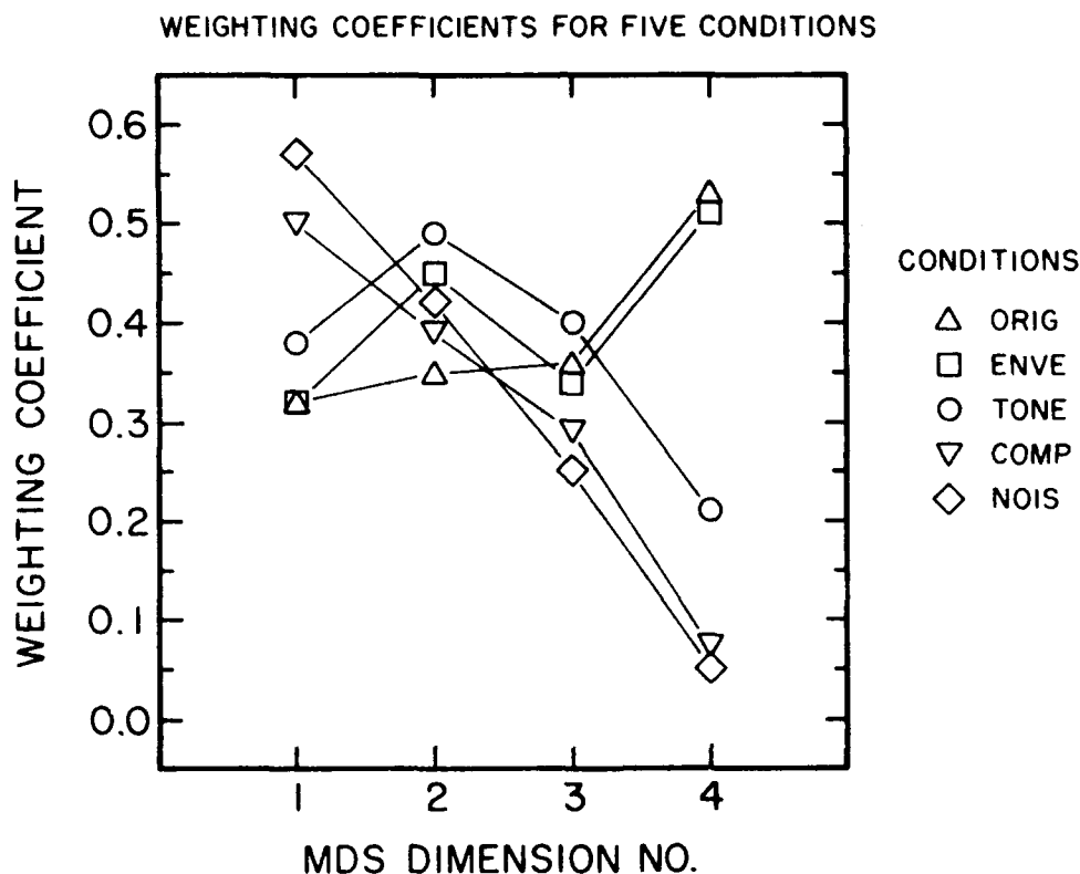
Figure 3. Dimensional weighting coefficients for L1. The different symbols represent the five stimulus conditions.
