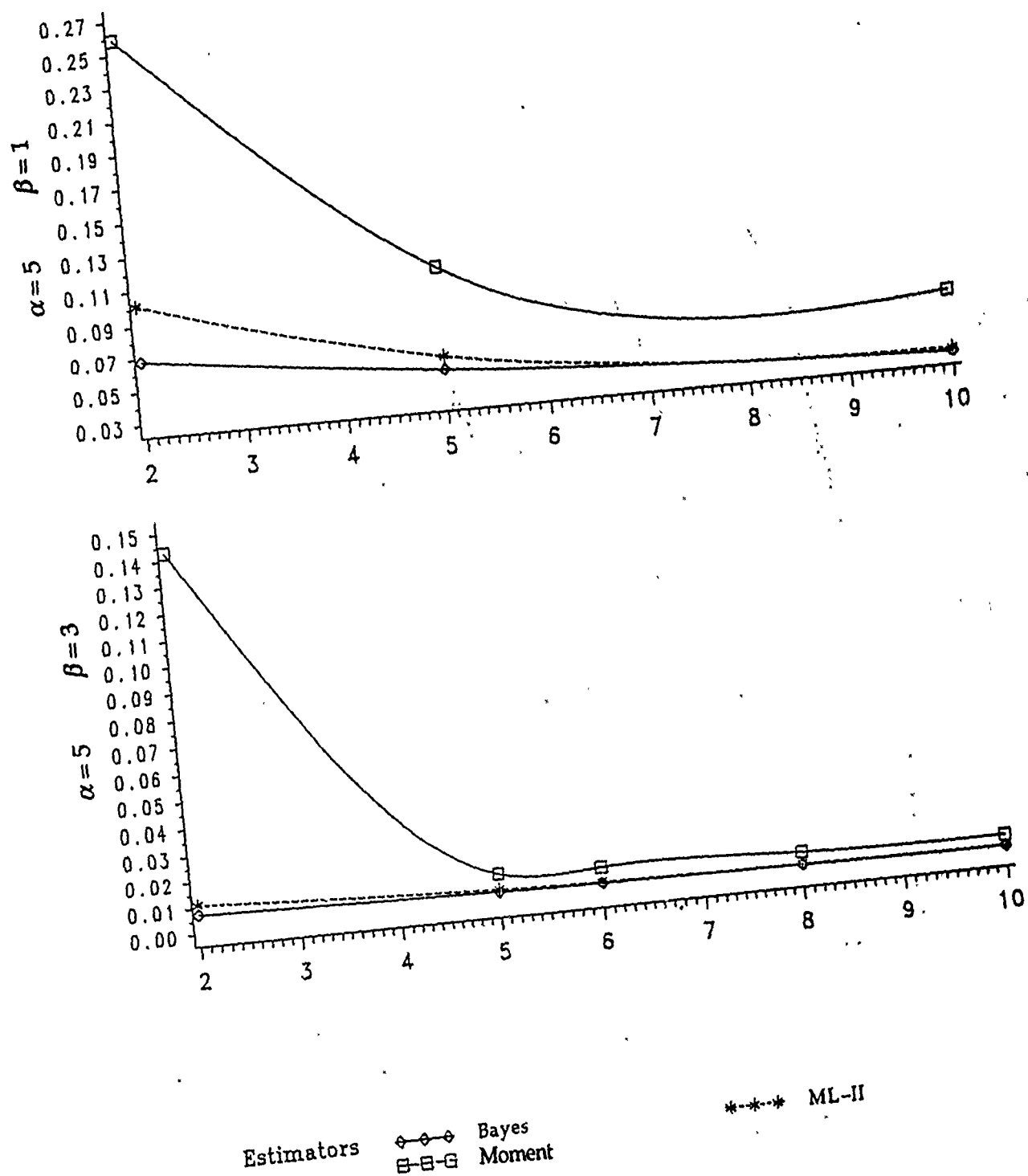
Figure 3. EB risks of the three estimators are plotted versus r for two configurations when \beta is known.
