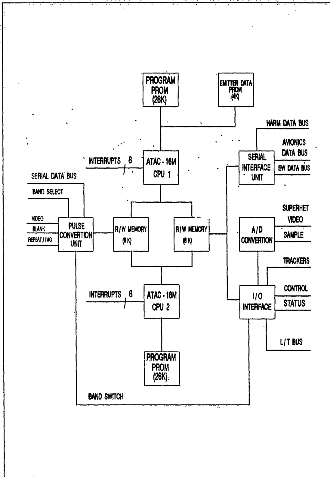
Figure 14: ALR-67 Processor (CP-1293)
