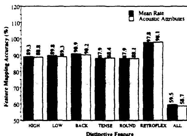
Figure 3.3: Distinctive Features Mapping Accuracies for the Mean Rate Response and Acoustic Attributes
