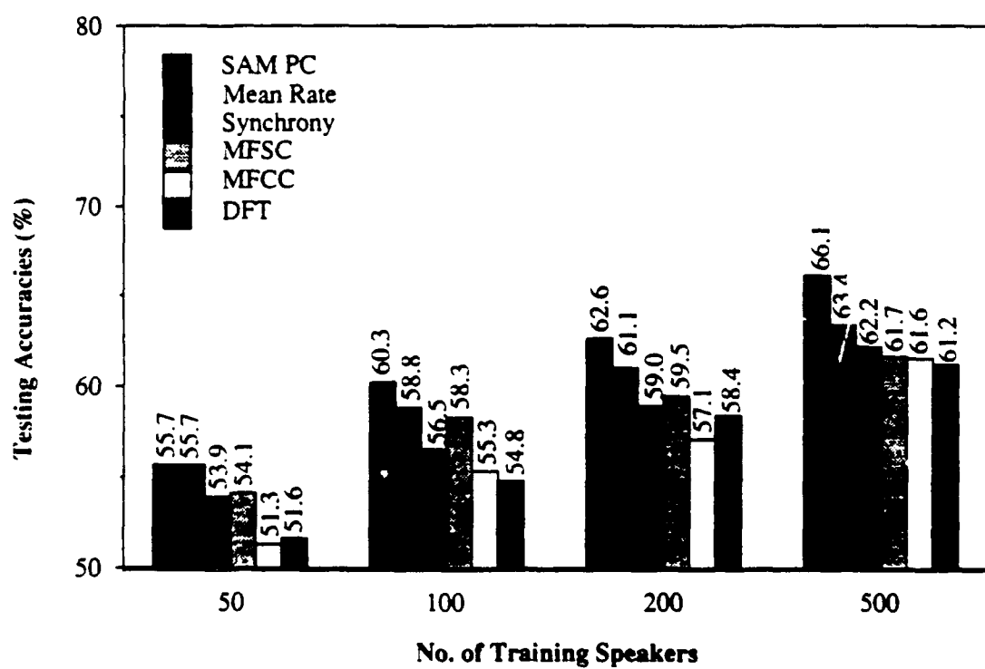
Figure B.1: Overall comparison results for the six acoustic representations
