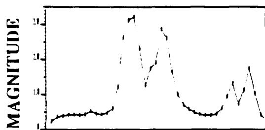
Clean Speech
