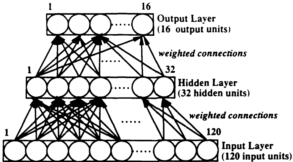
Figure 2.6: Structure of the Multi-Layer Perceptron Classifier
