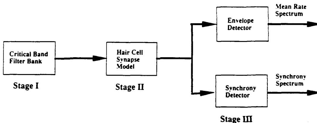
Figure 2.1: Block diagram of Seneff's auditory model
