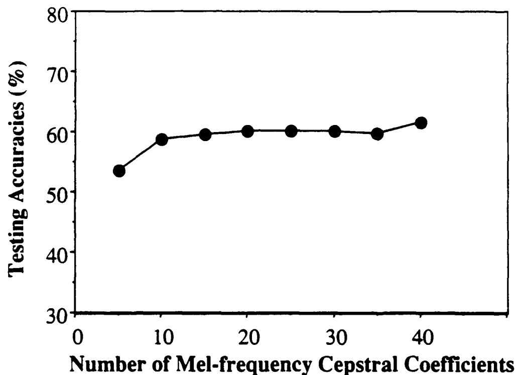
Figure 2.10: Effect of Varying the Number of MFCC on Vowel Classification Performance
