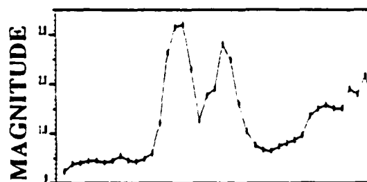
Noisy Speech
