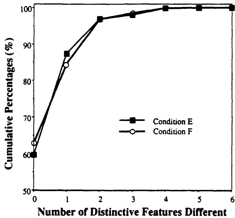
Figure 3.8: Performance of conditions E and F in terms of the number of features different between network outputs and transcription labels
