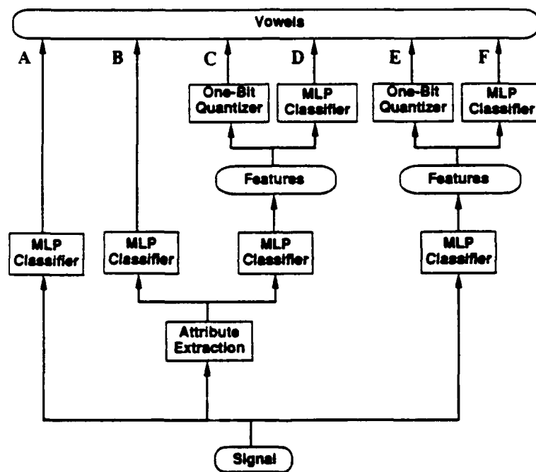
Figure 3.1: Experimental paradigm comparing direct phonetic classification with attribute extraction, and the use of linguistic features.
