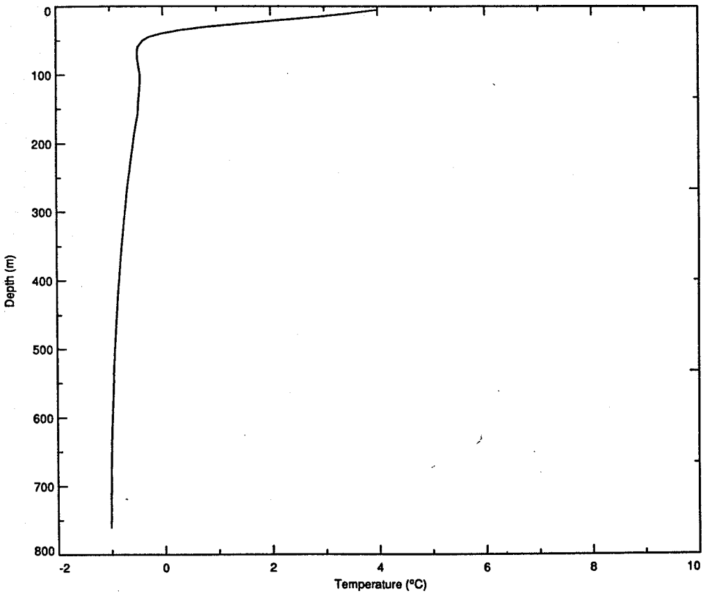
Figure 4.16. Average of all XBT profiles from 1989.
