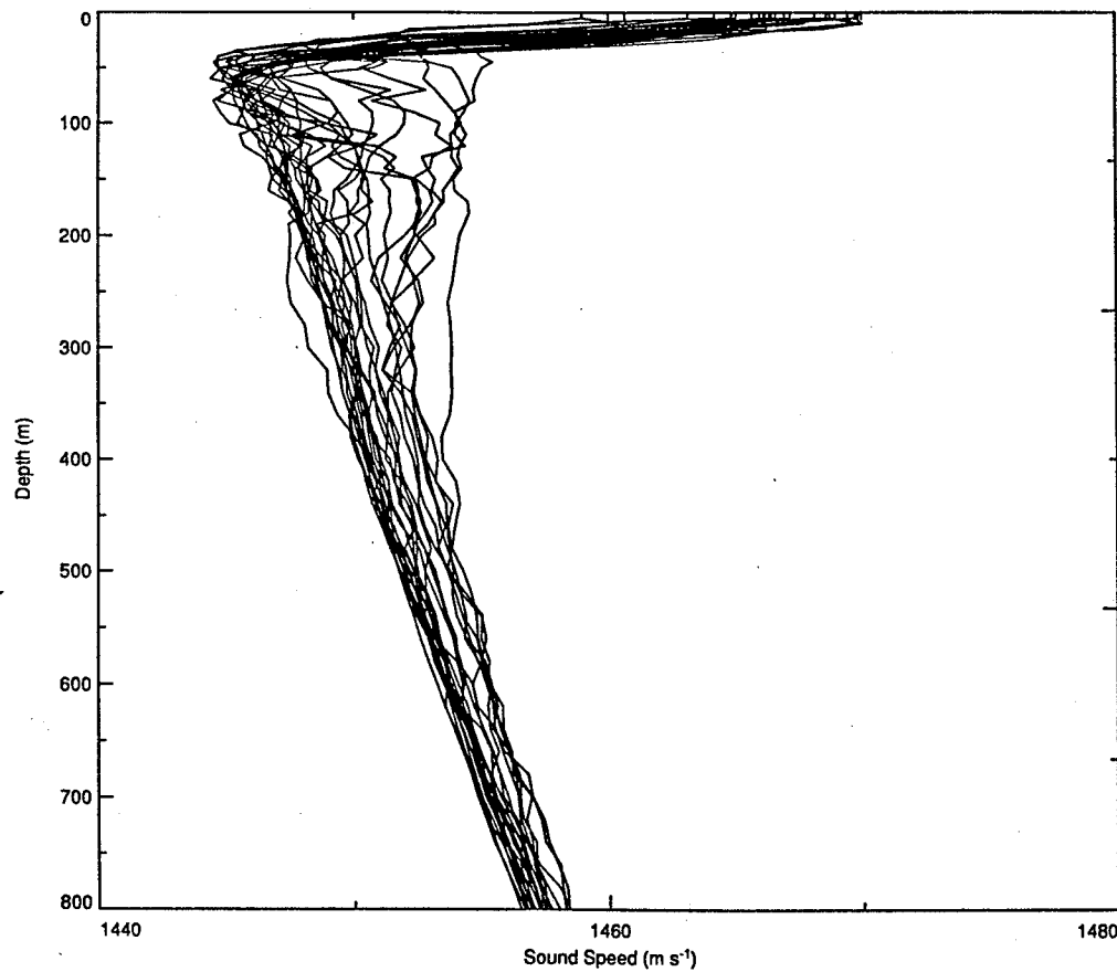
Figure 4.19. XSV sound speed profiles from 1989.
