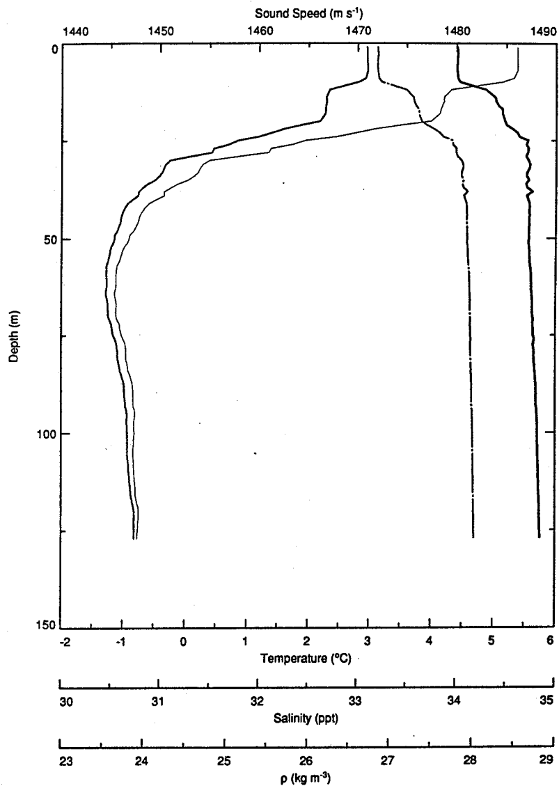
1989 MST : CTD Cast 044
