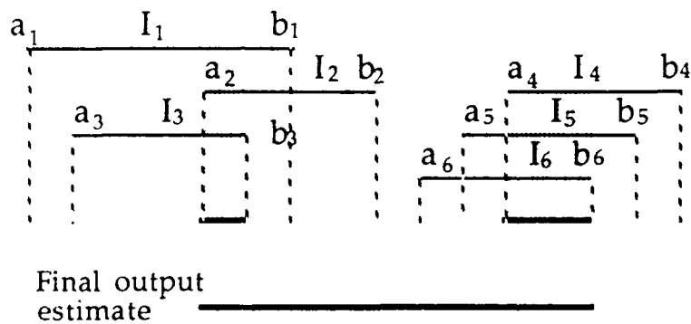
Figure 1. Integration Interval estimates (a_1 < a_3 < a_2 < b_3 < b_1 < b_2 < a_6 < a_5 < a_4 < b_6 < b_5 < b_4)
