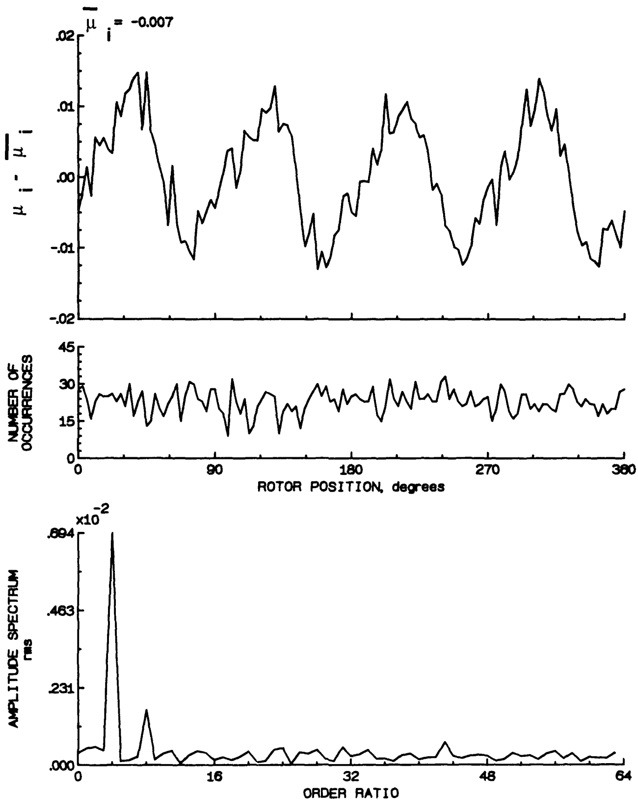
Figure 131.- Induced inflow velocity measured at 240 degrees and r/R of 0.40.
