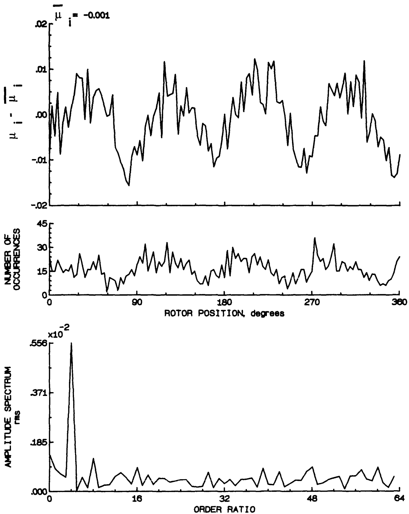
Figure 189.- Induced inflow velocity measured at 330 degrees and r/R of 1.10.
