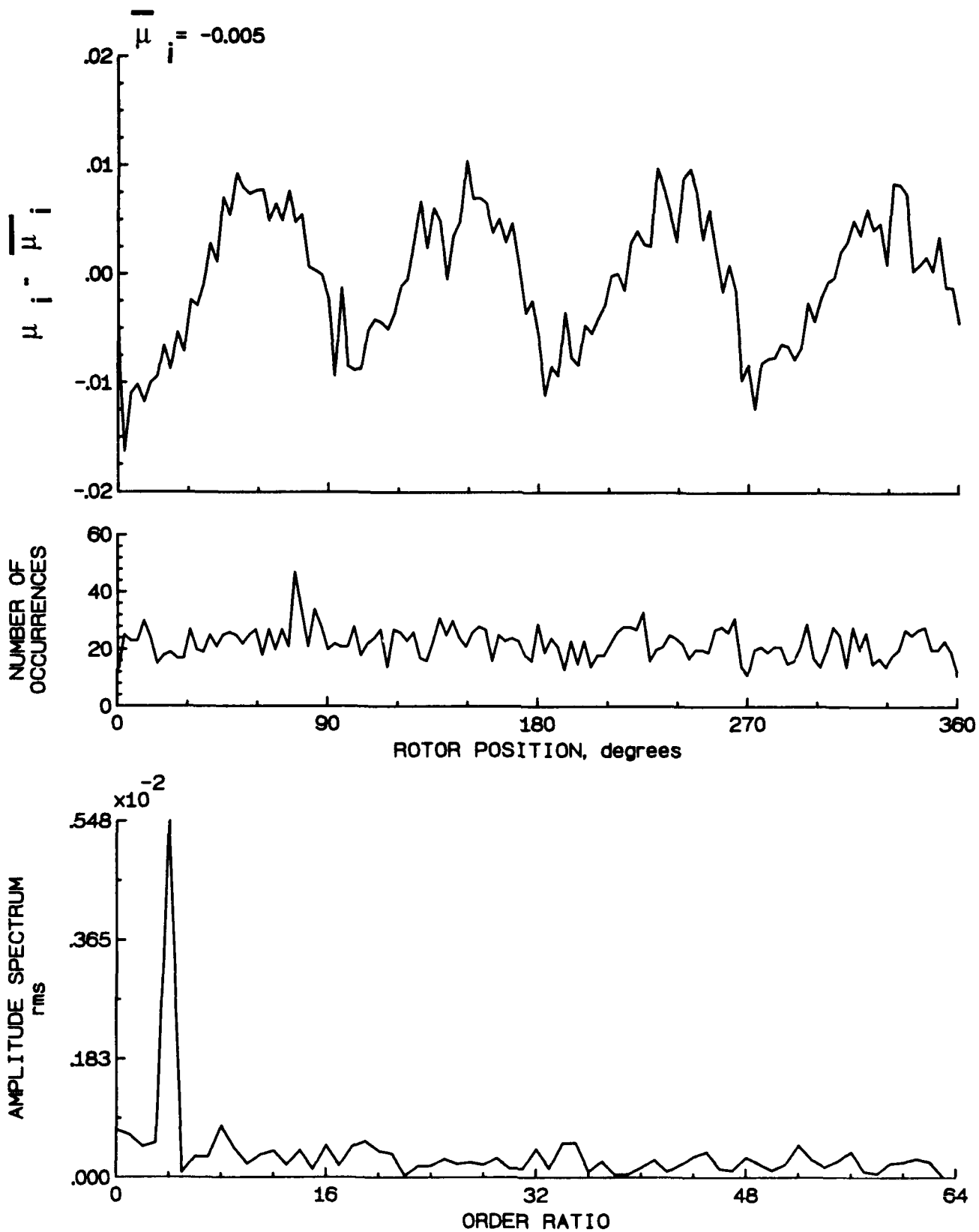
Figure 149.- Induced inflow velocity measured at 270 degrees and r/R of 0.70.
