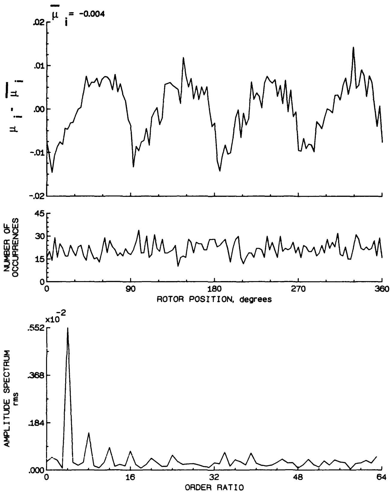
Figure 151.- Induced inflow velocity measured at 270 degrees and r/R of 0.78.
