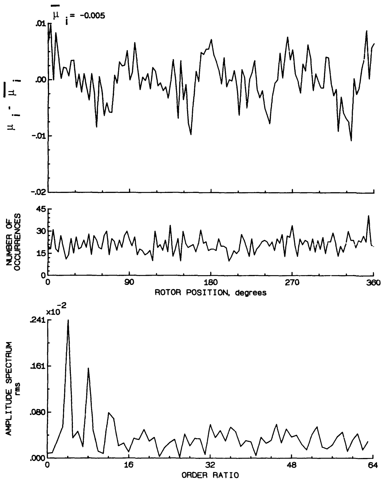
Figure 139.- Induced inflow velocity measured at 240 degrees and r/R of 0.90.
