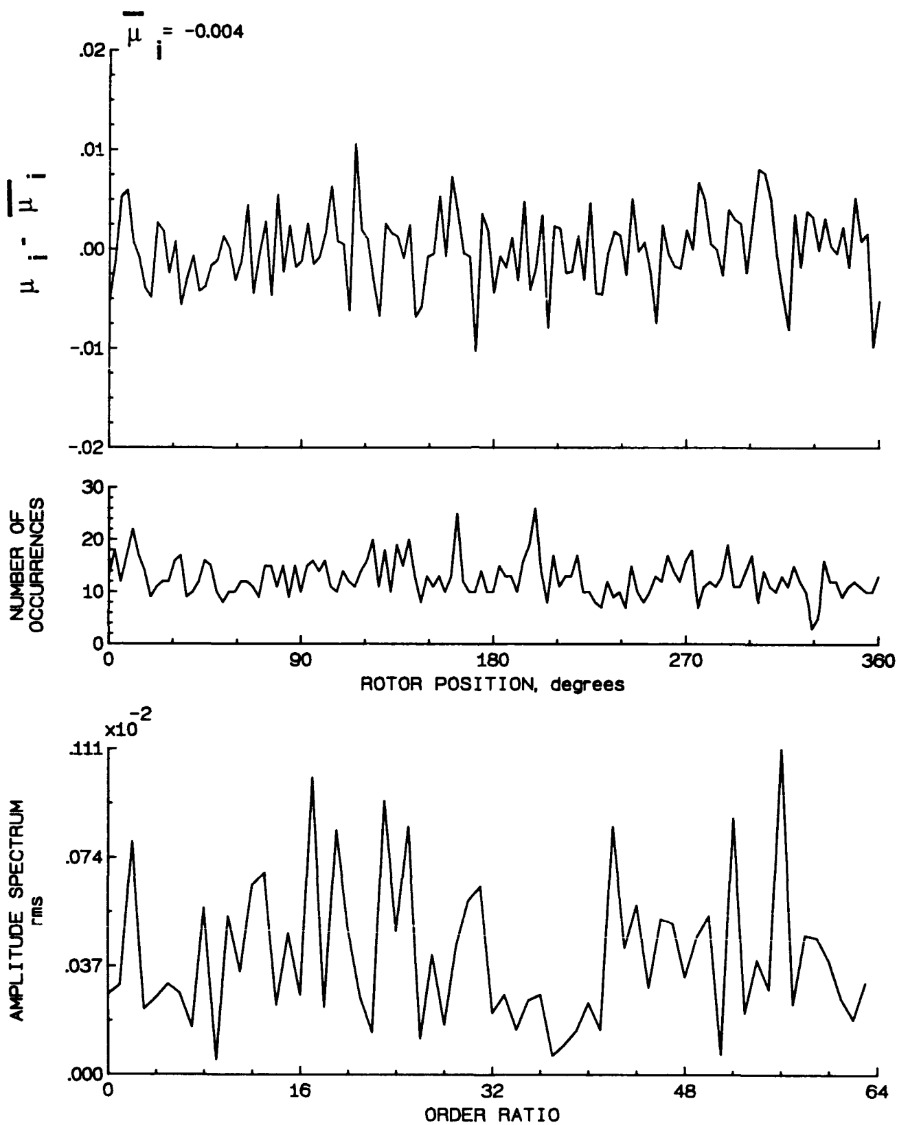
Figure 56.- Induced inflow velocity measured at 60 degrees and r/R of 1.10.
