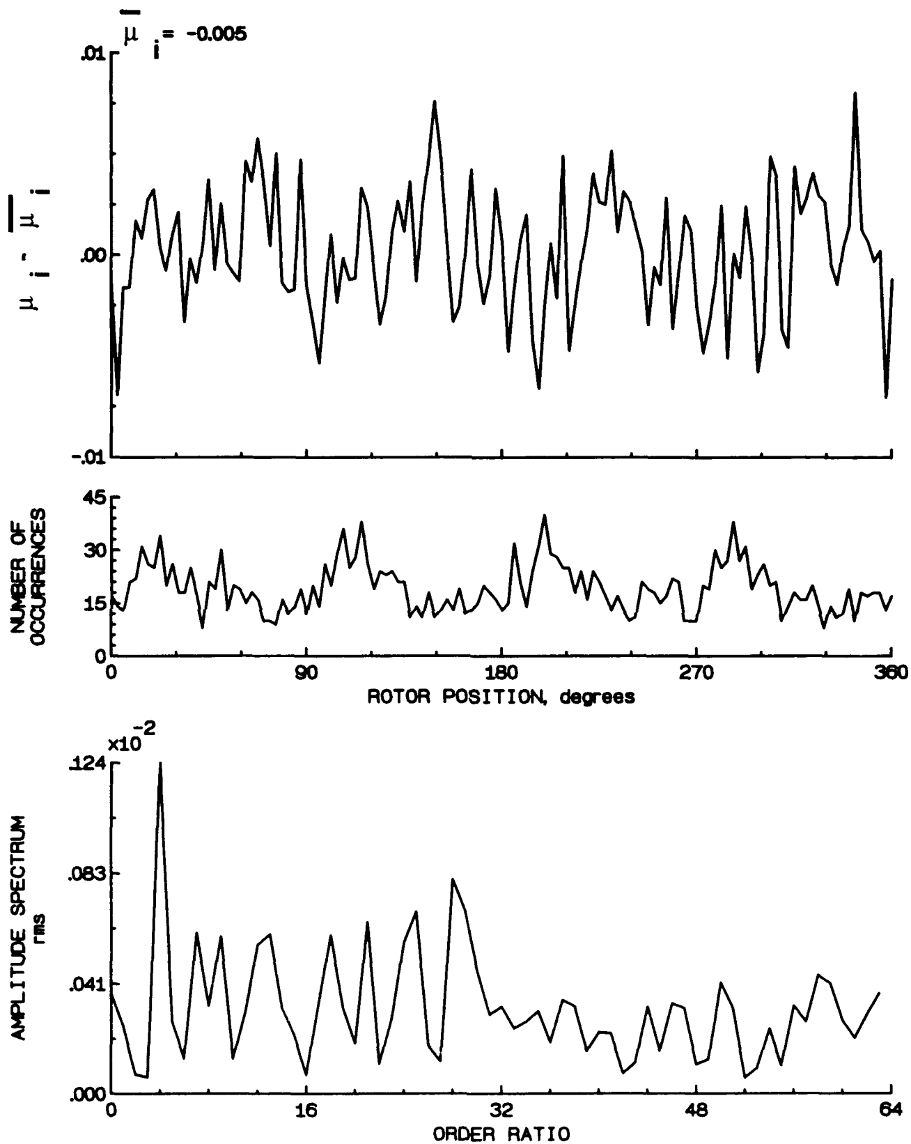
Figure 157.- Induced inflow velocity measured at 270 degrees and r/R of 1.02.
