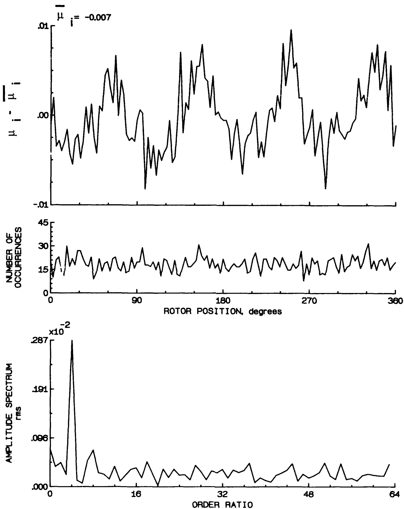
Figure 89.- Induced inflow velocity measured at 150 degrees and r/R of 0.50.
