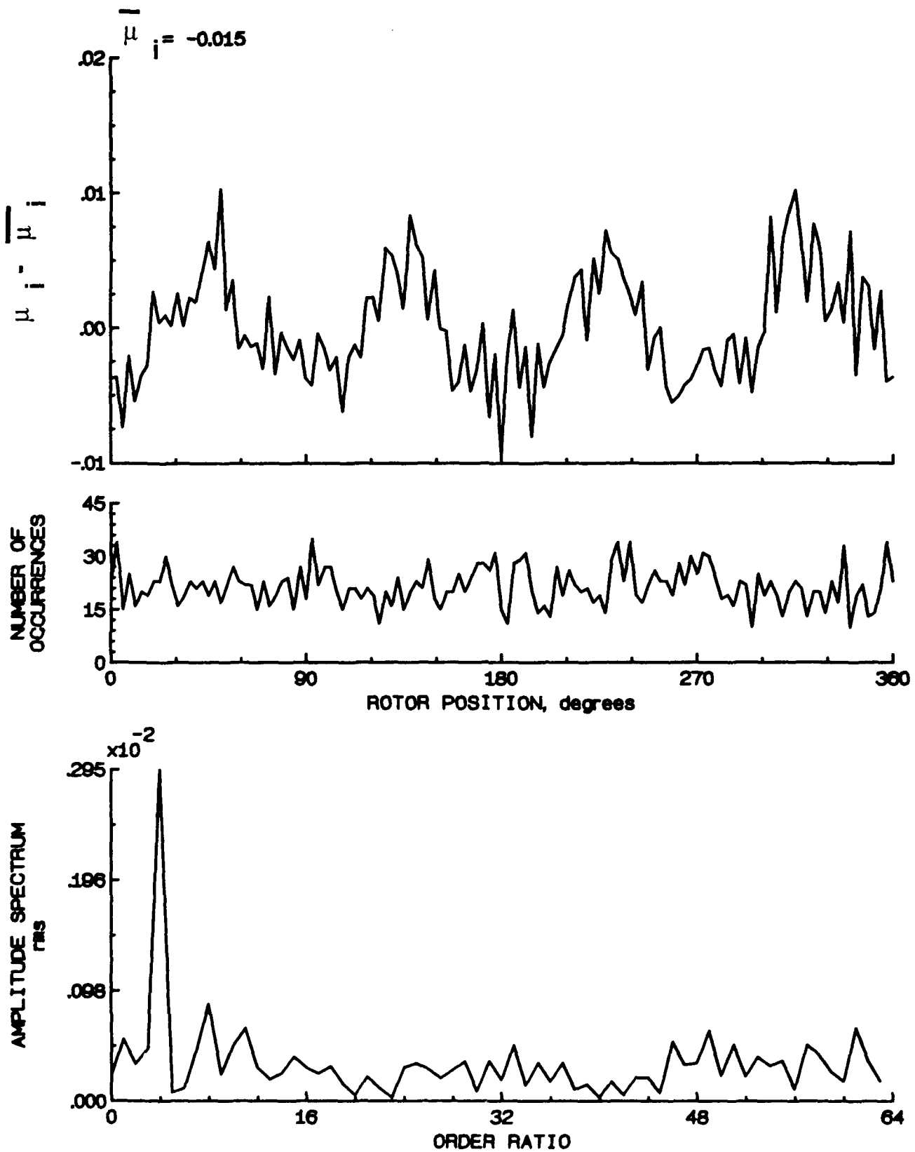
Figure 106.- Induced inflow velocity measured at 180 degrees and r/R of 0.70.
