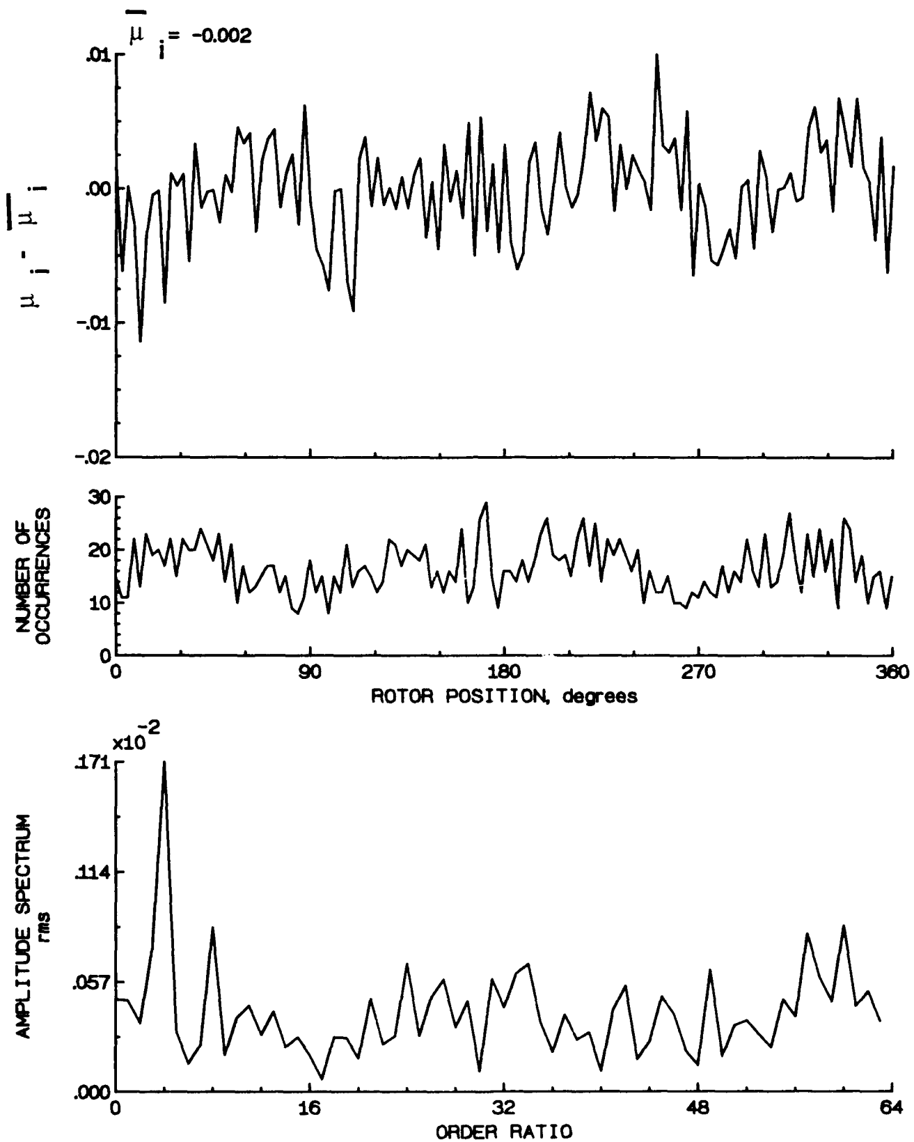
Figure 21.- Induced inflow velocity measured at 0 degrees and r/R of 0.90.
