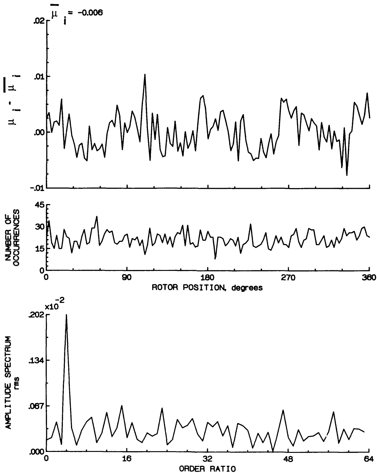
Figure 140.- Induced inflow velocity measured at 240 degrees and r/R of 0.94.
