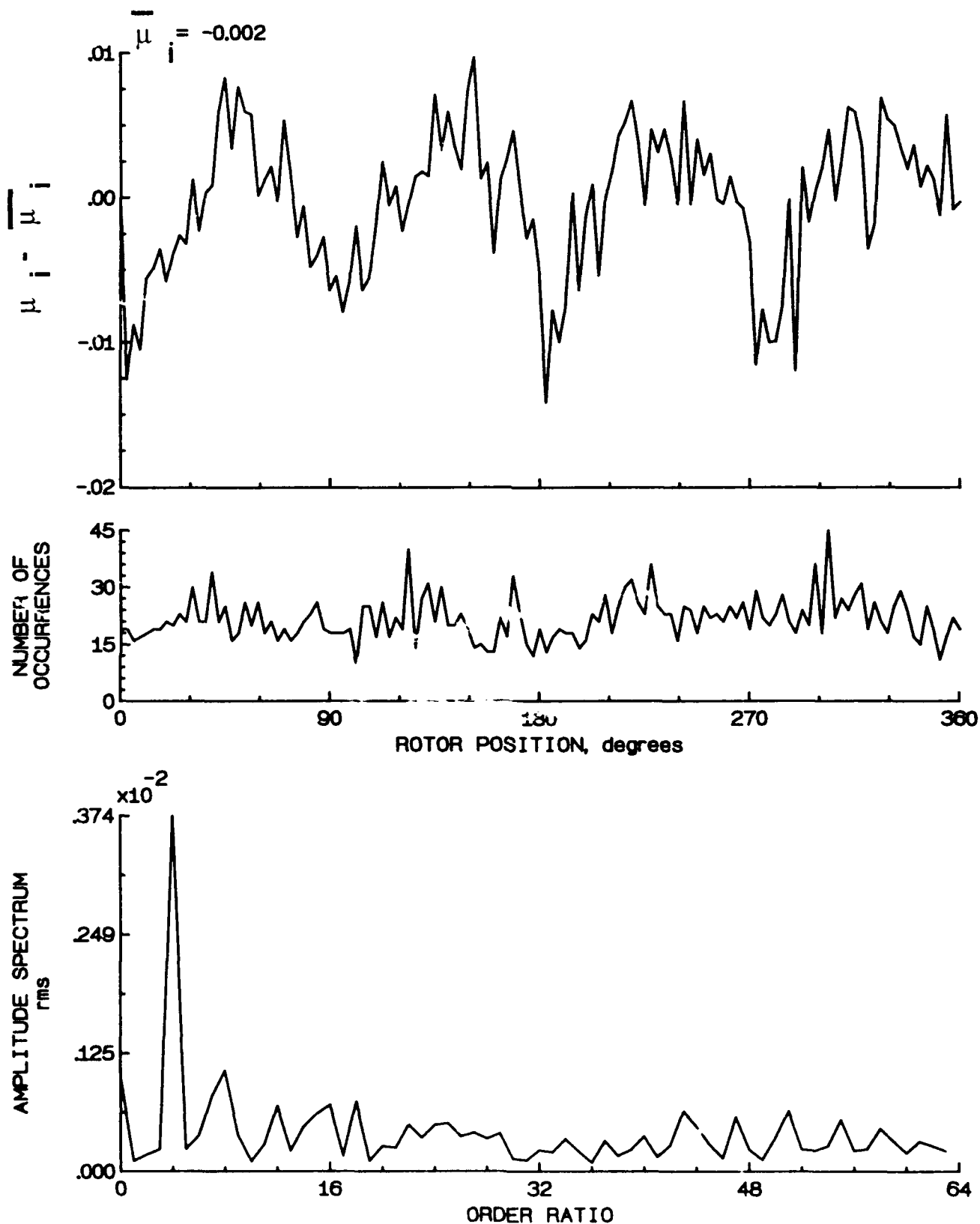
Figure 154.- Induced inflow velocity measured at 270 degrees and r/R of 0.90.
