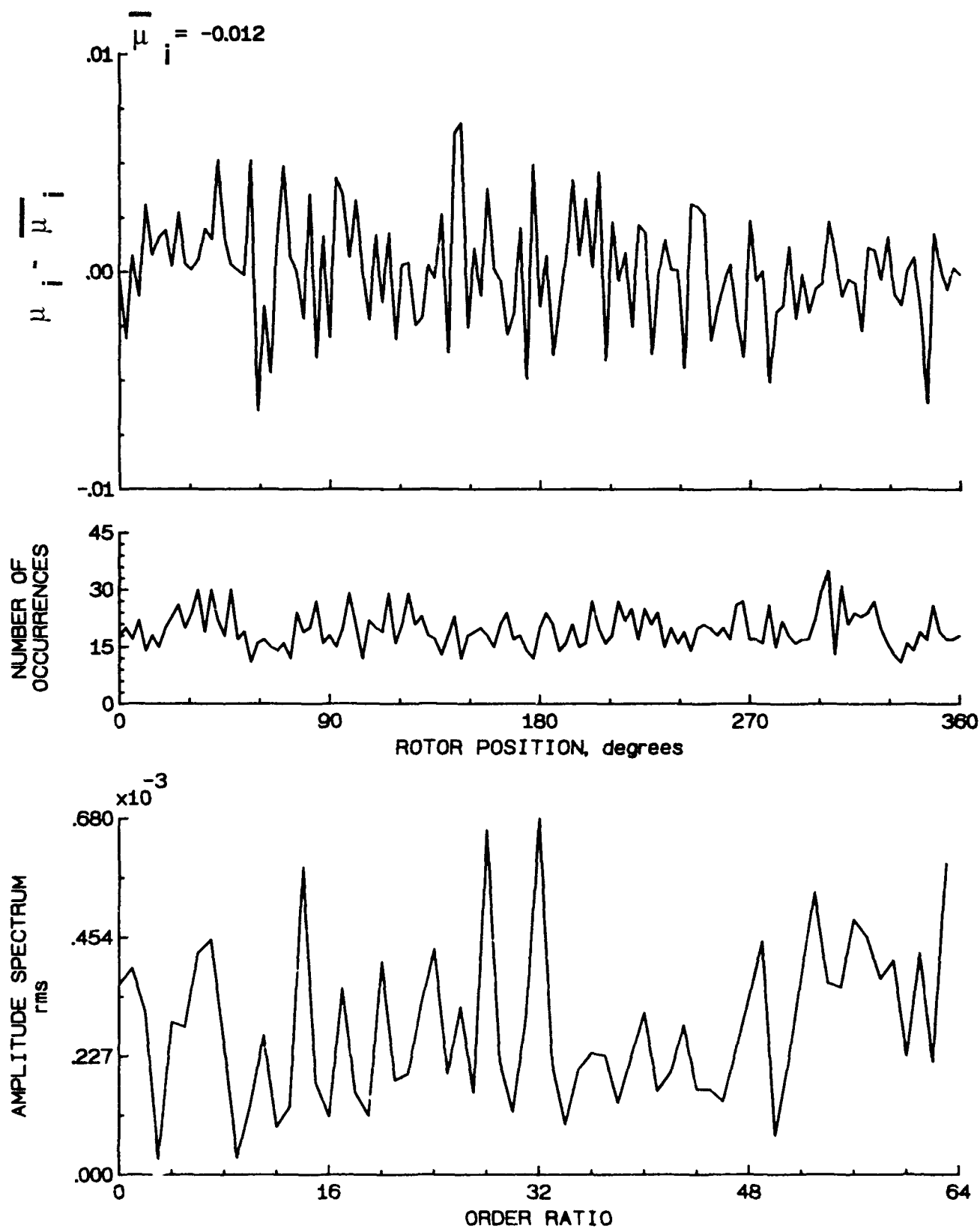
Figure 85.- Induced inflow velocity measured at 120 degrees and r/R of 1.04.
