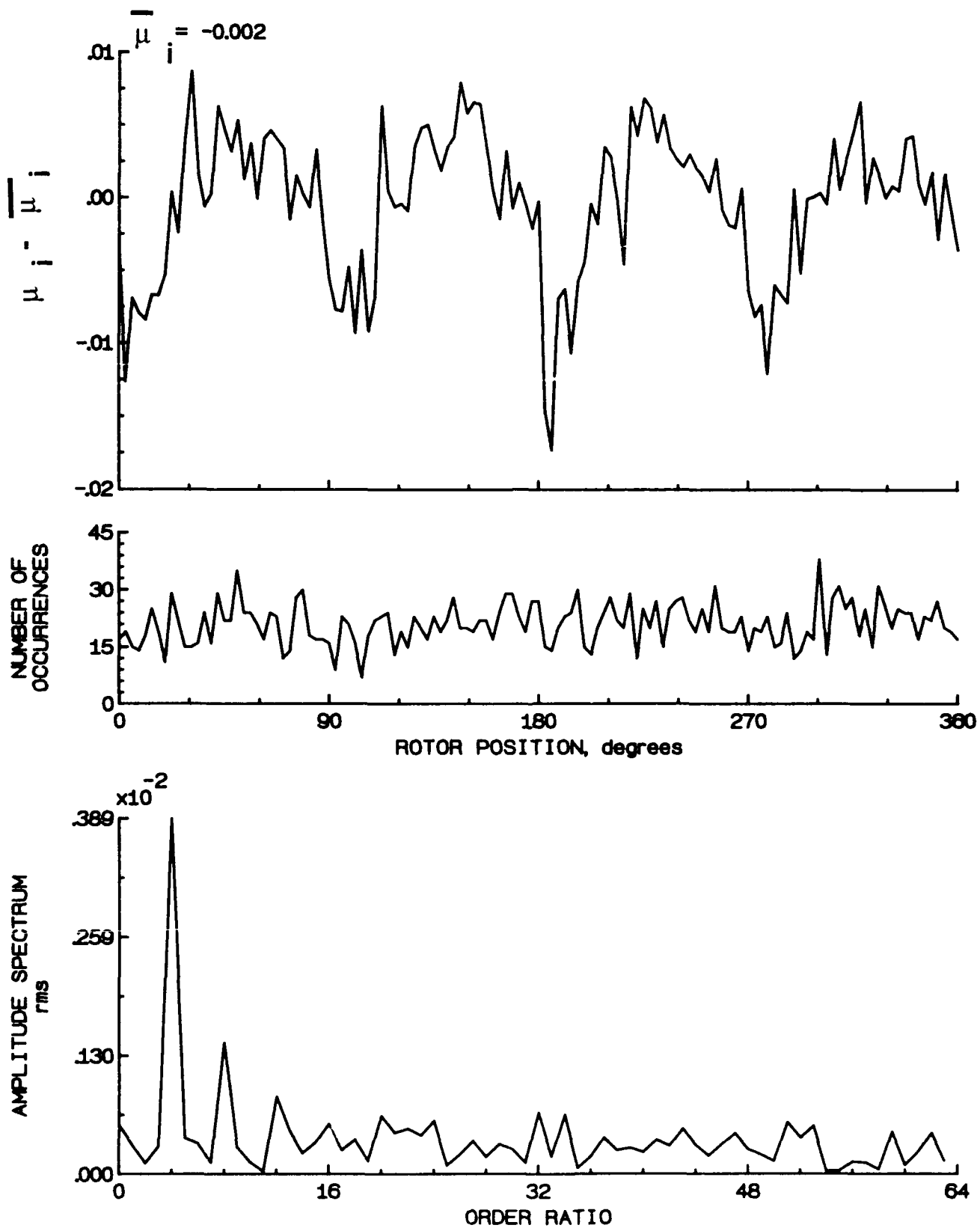
Figure 153.- Induced inflow velocity measured at 270 degrees and r/R of 0.86.
