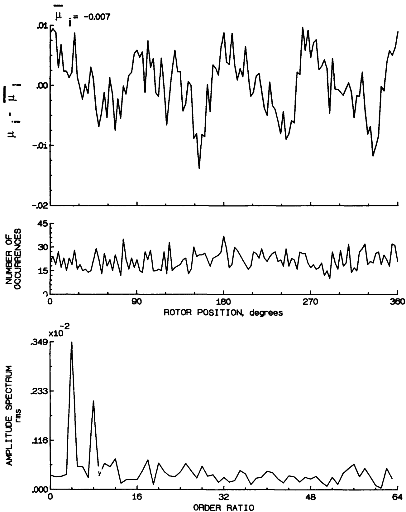
Figure 138.- Induced inflow velocity measured at 240 degrees and r/R of 0.86.
