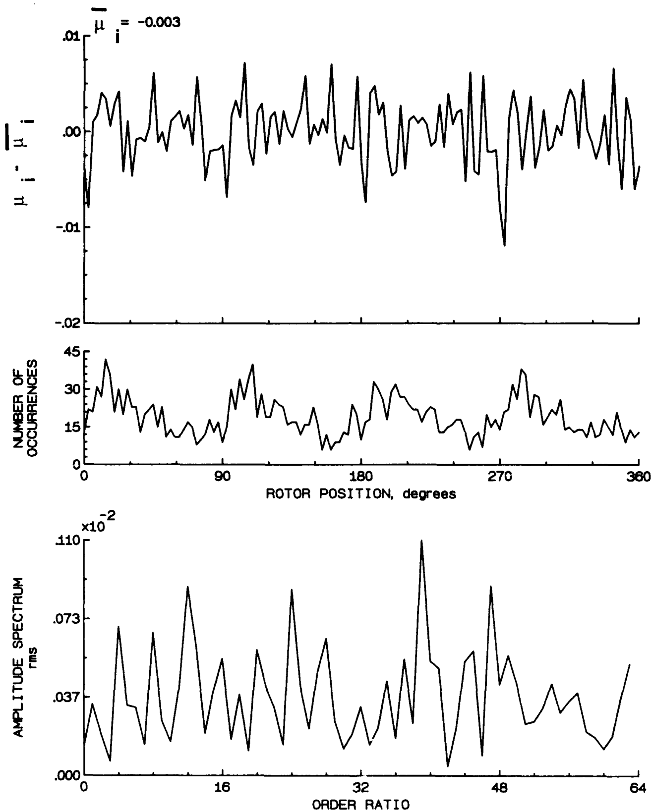
Figure 158.- Induced inflow velocity measured at 270 degrees and r/R of 1.04.
