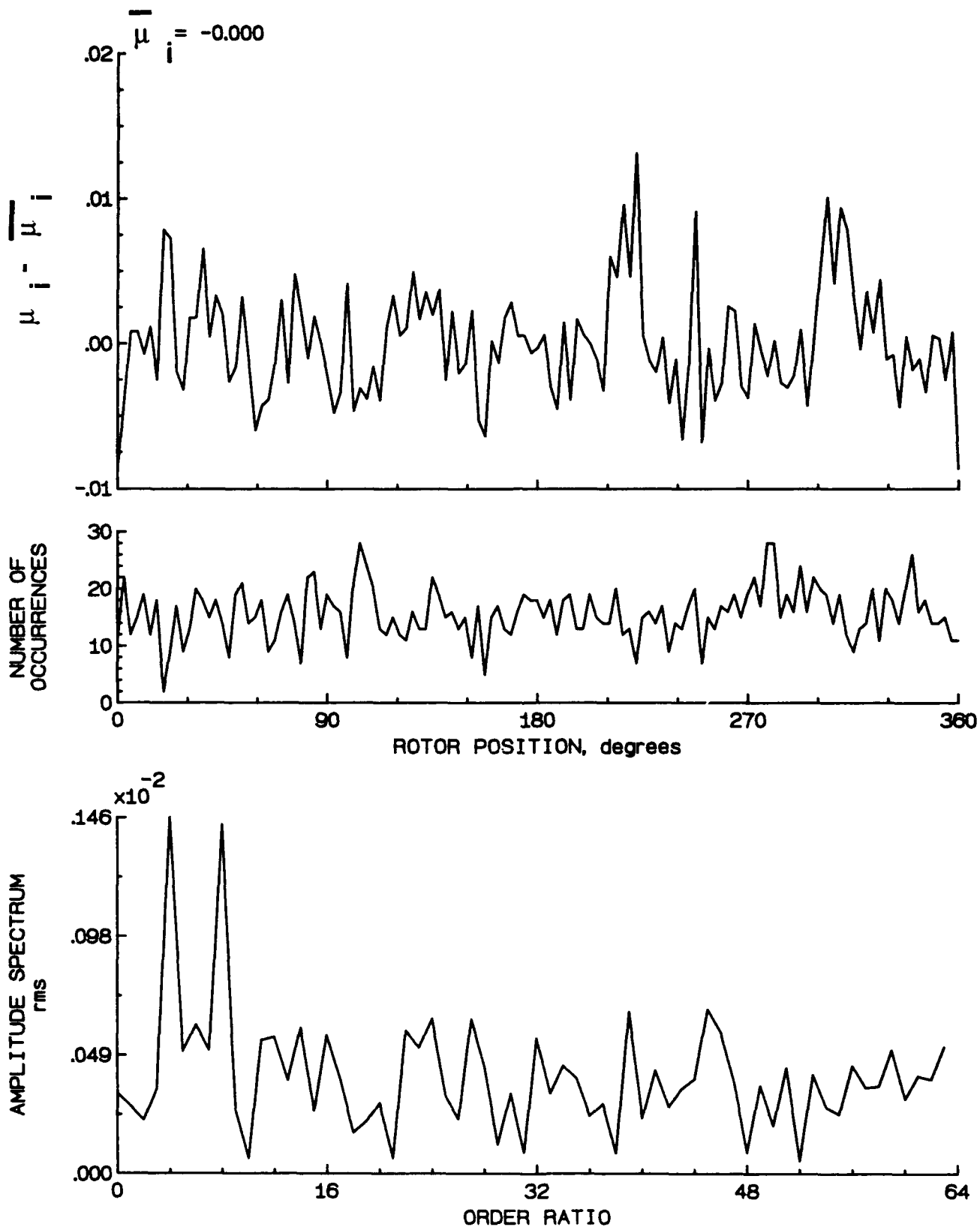
Figure 76.- Induced inflow velocity measured at 120 degrees and r/R of 0.70.
