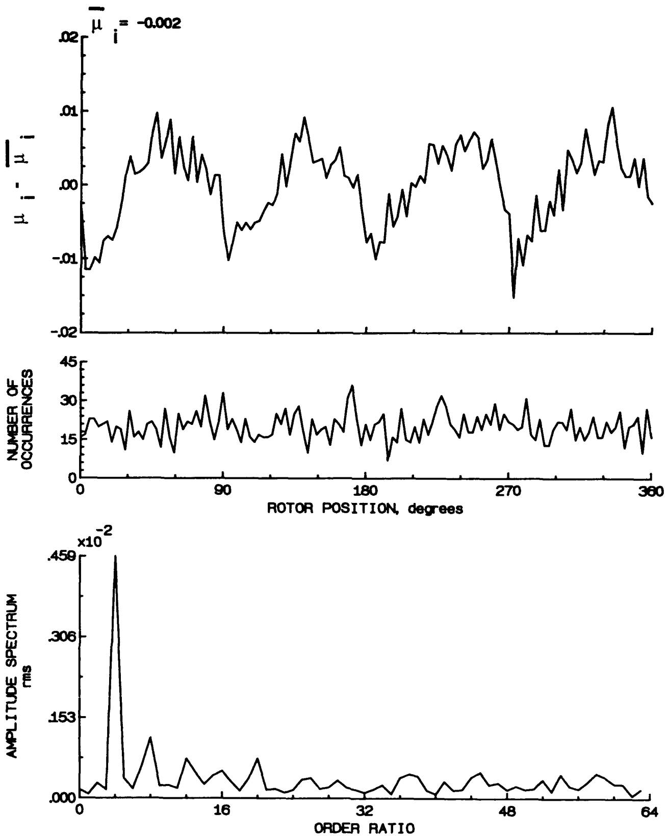
Figure 152.- Induced inflow velocity measured at 270 degrees and r/R of 0.82.
