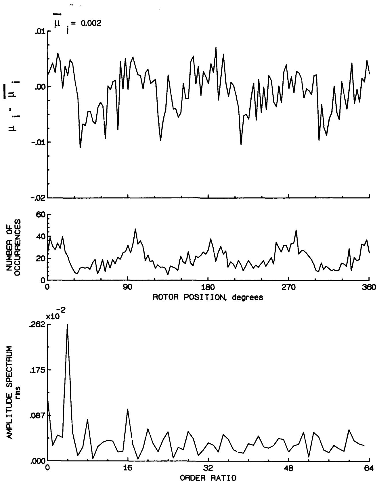
Figure 168.- Induced inflow velocity measured at 300 degrees and r/R of 0.86.
