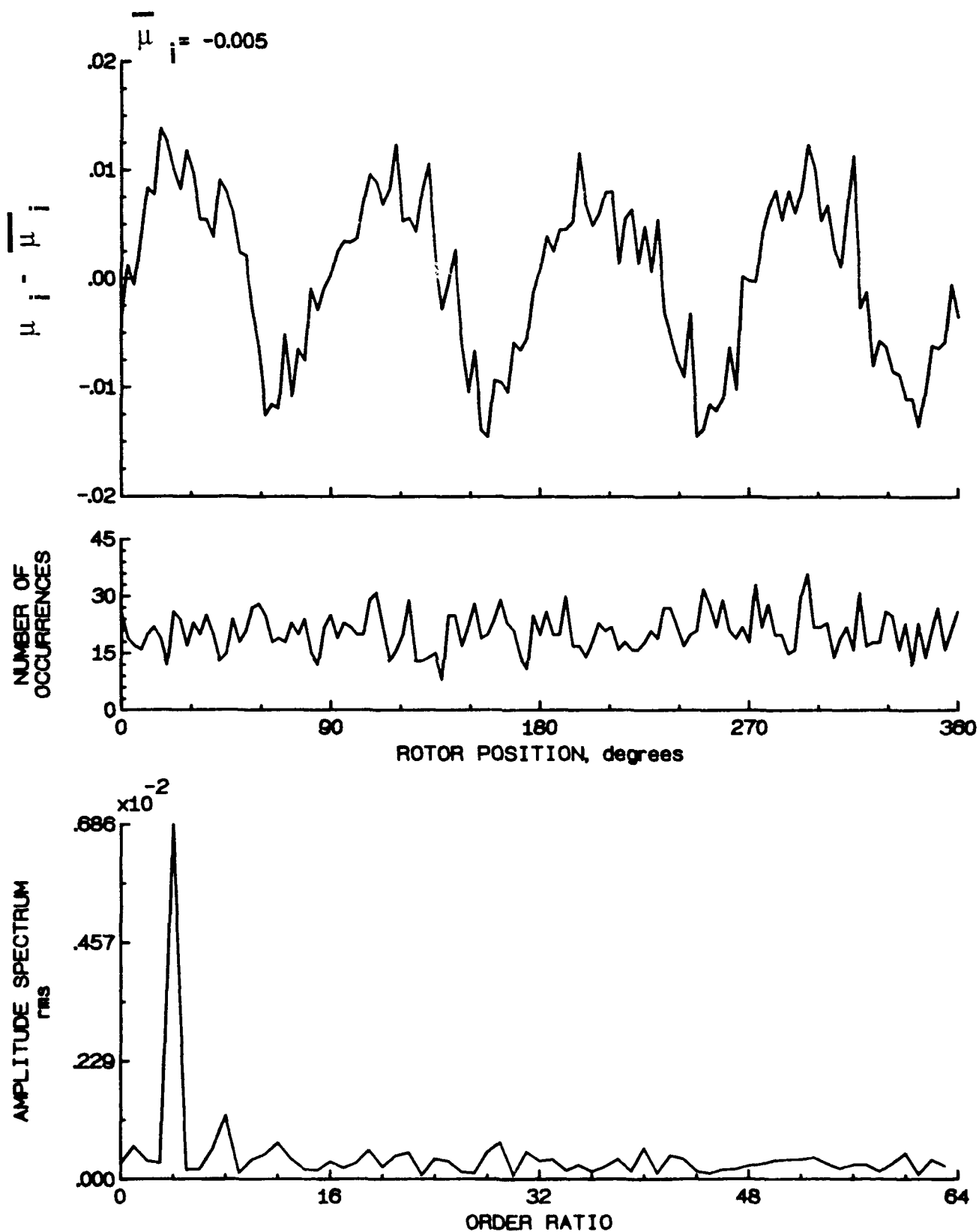
Figure 133.- Induced inflow velocity measured at 240 degrees and r/R of 0.60.
