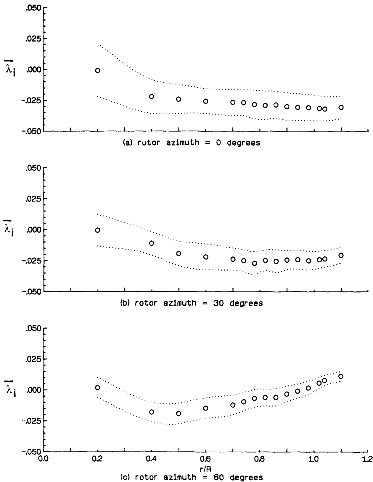
Figure 9. Radial distribution of mean induced inflow ratio - \bar{\lambda}_i .
