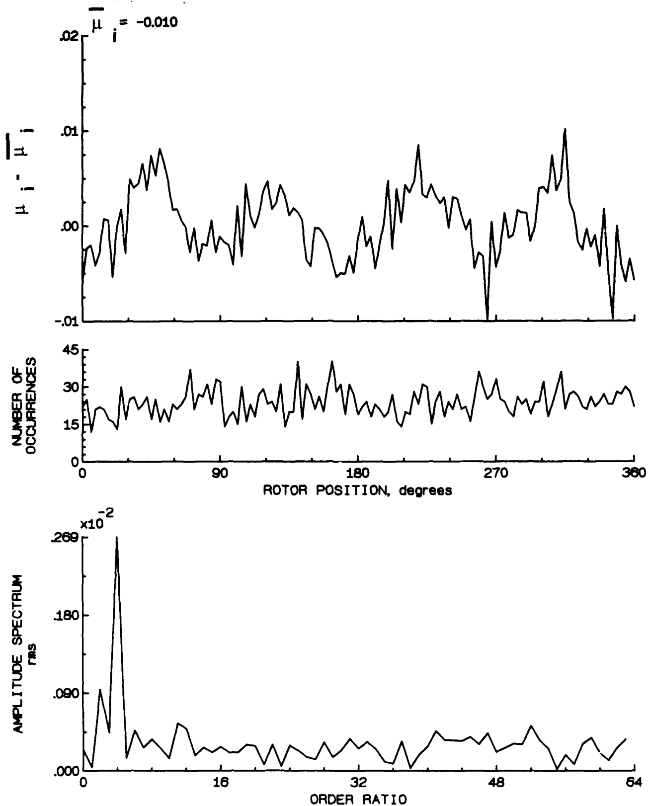
Figure 130.- Induced inflow velocity measured at 240 degrees and r/R of 0.20.
