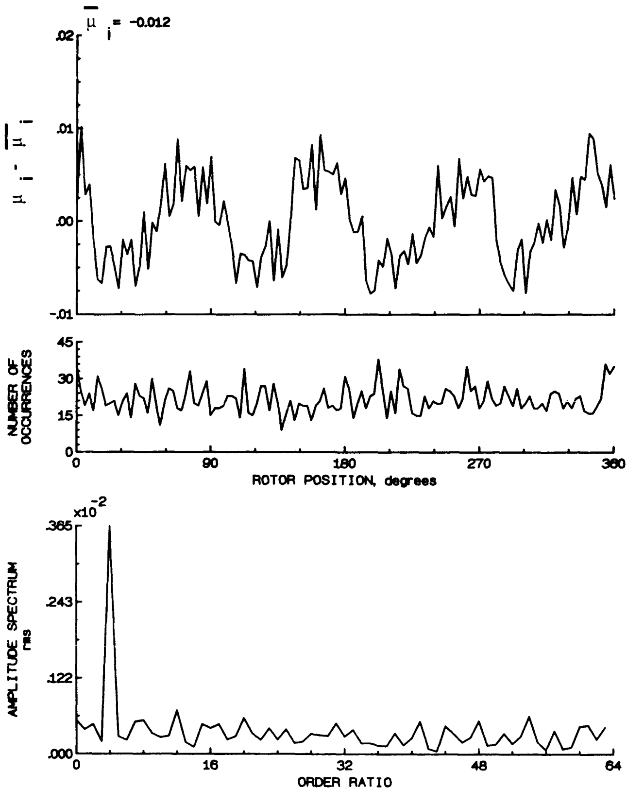
Figure 104.- Induced inflow velocity measured at 180 degrees and r/R of 0.50.
