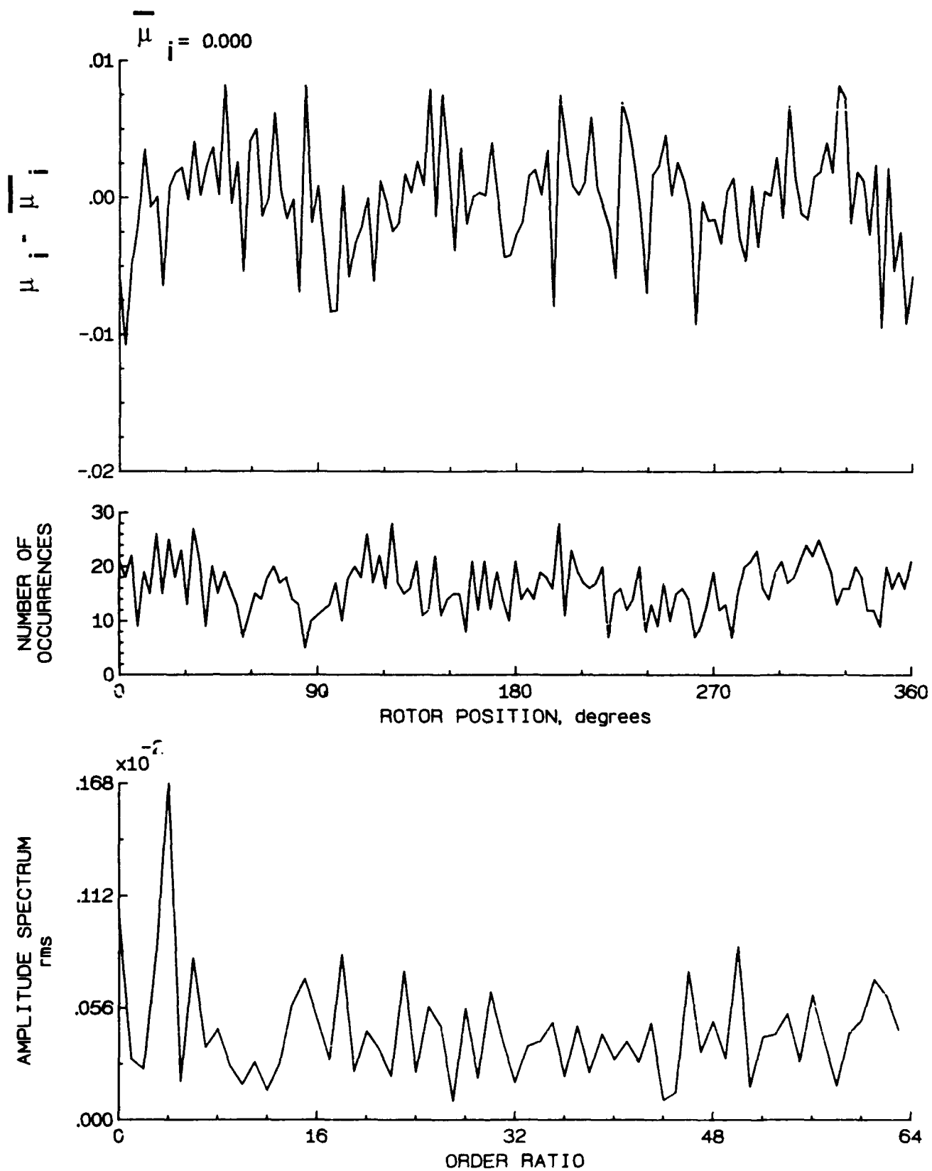
Figure 19.- Induced inflow velocity measured at 0 degrees and r/R of 0.82.
