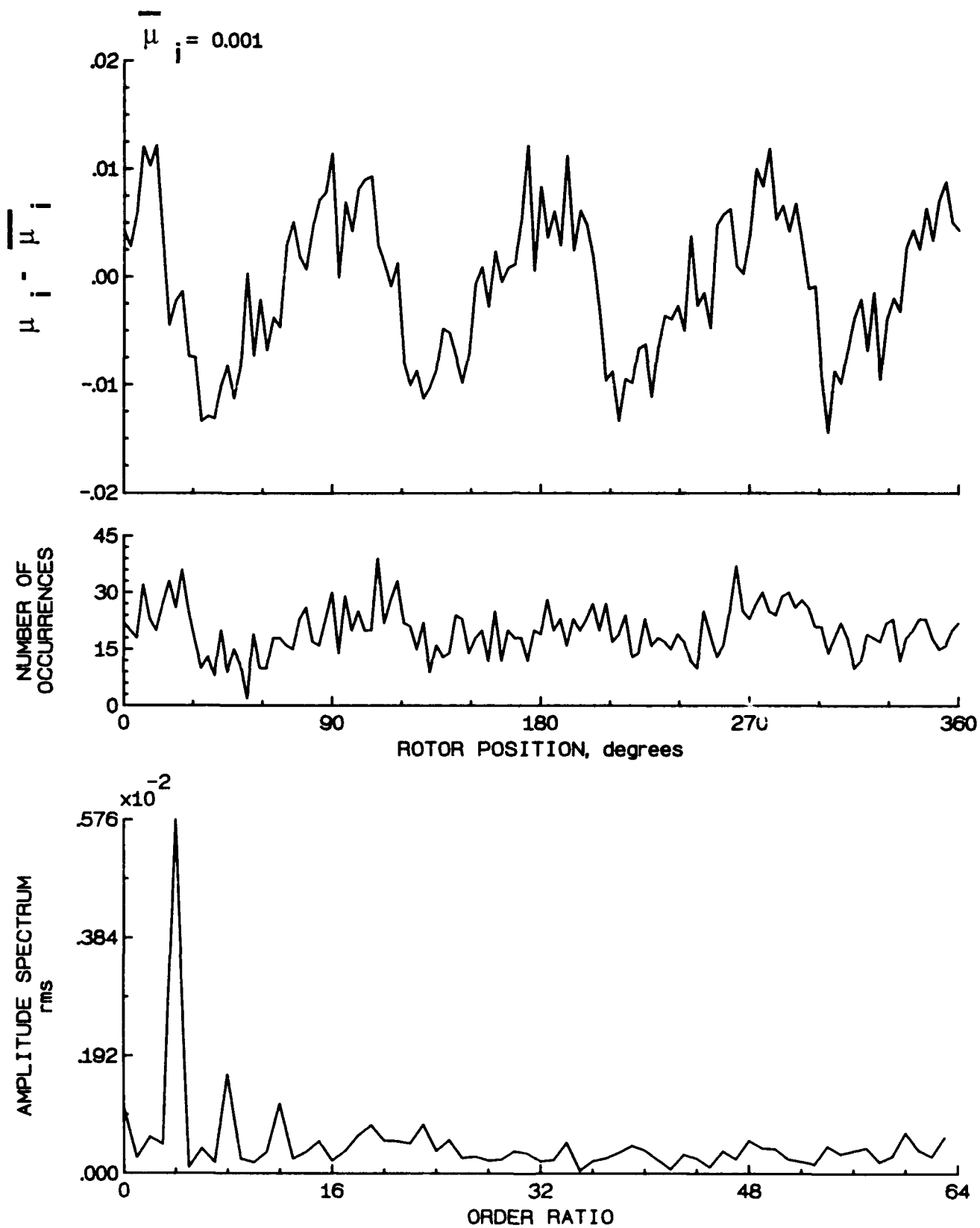
Figure 162.- Induced inflow velocity measured at 300 degrees and r/R of 0.50.
