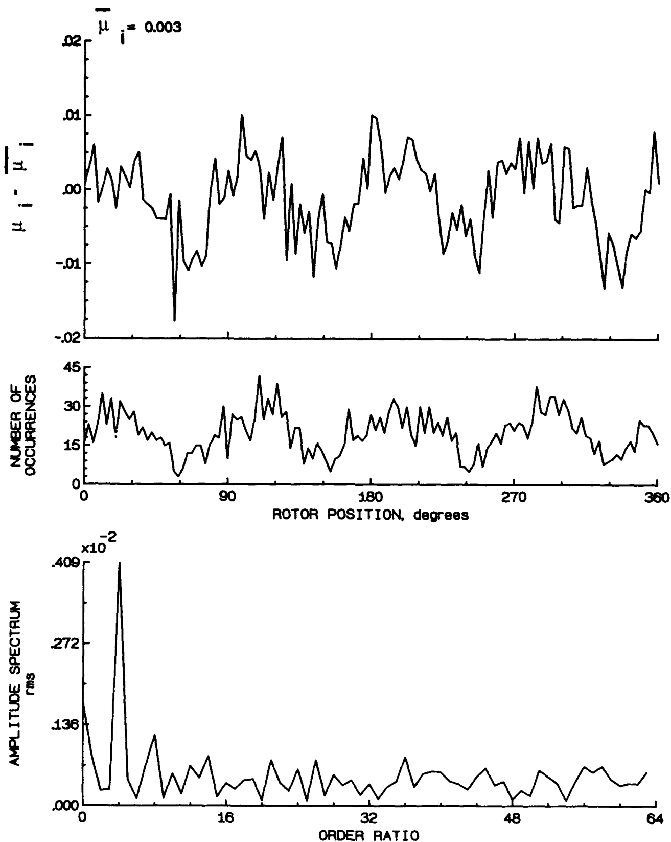
Figure 185.- Induced inflow velocity measured at 330 degrees and r/R of 0.94.
