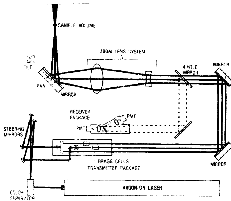
Figure 3. Schematic of Laser Velocimeter optics subsystem.
