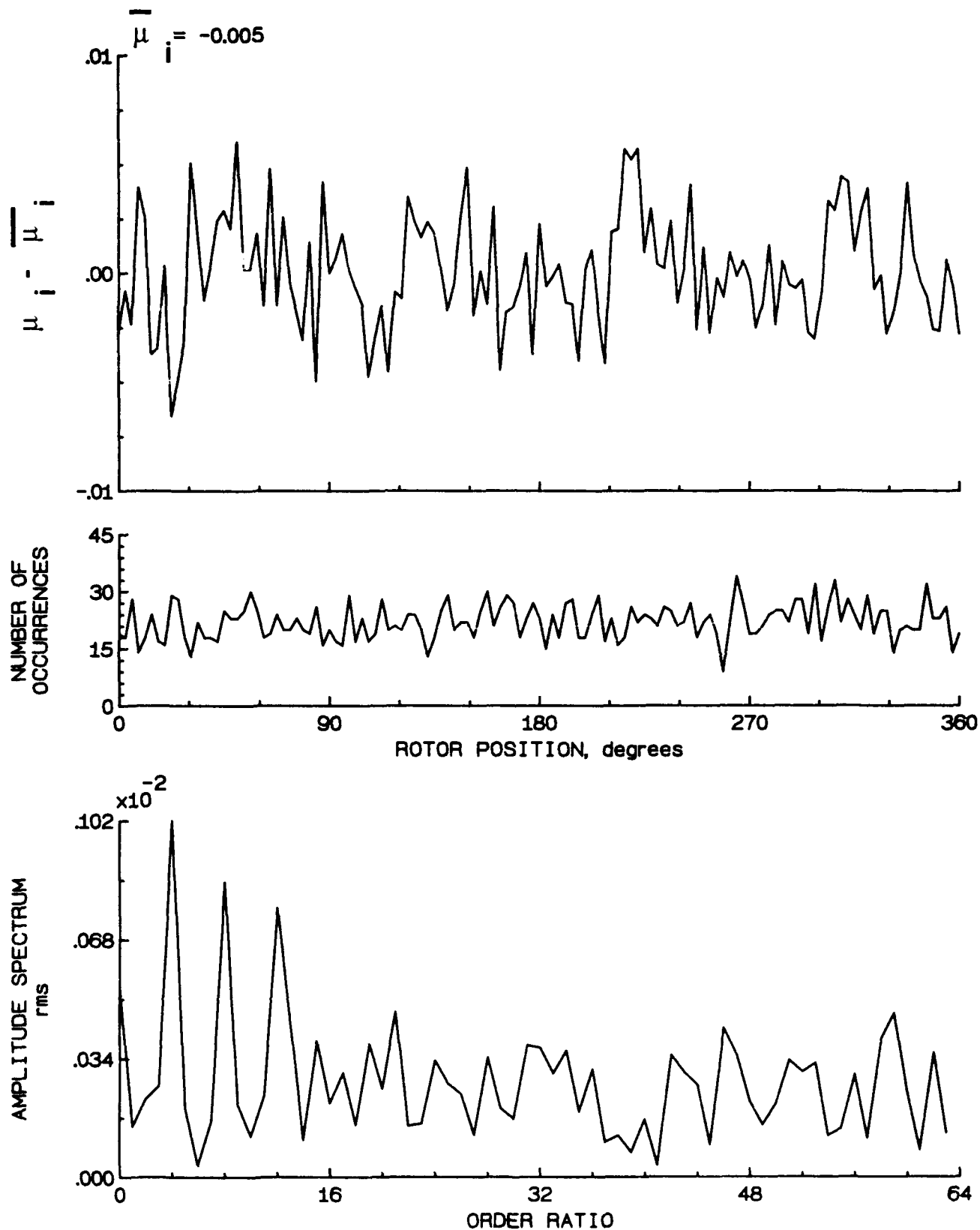
Figure 79.- Induced inflow velocity measured at 120 degrees and r/R of 0.82.
