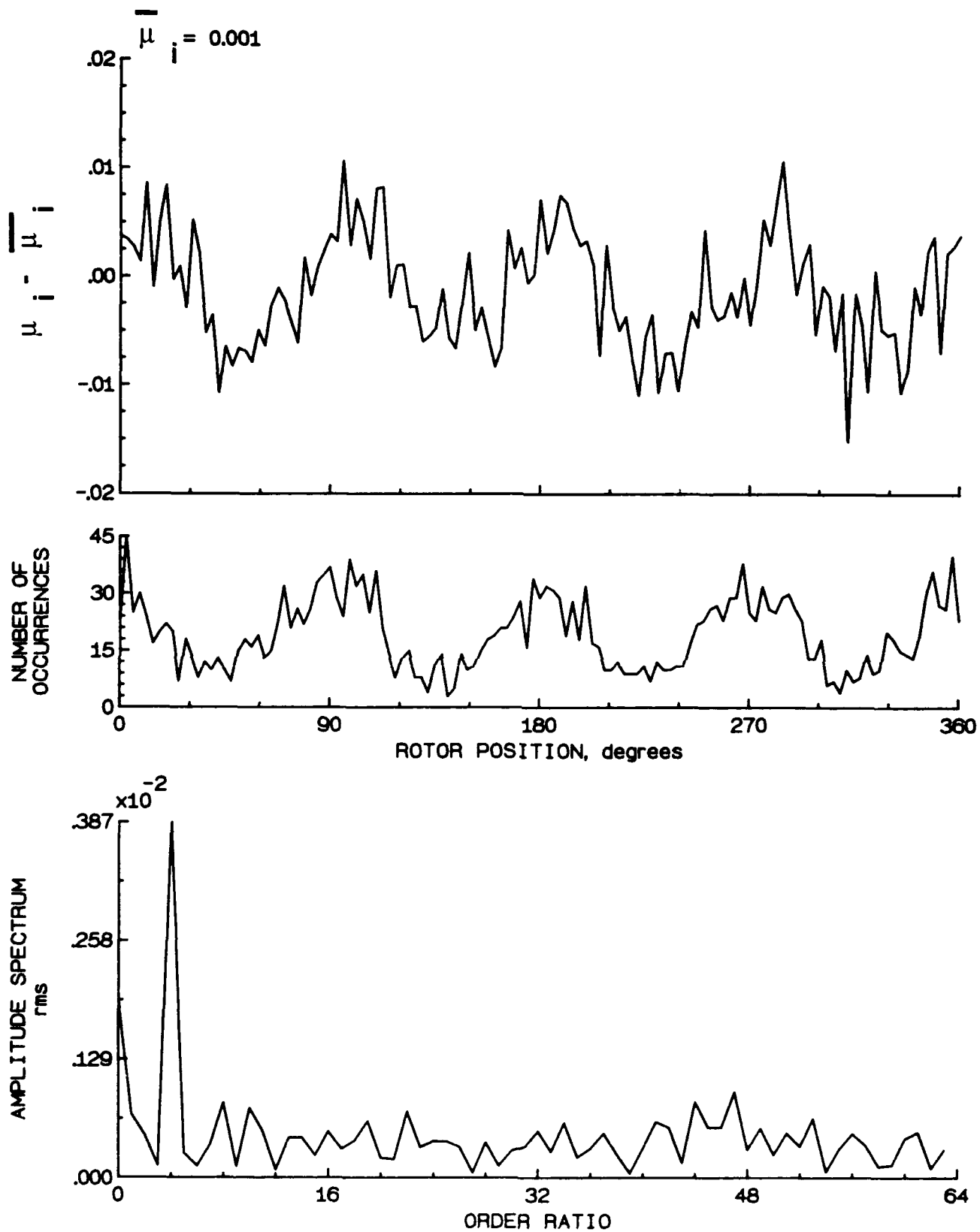
Figure 163.- Induced inflow velocity measured at 300 degrees and r/R of 0.60.
