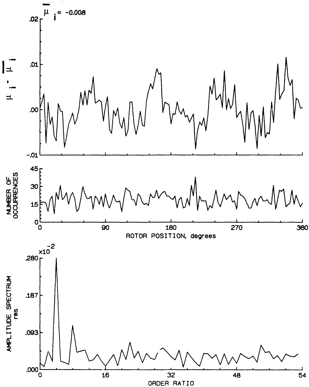
Figure 120.- Induced inflow velocity measured at 210 degrees and r/R of 0.74.
