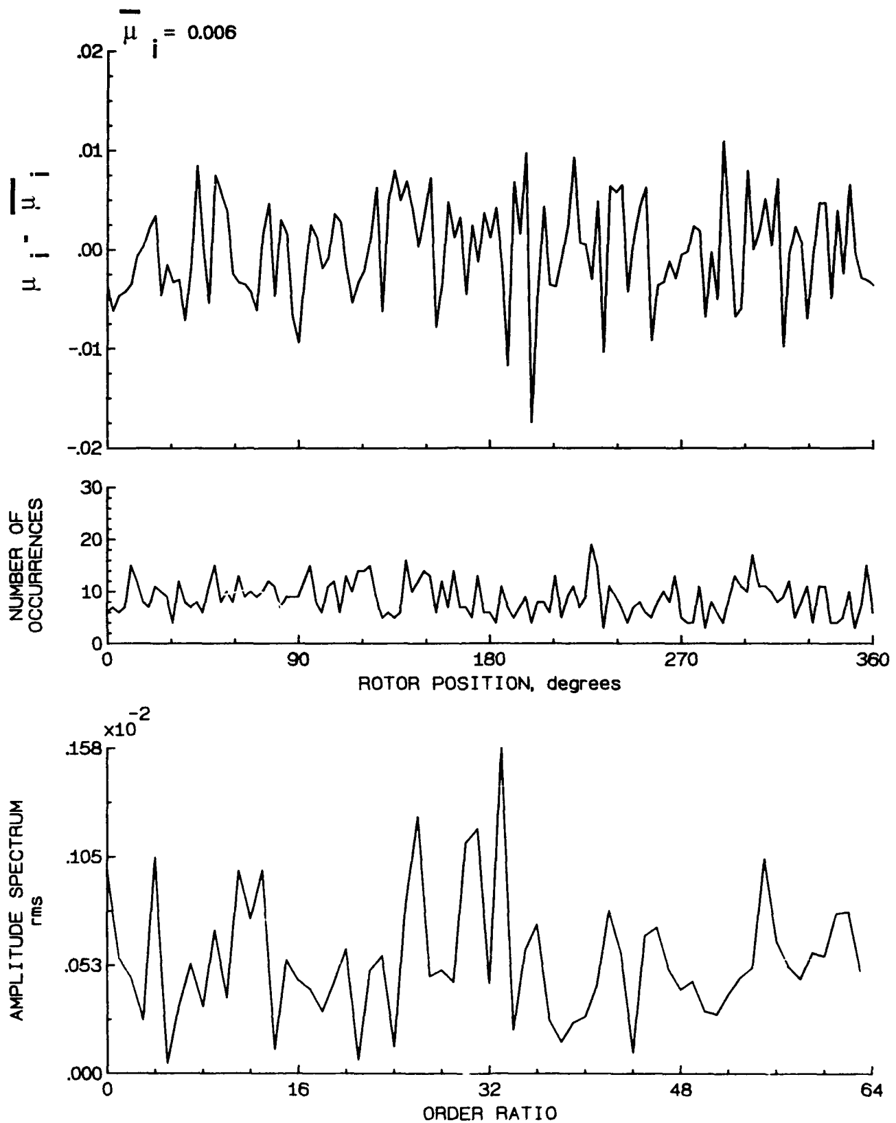
Figure 30.- Induced inflow velocity measured at 30 degrees and r/R of 0.60.
