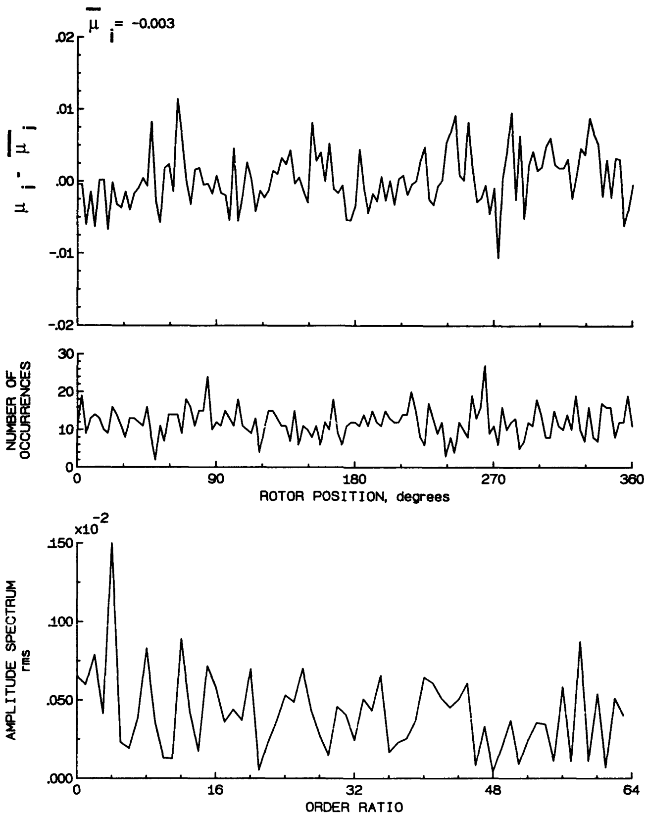
Figure 55.- Induced inflow velocity measured at 60 degrees and r/R of 1.04.
