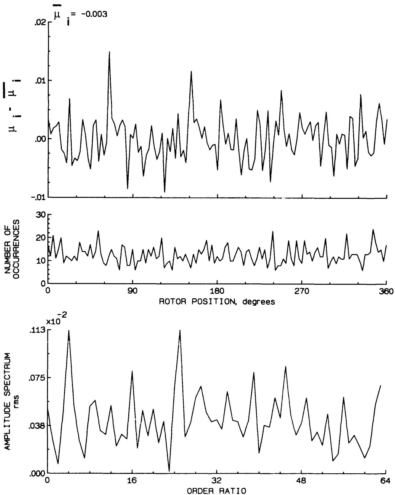
Figure 53.- Induced inflow velocity measured at 60 degrees and r/R of 0.98.
