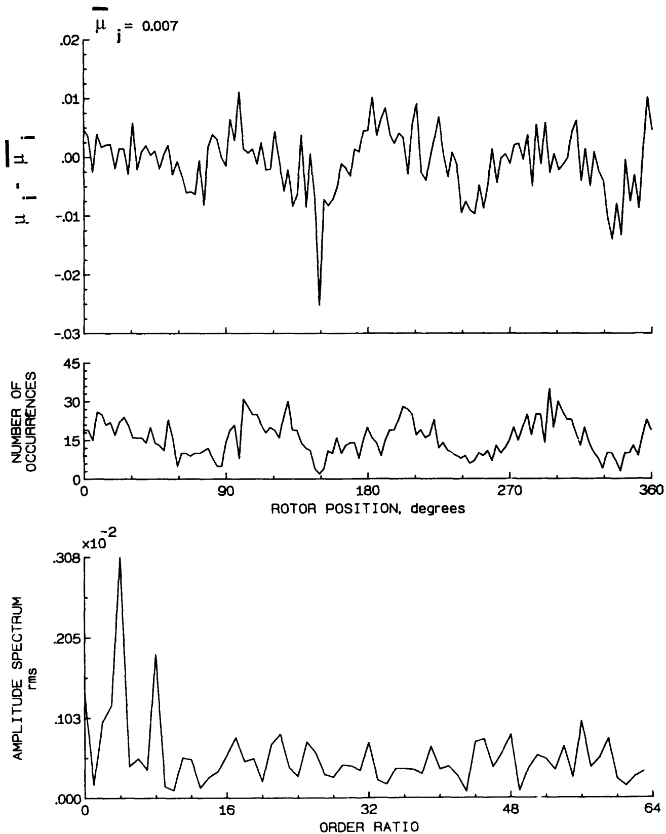
Figure 183.- Induced inflow velocity measured at 330 degrees and r/R of 0.86.
