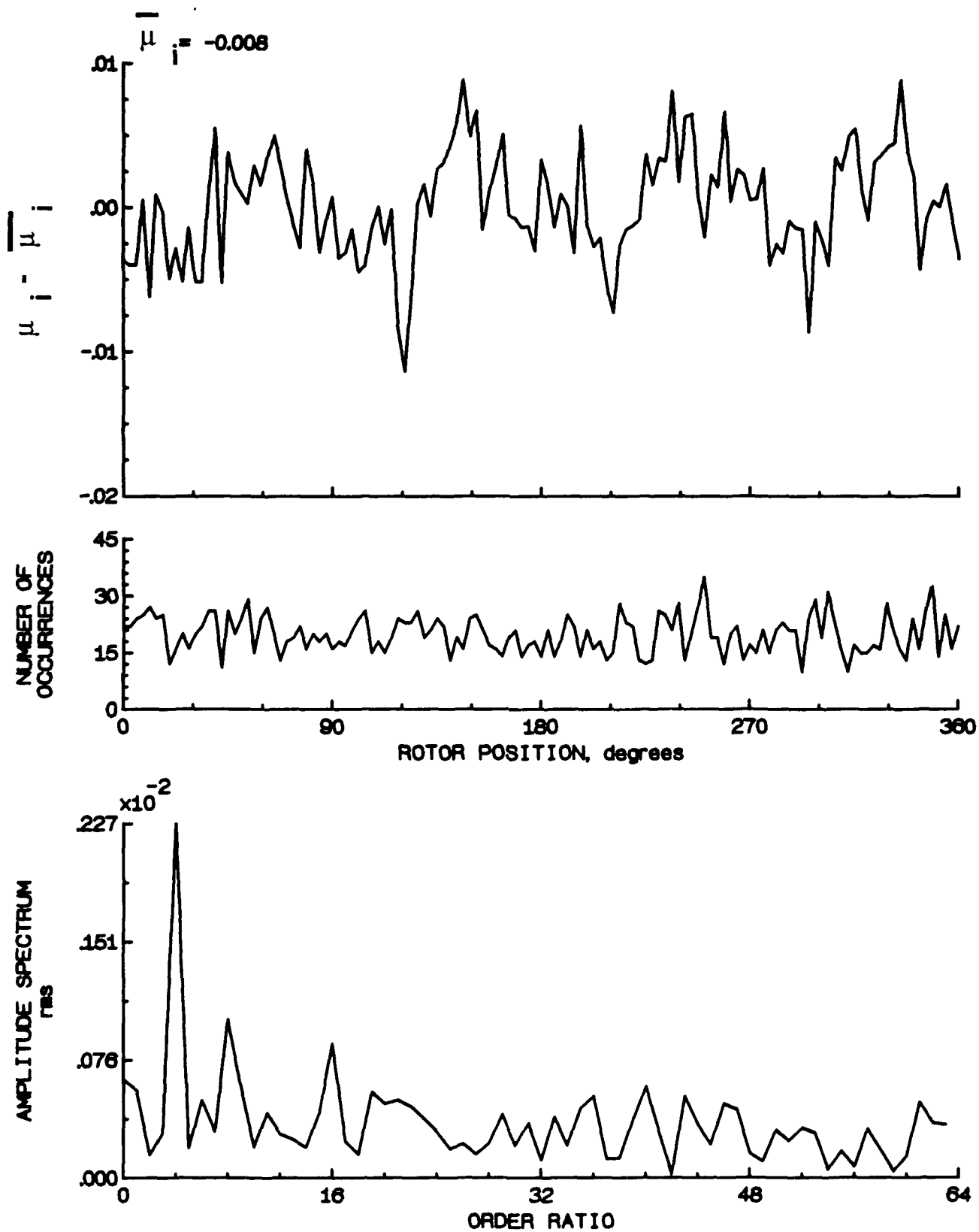
Figure 123.- Induced inflow velocity measured at 210 degrees and r/R of 0.86.
