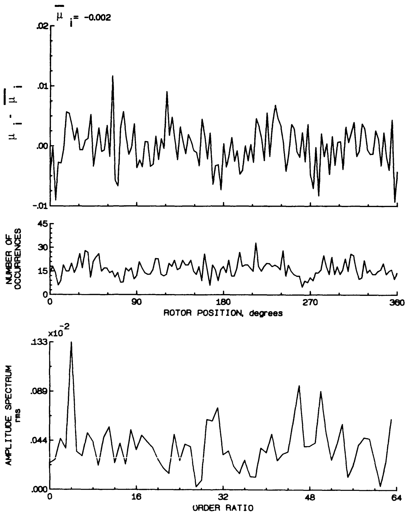
Figure 20.- Induced inflow velocity measured at 0 degrees and r/R of 0.86.
