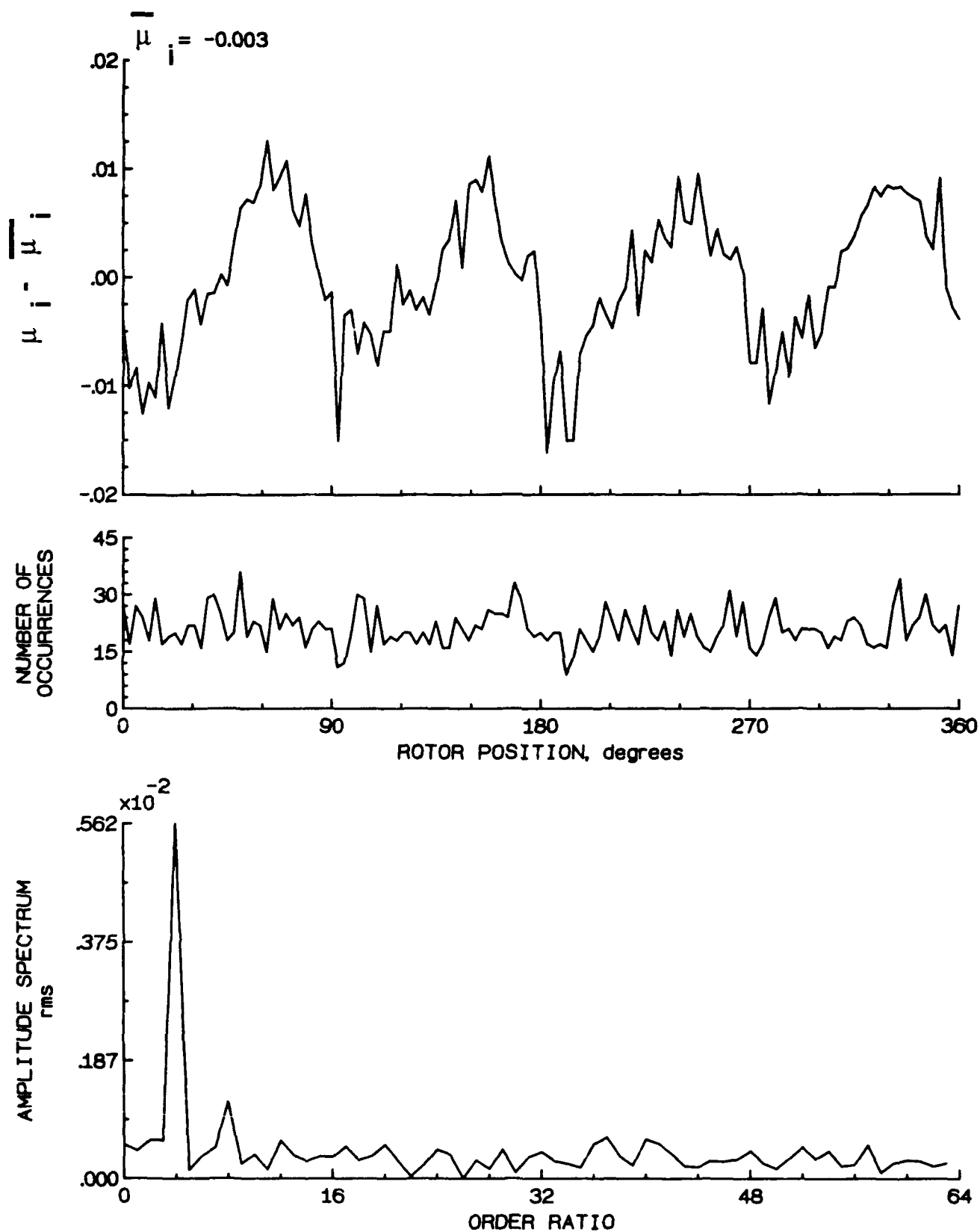
Figure 148.- Induced inflow velocity measured at 270 degrees and r/R of 0.60.
