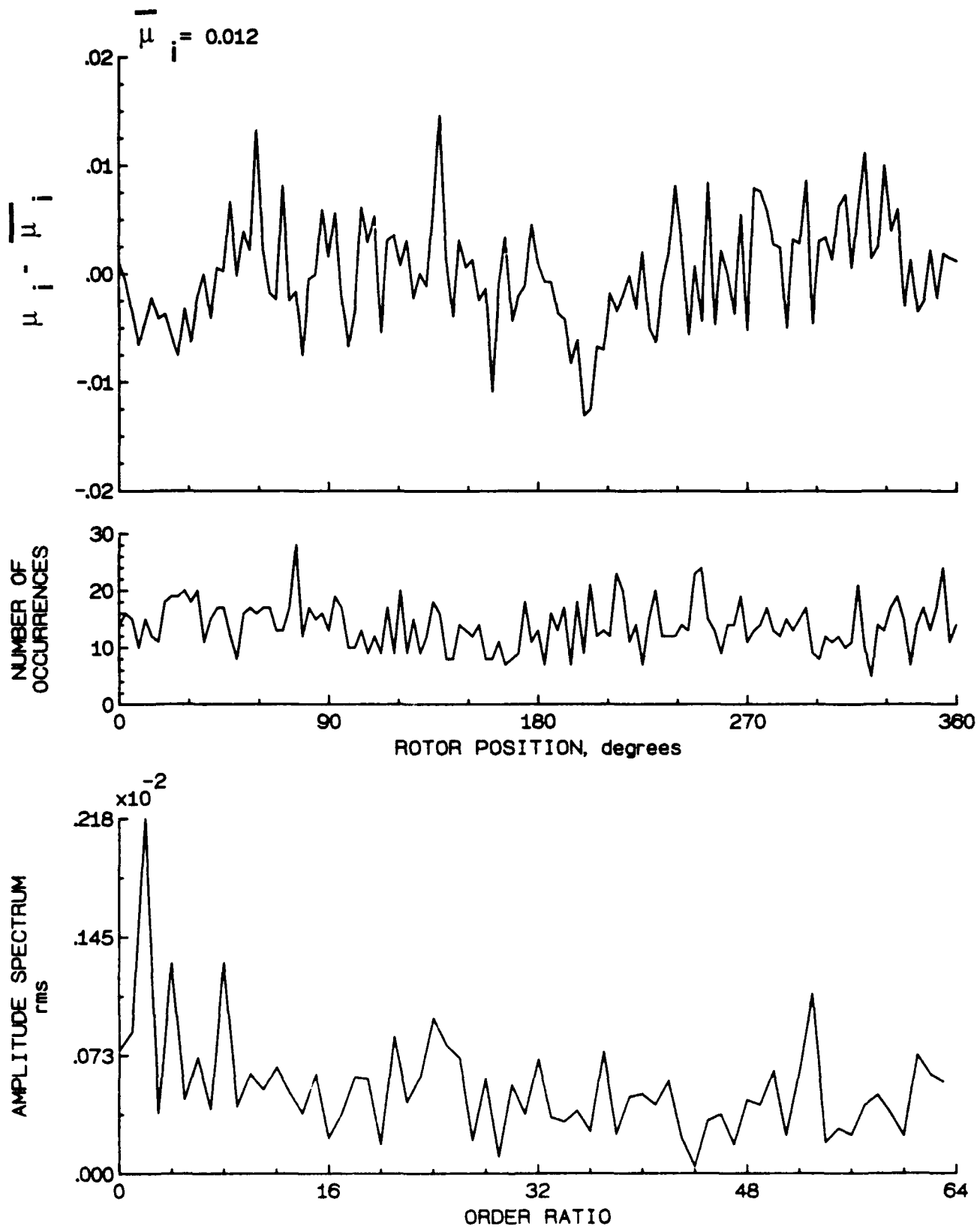
Figure 27.- Induced inflow velocity measured at 30 degrees and r/R of 0.20.
