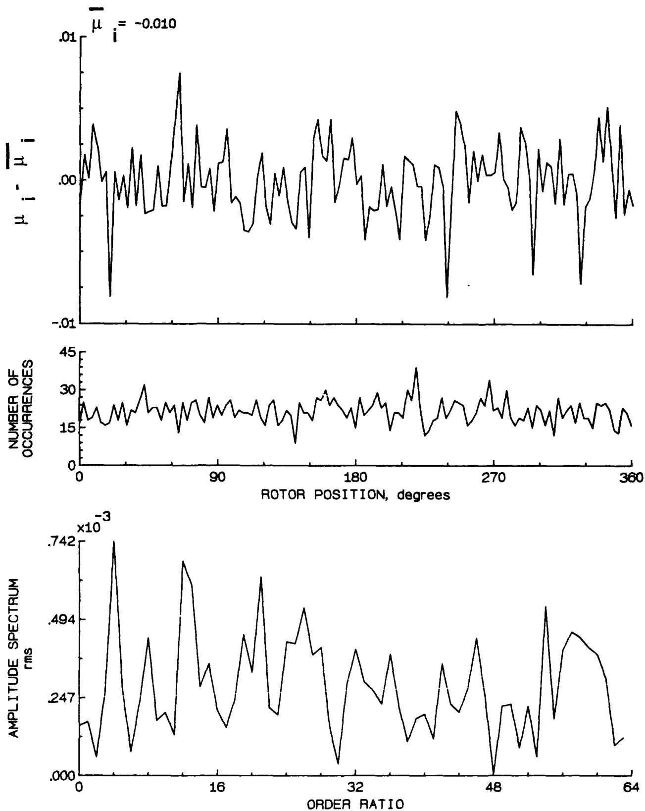
Figure 99.- Induced inflow velocity measured at 150 degrees and r/R of 1.02.
