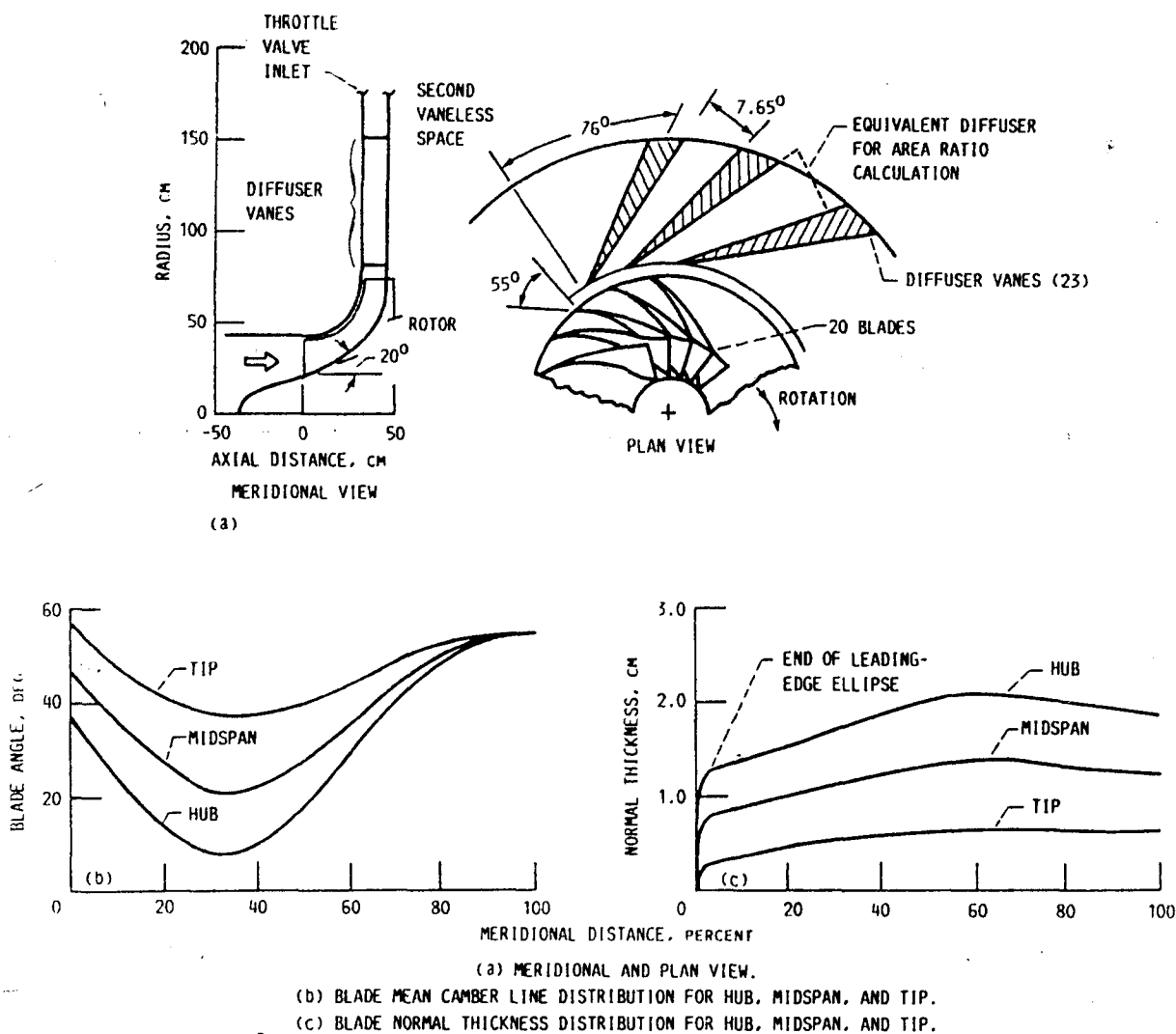
Figure 2 Configuration of low-speed centrifugal compressor initial stage design.
