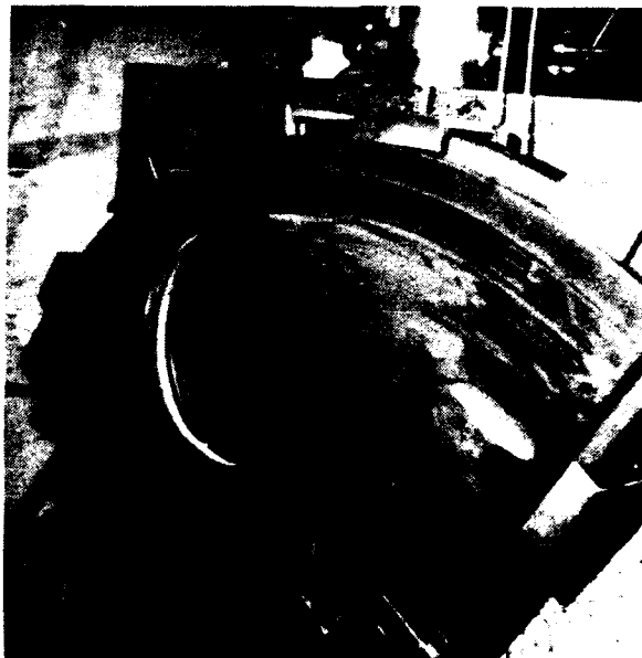
Figure 18. Graphite Seal Plate Being Held in Place by Clips
