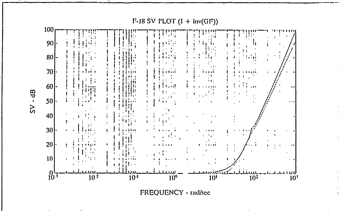
Figure 4-16 SV Plot of I + (G(s)F(s))^{-1} , H_\infty Design F-18
