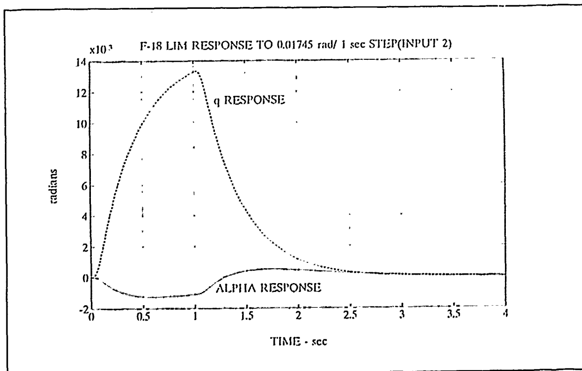
Figure 4-44 Lim. Perf. H_\infty \alpha & q Resp. to 1^\circ/\text{s} 1-sec Pulse at u_2
