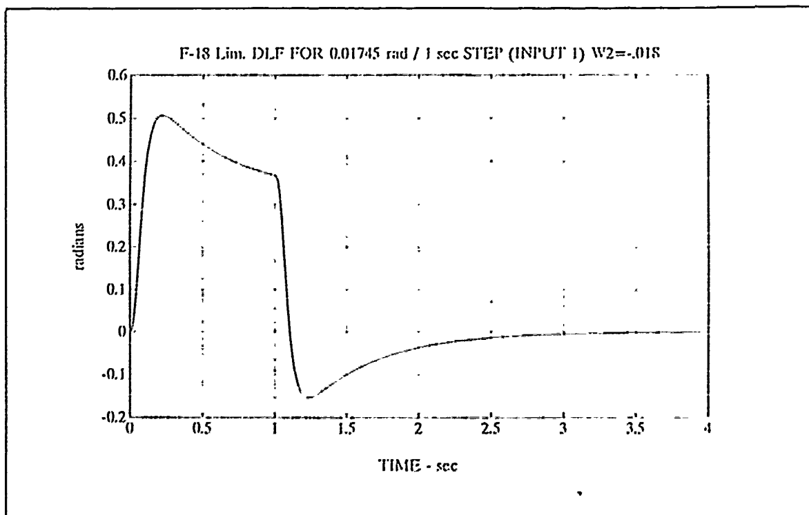
Figure 4-46 Lim. Perf. Leading Flap \delta_{lf} to 1^\circ 1-s Pulse in u_1
