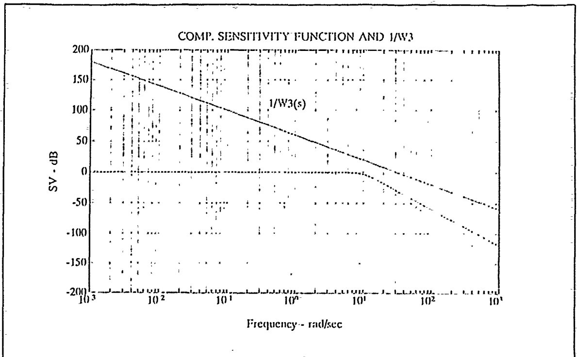
Figure 4-10 H2 Complementary Sensitivity Function T(s) , \gamma=1
