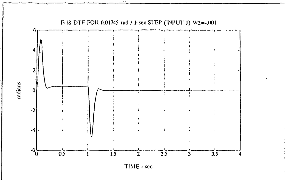
Figure 4-27 Trailing Flap Response to 1^\circ 1-sec Pulse in u_1 , H_\infty
