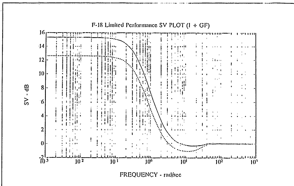
Figure 4-35 Limited Perf. SV Plot of (1 + GF) , \gamma=1.58
