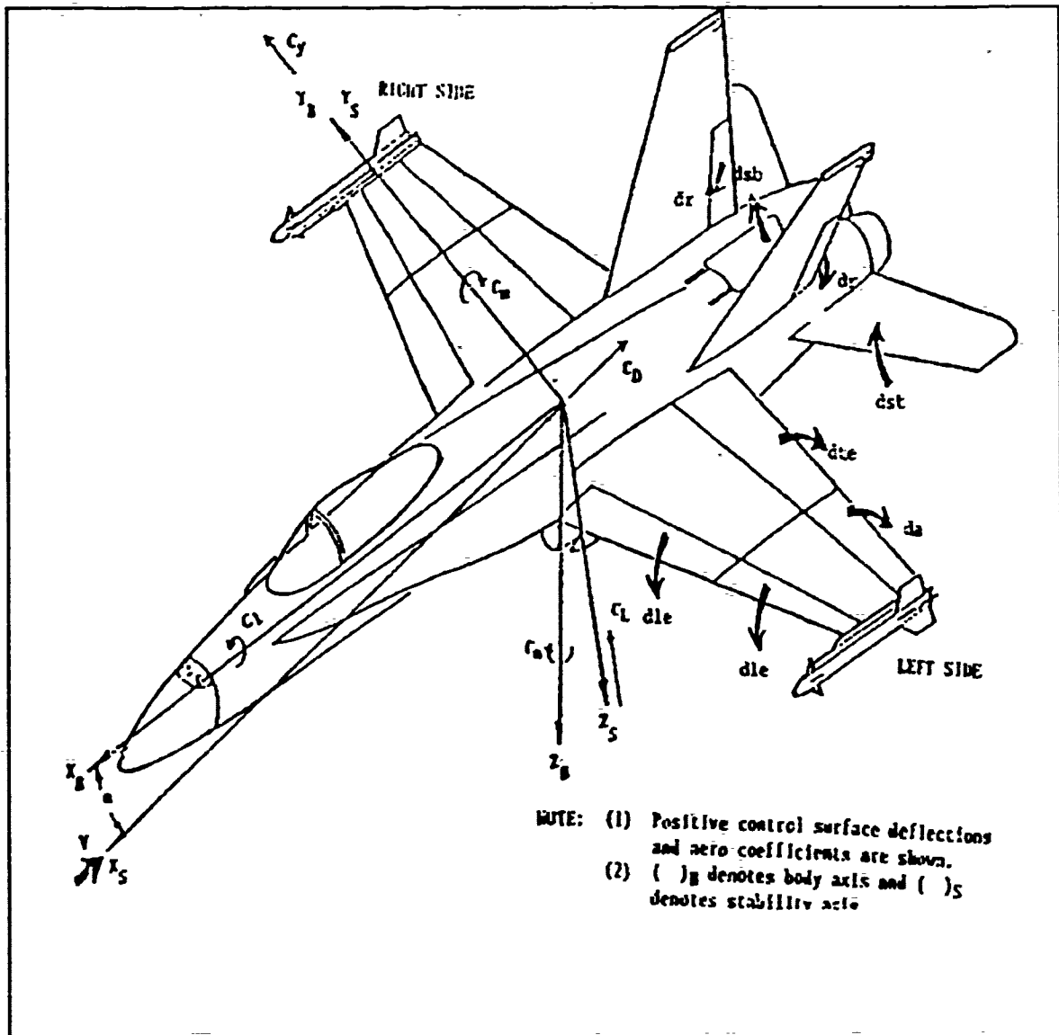
Figure 4-1 F-18 Control Surfaces and Sign Conventions
