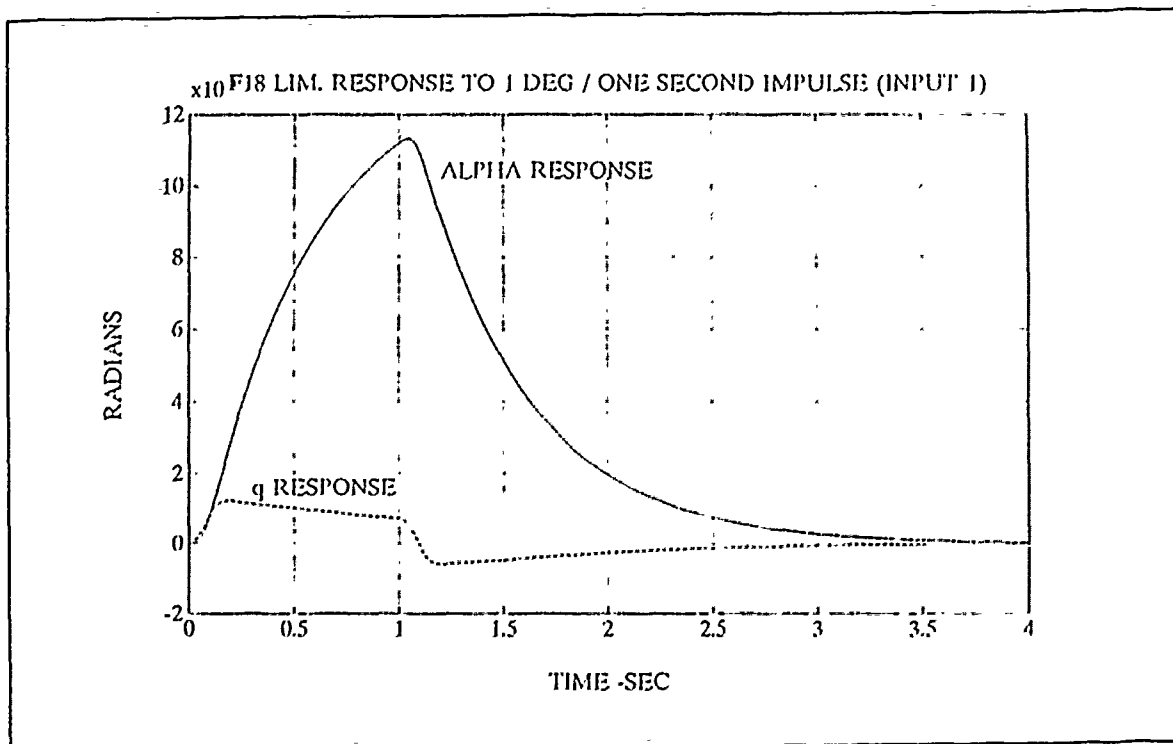
Figure 4-43 Lim. Perf. \alpha and q Resp. to 1^\circ/\text{s} 1-s Pulse at u_1
