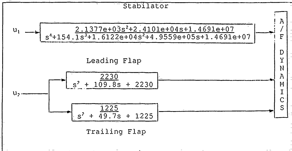
Figure 4-2 Uncompensated F-18 Open Loop Configuration
