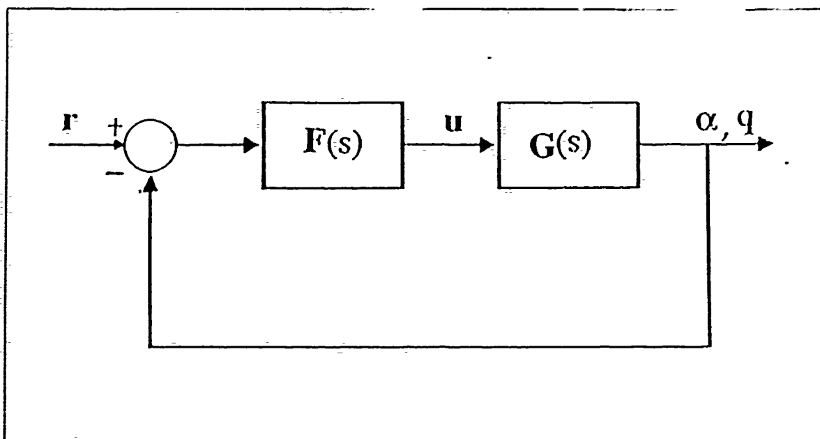
Figure 4-13 Feedback Configuration
