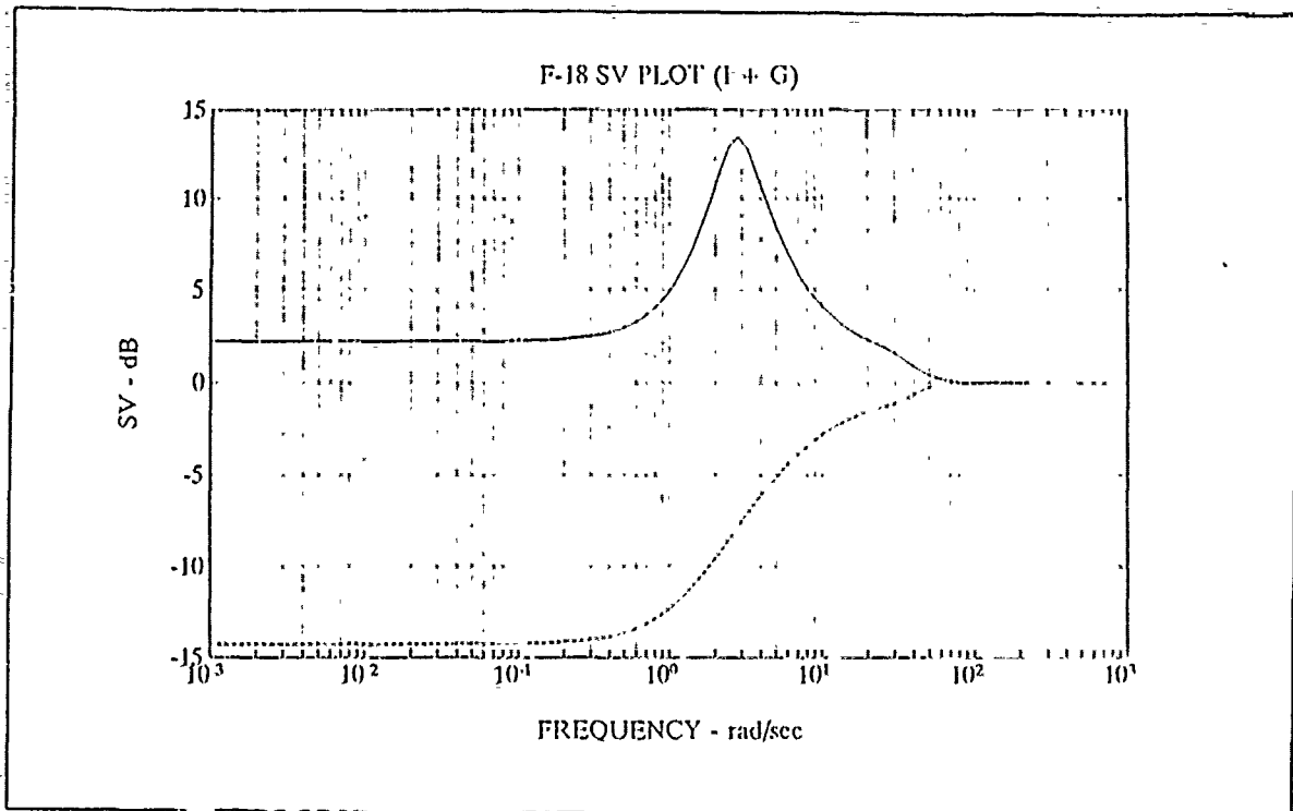
Figure 4-14 Singular Value Plot I+G(s) , Uncompensated F-18
