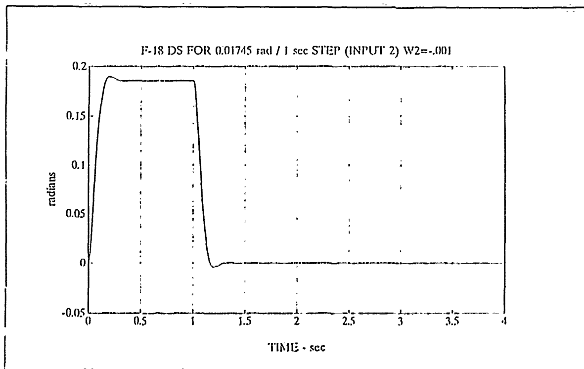
Figure 4-28 Stabilator Response to 1^\circ/\text{sec} 1-sec Pulse in u_2 , H_\infty
