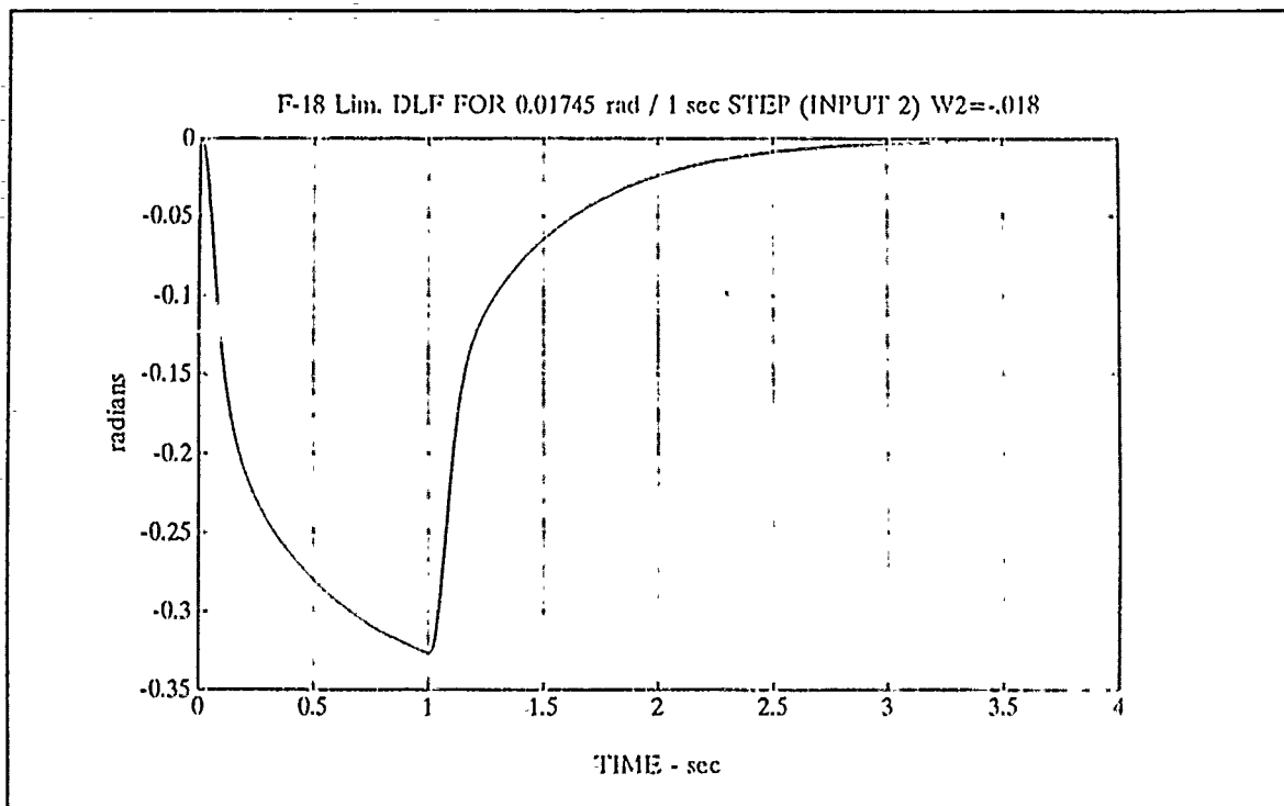
Figure 4-49 Lim. Perf. Leading Flap \delta_{lf} to 1^\circ/s 1s Pulse at u_2
