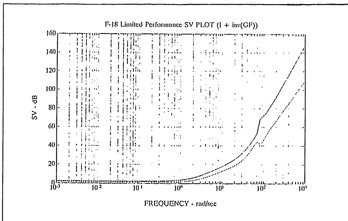
Figure 4-36 Limited Perf. SV plot of [1 + (GF)^{-1}] , \gamma=1.58
