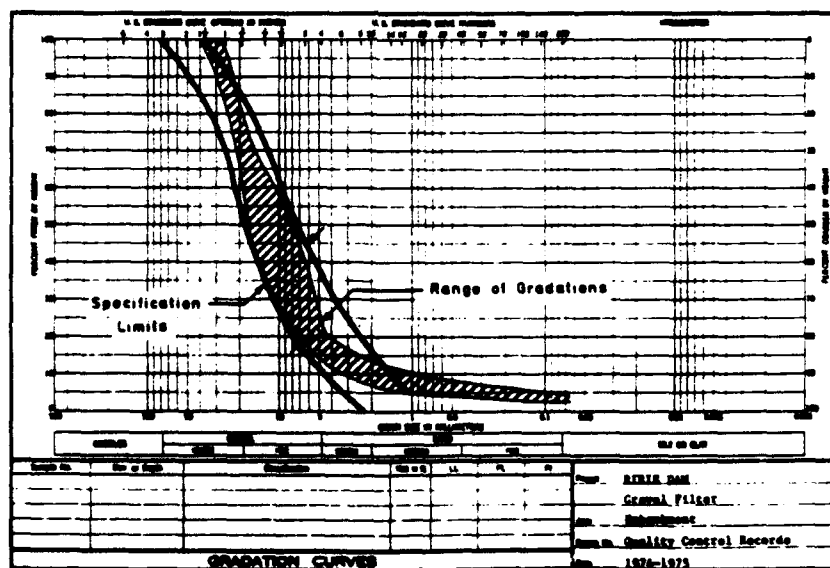
Figure 6. Range in gradations and criteria for sand filter and gravel filter
