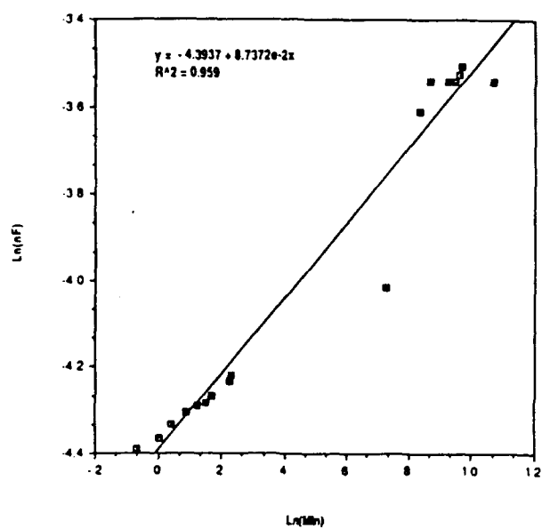
Figure 7. Long Term Capacitance Effects (0 V Bias)
