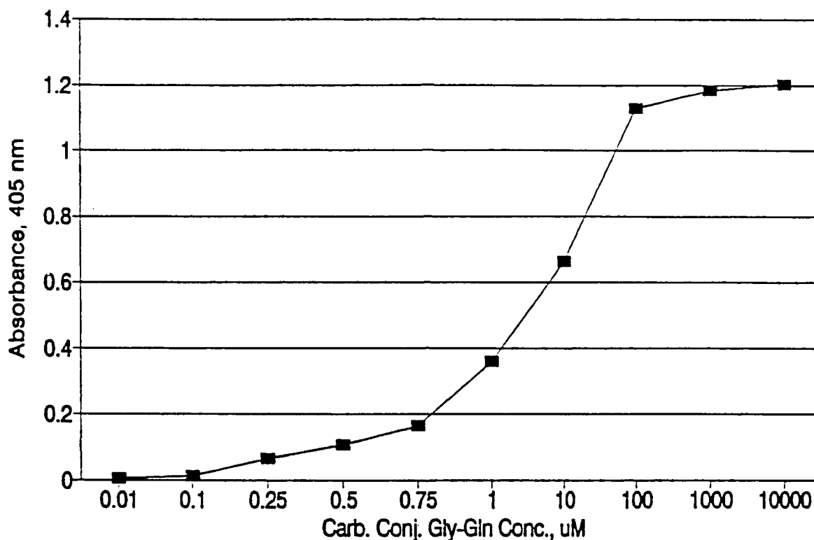
Figure 8. ELISA assay standard curve of BSA-conjugated glycyl-L-glutamine. Glycyl-L-glutamine was covalently linked to BSA by carbodiimide conjugation, dialyzed and plated in 96 well microtiter plates. BSA-conjugated glycyl-L-glutamine was detected using a primary antisera dilution of 1:10,000 followed by goat anti-rabbit IgG coupled to alkaline phosphatase. The carbodiimide conjugated glycyl-L-glutamine concentration (carb. conj. Gly-Gln conc.) was estimated from the glycyl-L-glutamine concentration used in the conjugation reaction. The limit sensitivity of the assay is approximately 1 pmol.
