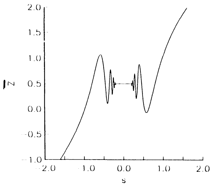
Figure 12. Plot of the composite solution \bar{Z} versus s for \theta = \pm \pi/2 , with k_1 = 0.5 , k_2 = 1 , \delta = 0.05 , and \bar{t} = 1 .
