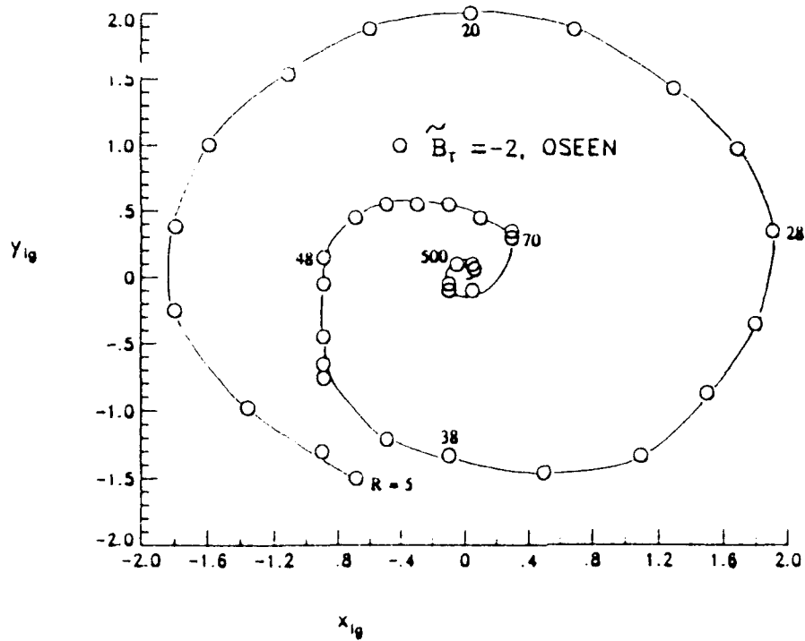
Figure 2. Plot of the ignition locations y_{ig} versus x_{ig} for various values of the vortex Reynolds number with Sc = \phi = 1 and \beta_T = -2 .
