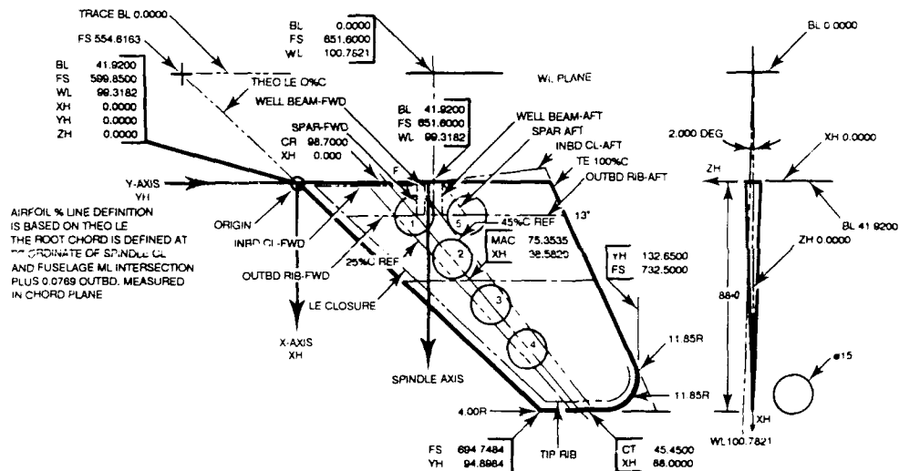
FIGURE 2. F-18 HORIZONTAL STABILATOR DEFINITION
