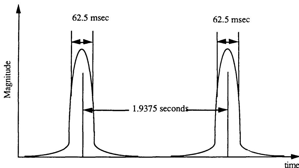
Figure 2.3. Magnitude of Transmitted Signal after Demodulation and m-Sequence Removal.
