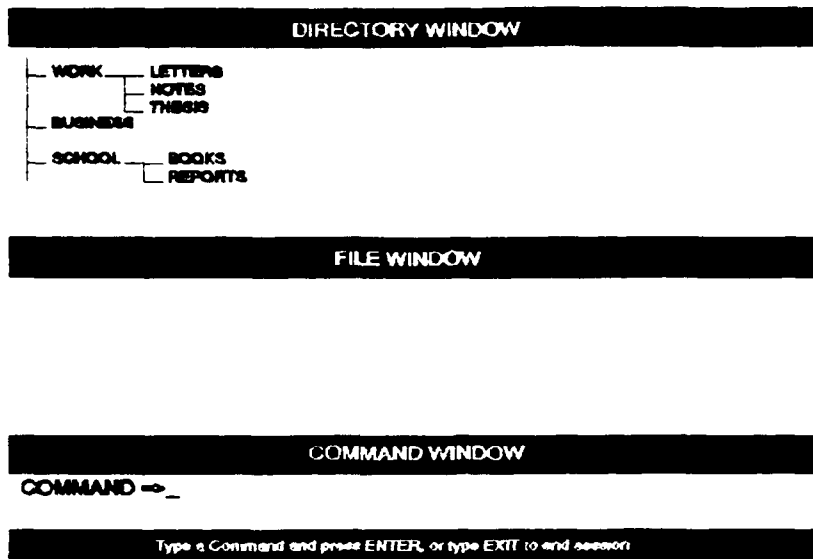
Figure 2. The Command Language Interface Windows.
