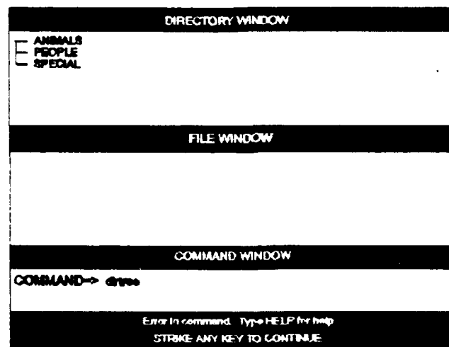
Figure 2. Command Language Screen Containing Error Message
