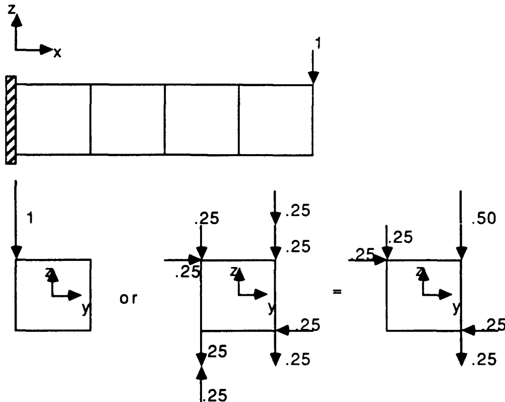
Figure 20. Square Beam Model
