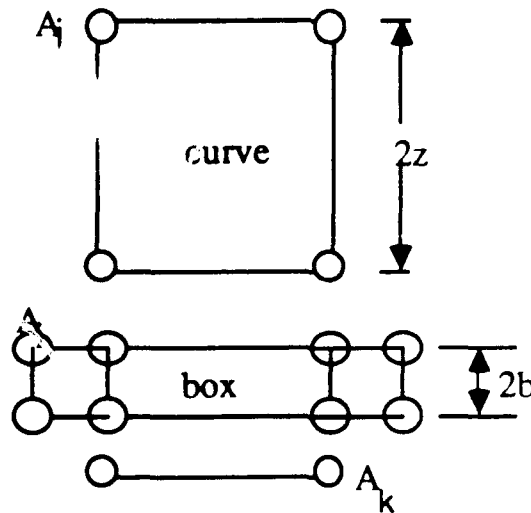
Figure 9. Idealized Fuselage Cross Section
