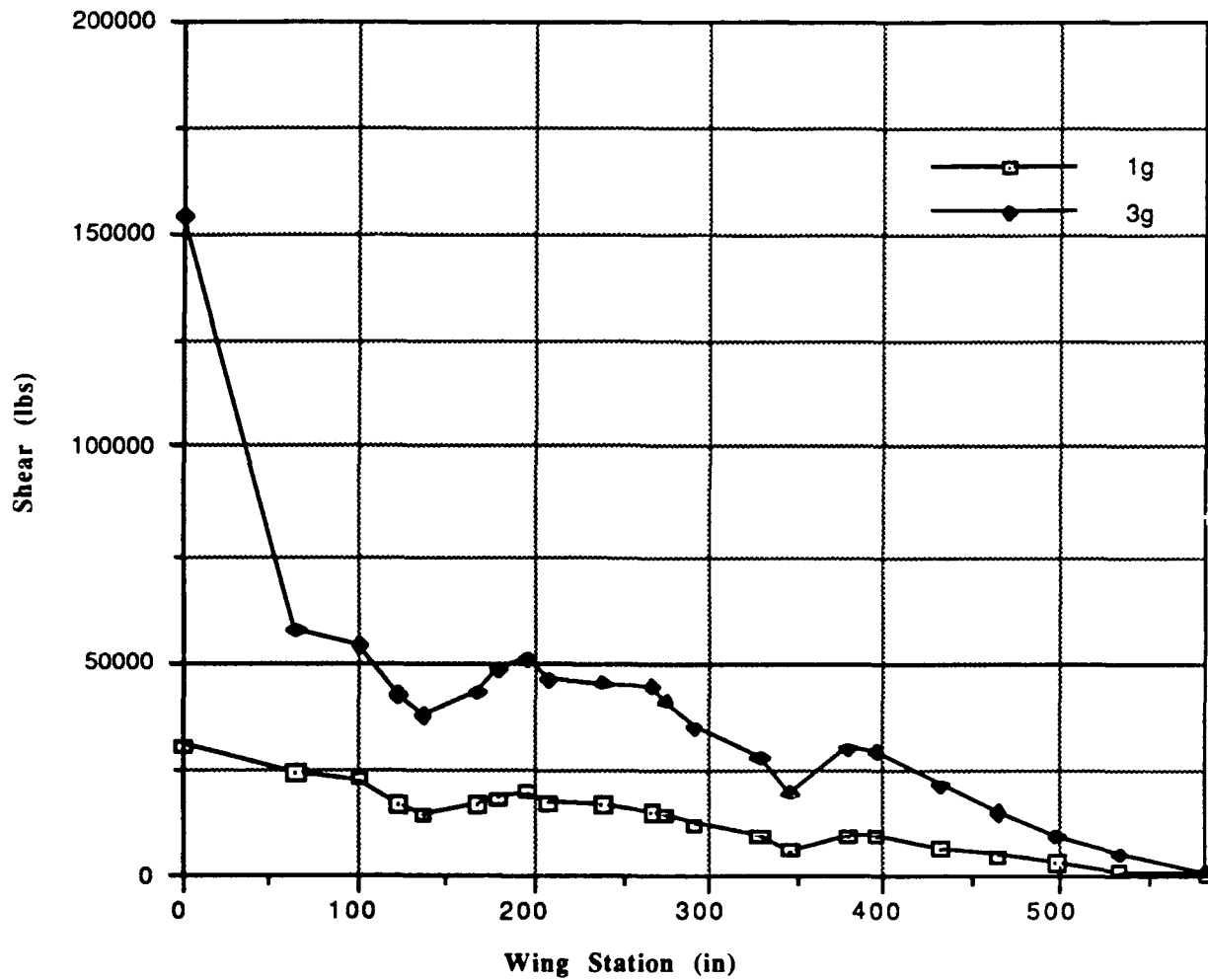
Figure 18. P-3C Wing Shear : 135,000 pounds gross weight.
