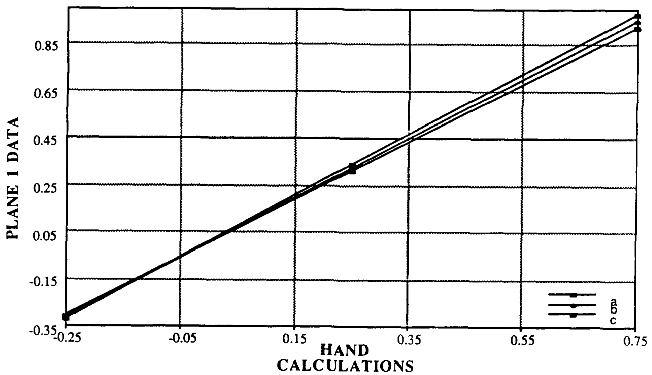
Figure 24. Plane 1 Results
