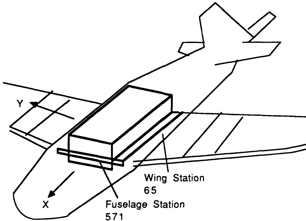
Figure 14. Stress Locations
