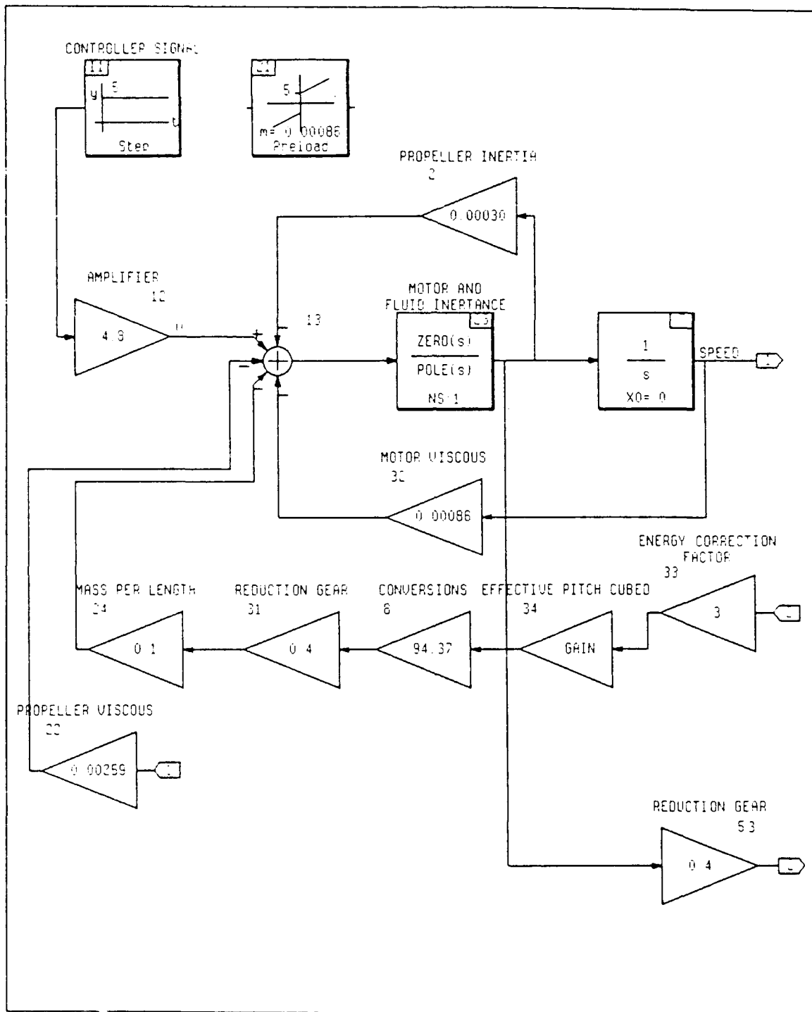
Figure 12 Tunnel Thruster Model--Left Side
