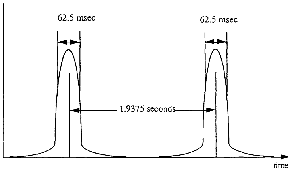
Figure 2.4: Acoustic arrival after demodulation and matched filtering.
