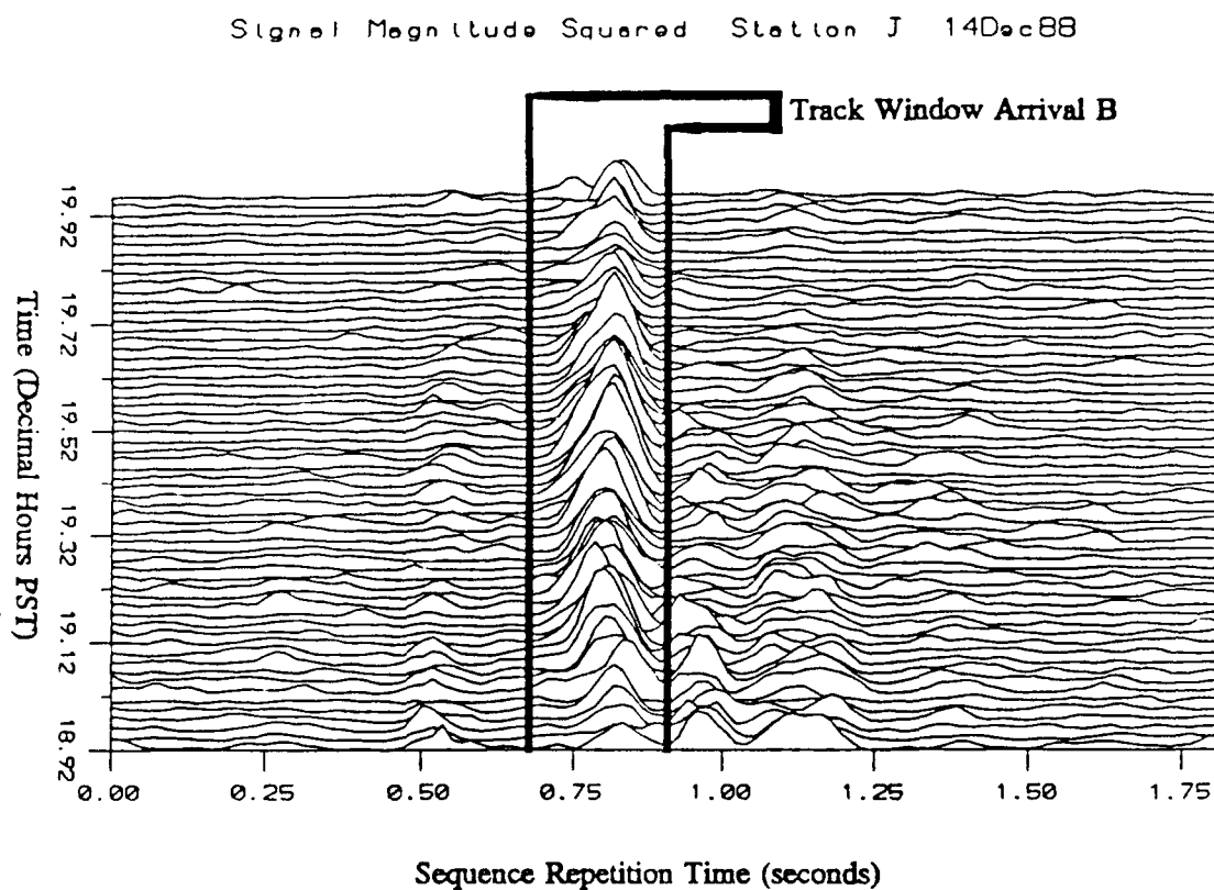
Figure 2.8: Waterfall display of received acoustic signals from station J, 14 Dec 88. Each trace is 31 seconds of data coherently averaged to one 1.9375 second maximal-length sequence period.
