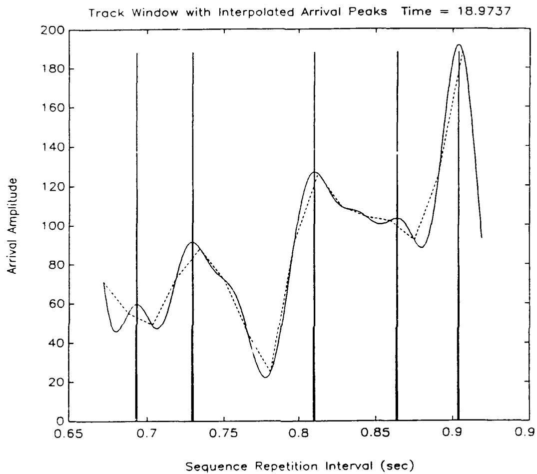
Figure 2.13: Station J arrival B 16 point track window FFT interpolated to 512 points, showing the positions of the local maxima located by a numerical second derivative operation.
