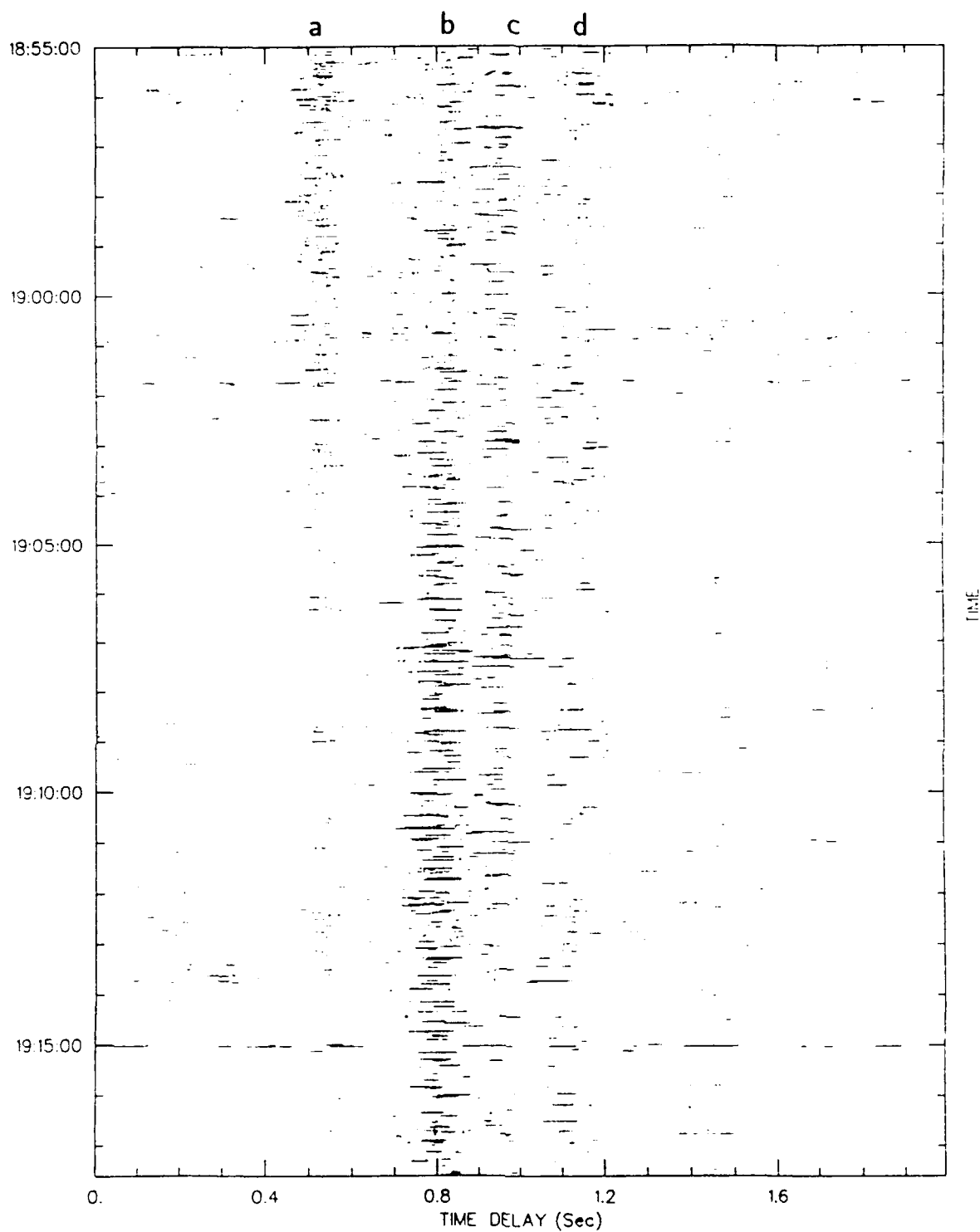
Figure 2.10: Correlogram display of received acoustic signals from station J, 14 Dec 88. Consecutive unaveraged 1.9375 second maximal-length sequence periods are quantized, converted to pixels and stacked to form a greyscale plot of the data.
