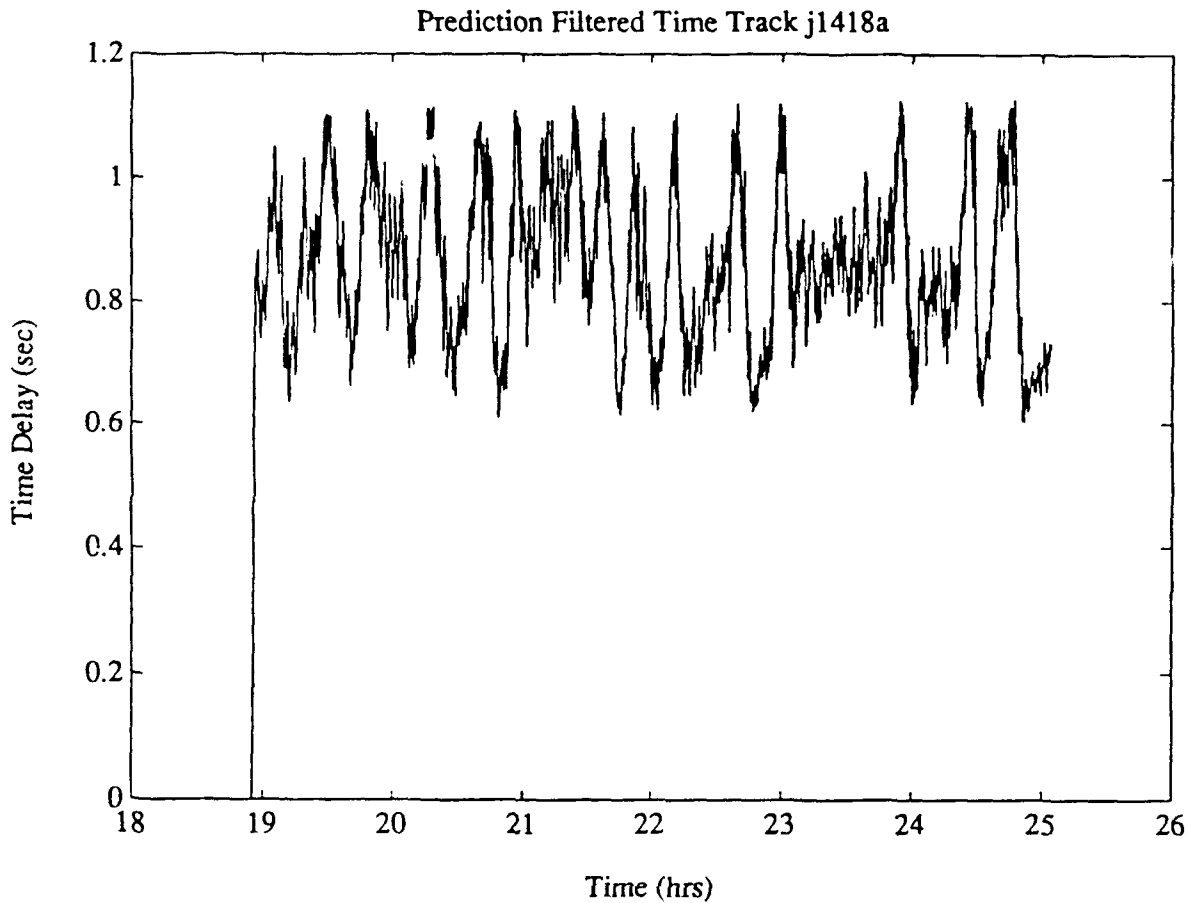
Figure 3.11: Arrival B station J track generated at the output of the LMS adaptive filter with applied amplitude bias in the arrival selection.
