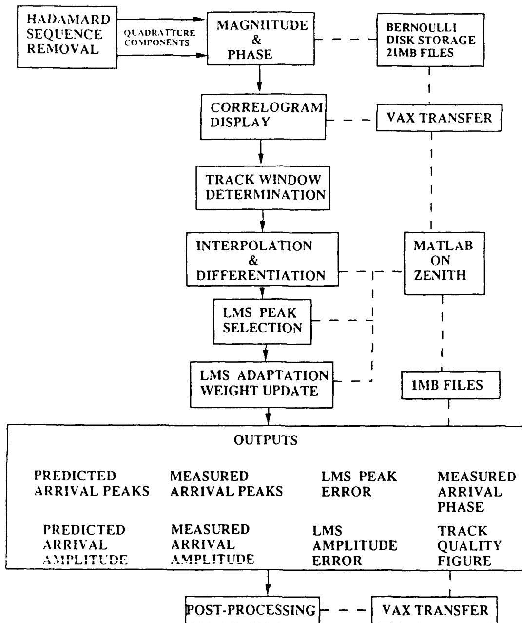
Figure 3.6: Schematic block diagram of LMS peak tracking algorithm.
