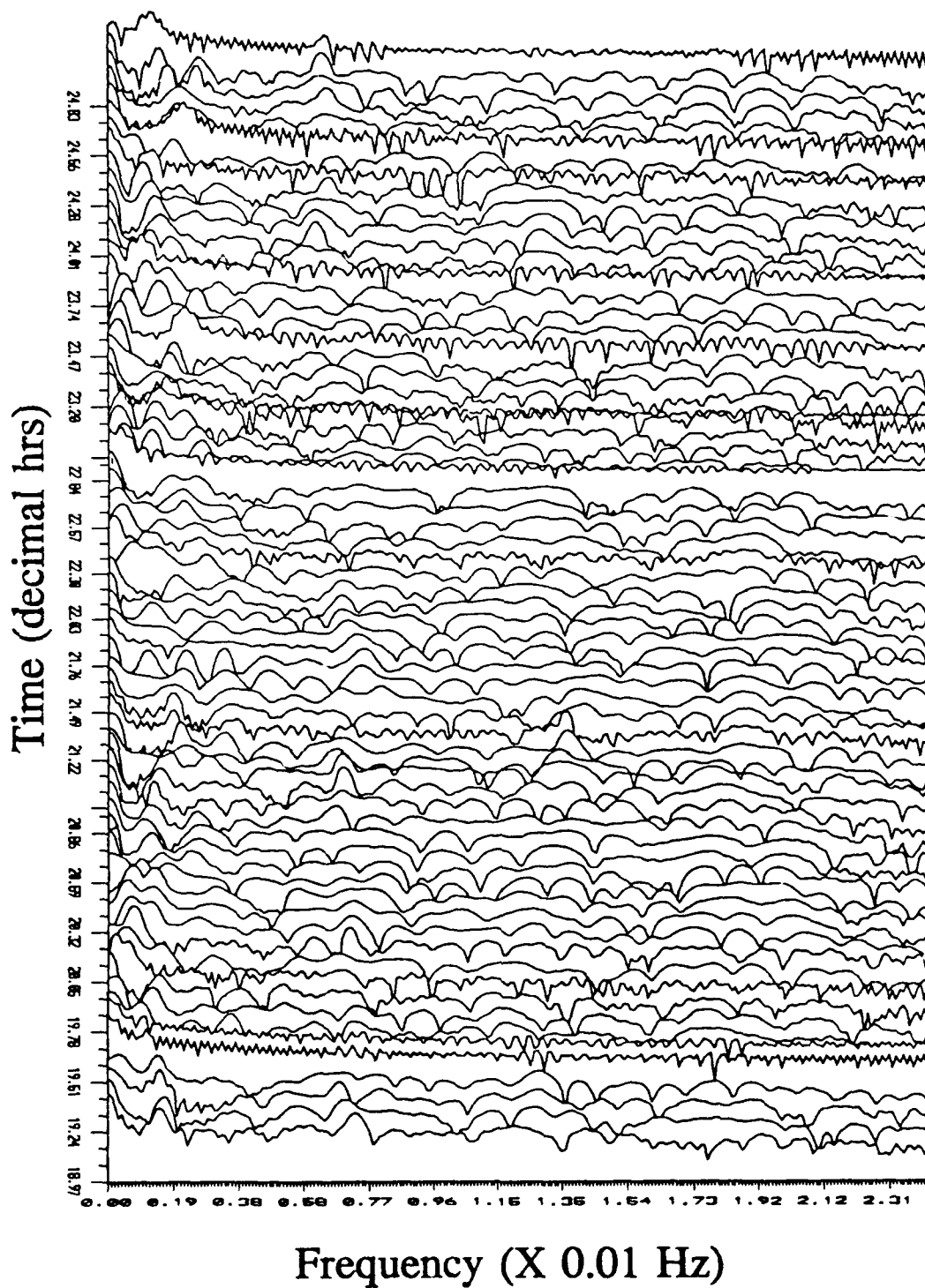
Figure 5.6: Dynamic spectral waterfall display at internal wave frequencies for arrival C station J.
