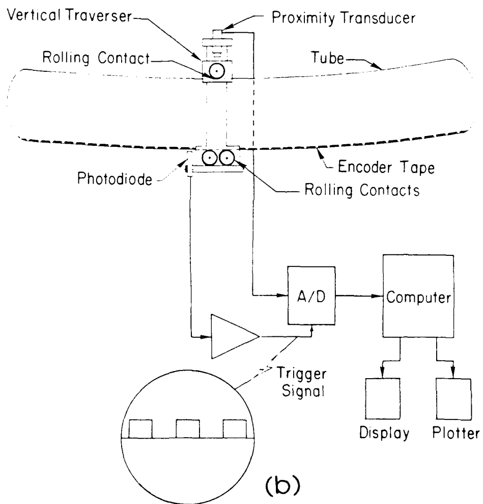
Fig. 7 (a) Transducer for scanning ovalization along shell length (b) Transducer schematic and A/D converter triggering circuit
