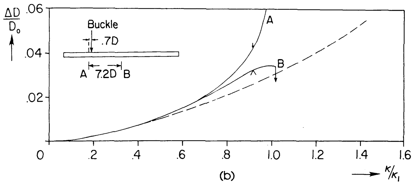
Fig. 18 Bending response of aluminum shell with D/t = 32.2 (a) Moment-curvature (b) Ovalization-curvature
