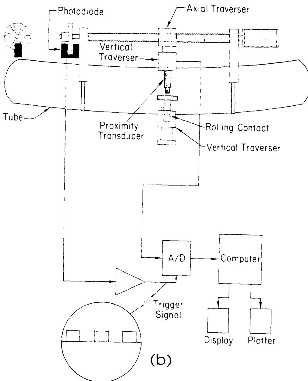
Fig. 8 (a) Ovalization transducer with high axial resolution (b) Transducer schematic and A/D converter triggering circuit
