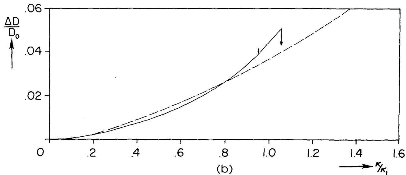
Fig. 14 Bending response of aluminum shell with D/t = 44 (a) Moment-curvature (b) Ovalization-curvature
