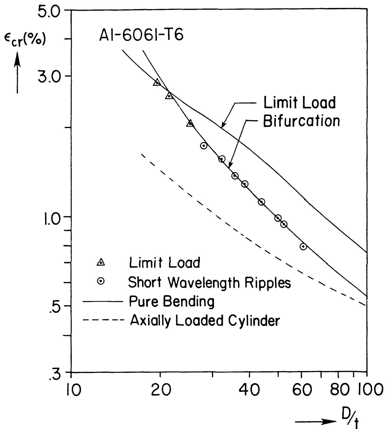
Fig. 24 Critical maximum St. Venant bending strain as a function of shell D/t . Comparison of experimental values and various predictions
