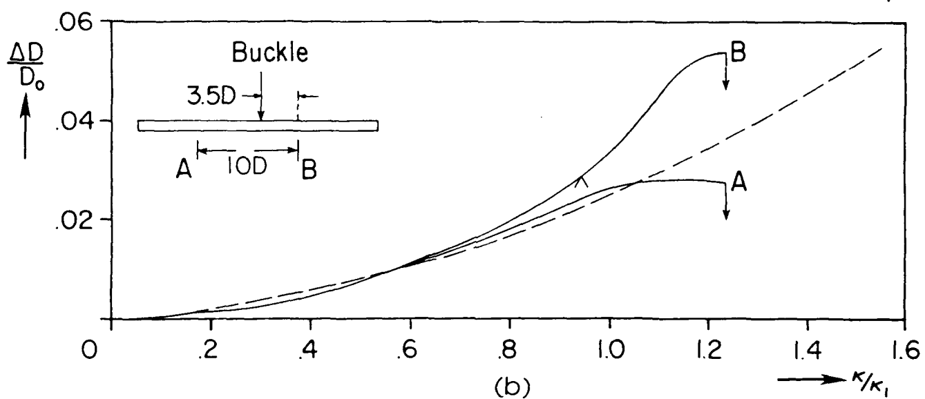
Fig. 22 Bending response of aluminum shell with D/t = 19.5 (a) Moment-curvature (b) Ovalization-curvature
