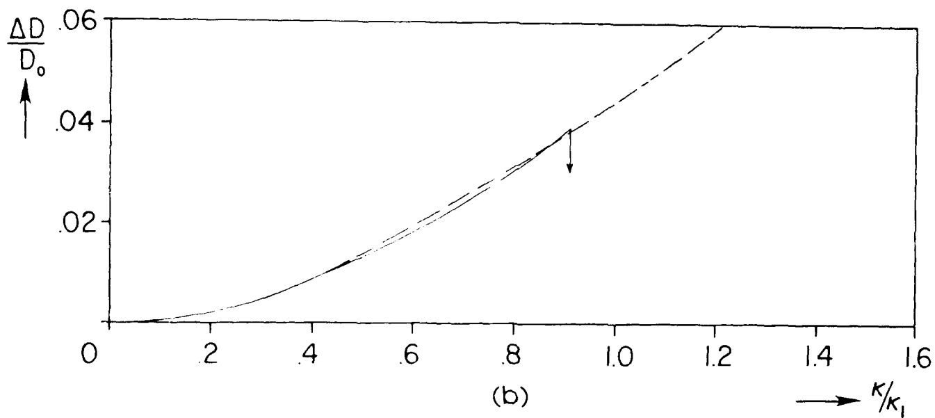
Fig. 10 Bending response of aluminum shell with D/t = 60.5 (a) Moment-curvature (b) Ovalization-curvature
