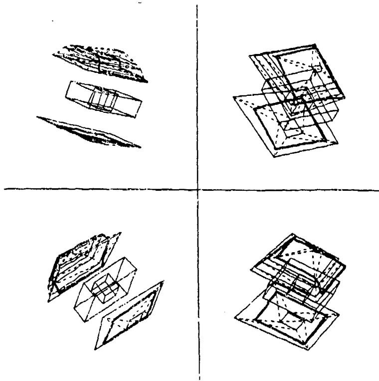
Figure 2: Example of the top and bottom cover of the cell generated by tumbling from one critical point to another along the central object's outer silhouette. The thick solid lines are the etchings on the covers; the thin solid and dashed lines are the triangulated objects.
