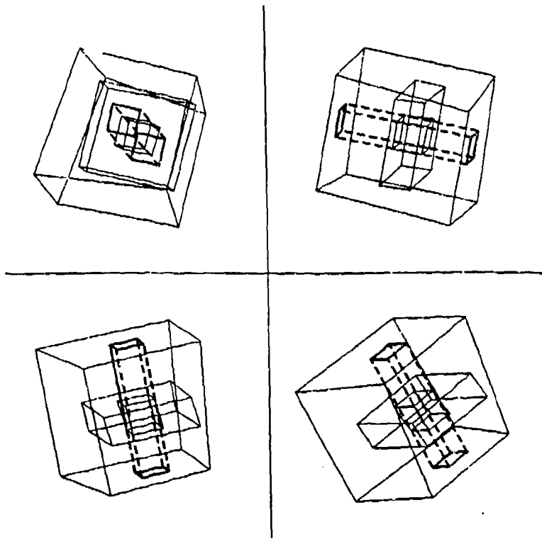
Figure 3: Example of a reconstructed cell generated by the hole in the object with covers on a surrounding object. The thick solid lines are the top and bottom covers; the thick dotted lines outline the z -vertical walls of the cell. Again the object has been rotated to afford a better view.
