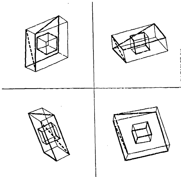
Figure 1: An example of the two silhouettes generated by an object with a hole. Thick solid lines are the full reflex edges; thick dashed lines are the inverse reflex edges; and the thin solid lines are the remaining edges of the object. The image has been rotated to provide a coherent view.
