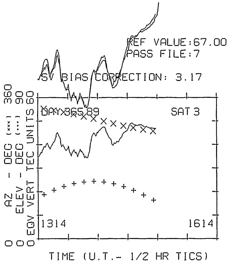
Figure 4. TEC values corresponding to S_4 records shown in Fig. 3, derived from the DGD (smoother of the two overlapping traces at the top) and DCP (more finely structured trace) measurements shown, in part, in Fig. 1. Lower solid trace is equivalent vertical TEC derived from DCP by removing effect of changing slant path-length. X and + indicate satellite azimuth and elevation, respectively. Time span is 13:14 through 16:14 UT.
