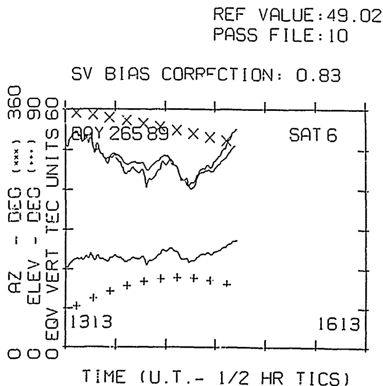
Figure 11. TEC measured during the first afternoon GPS track in Fig. 8.
