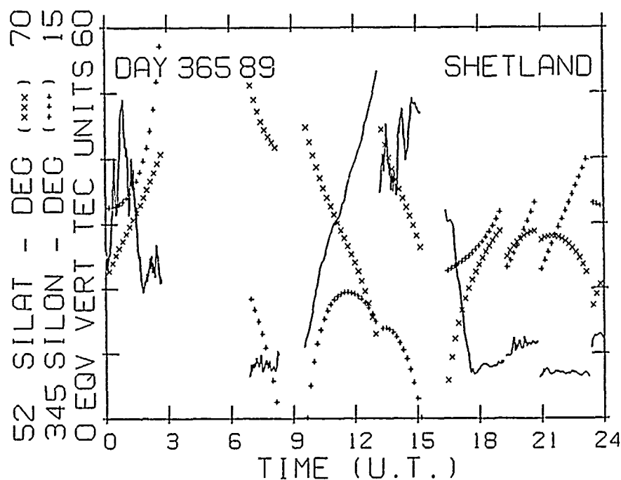
Figure 5. Synoptic chart of equivalent vertical TEC values (solid curves) derived from DCP and calibrated by means of DGD from measurements at Lerwick over the 24-hour period (31 December 1989, UT) in which the satellite track producing the data in Figs. 1, 3, and 4 occurred. x and + indicate satellite latitude and longitude, respectively.
