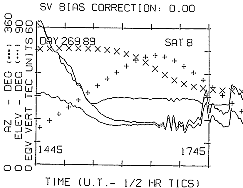
Figure 13 TEC measured during the second afternoon GPS track in Fig. 10. Note strong quasi-periodic signature centered on about 17:27 UT.
