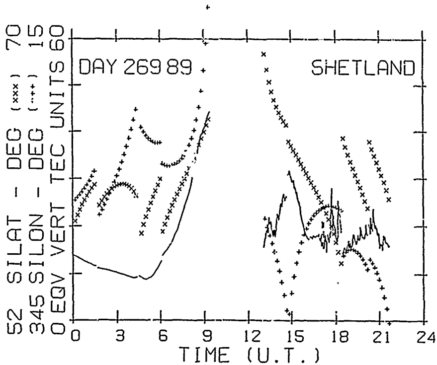
Figure 10. Synoptic chart of equivalent vertical TEC and satellite latitude and longitude for 24-hour period of 26 September 1989, UT.
