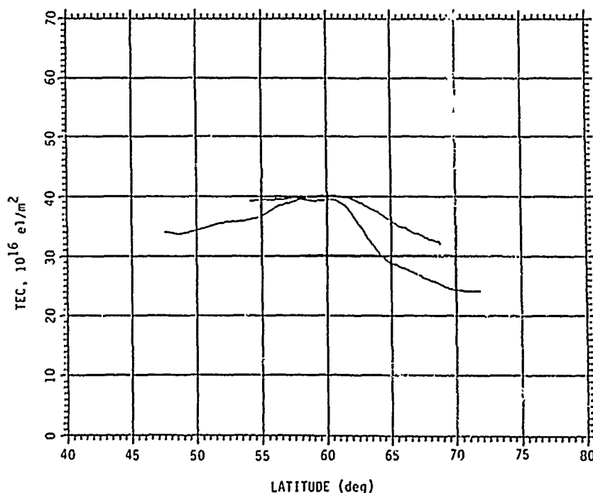
Figure 9 Latitudinal scans of TEC observed at Lerwick by means of polar-orbiting "Transit" satellites between 0906 and 0918 UT (shallow curve) and between 1518 and 1529 UT (steeper curve) on 22 September 1989. The former was approximately along the 353-deg meridian, and the latter approximately along the 4-deg meridian. (Data provided by L. Kersley via G. Bishop.)
