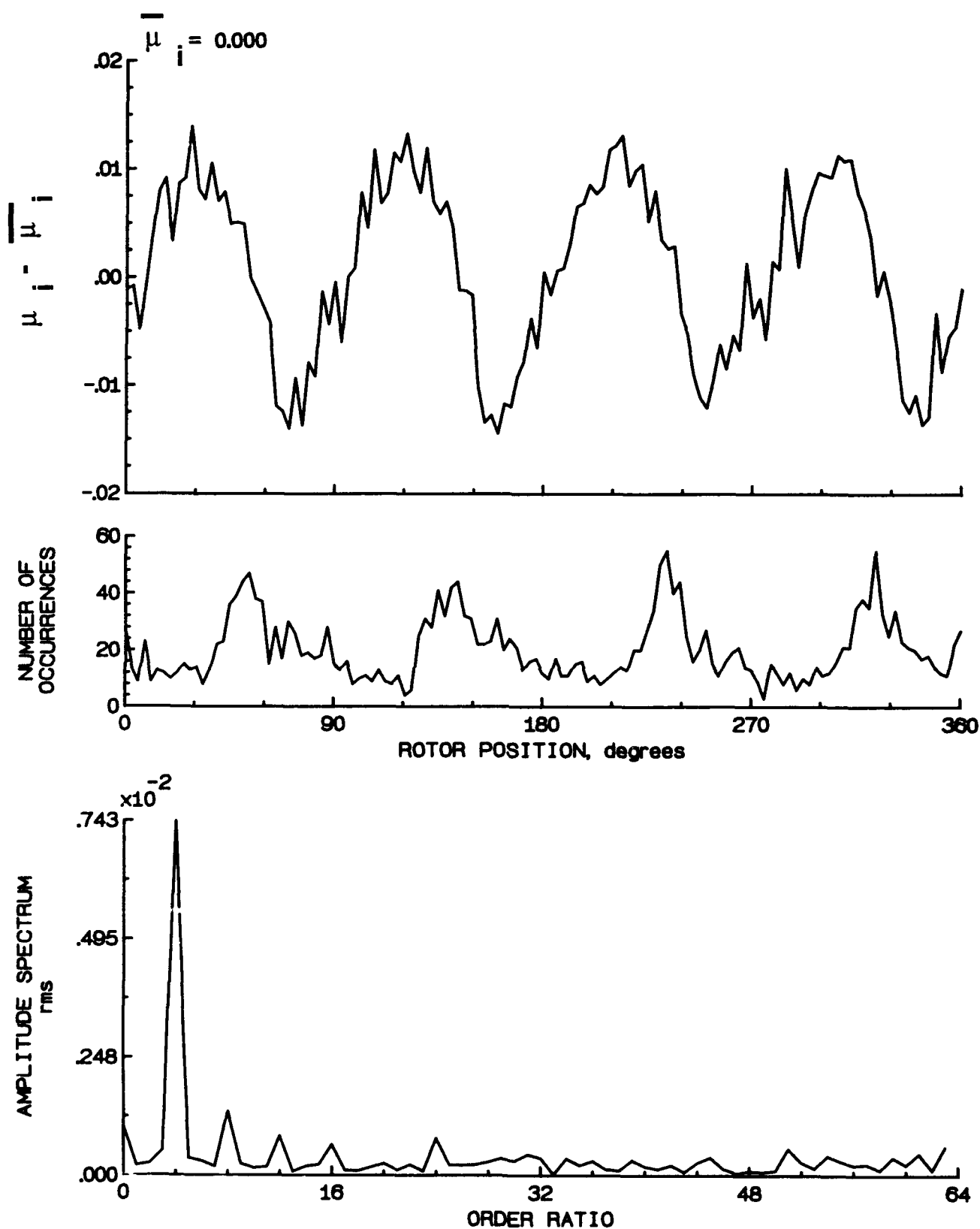
Figure 134.- Induced inflow velocity measured at 240 degrees and r/R of 0.60.
