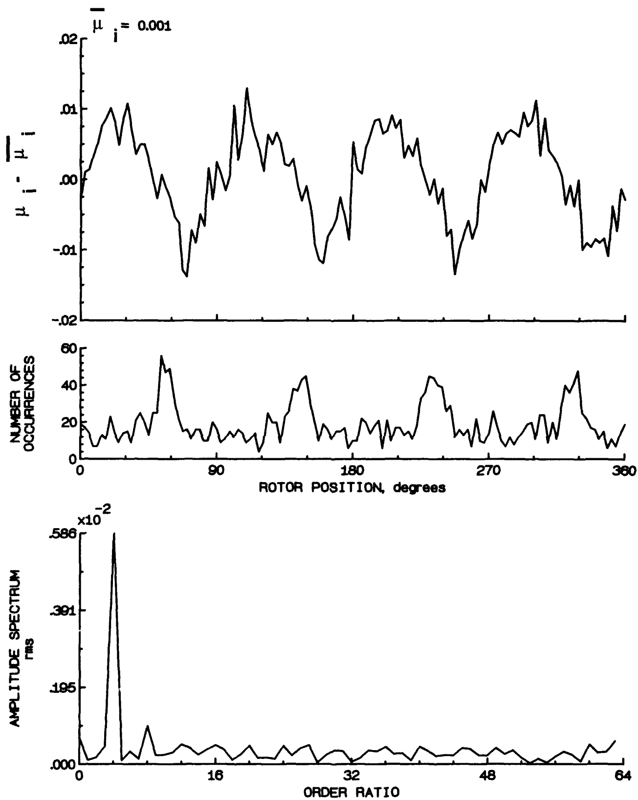
Figure 135.- Induced inflow velocity measured at 240 degrees and r/R of 0.70.
