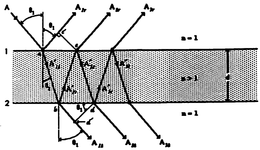
Figure 2.1 - Multiple Beam Interference in Nonabsorbing Fabry-Perot Etalon.
