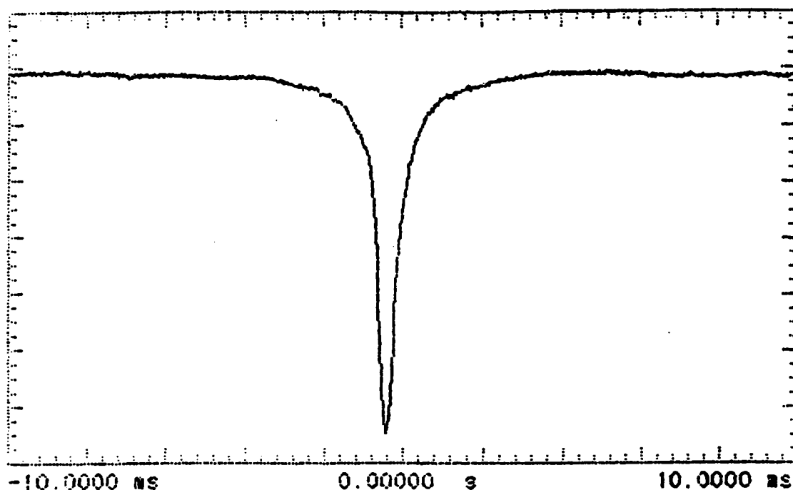
Figure 4.2 - Autocorrelation Trace of 2 Picosecond Pulses at 1.3 \mu\text{m} .
