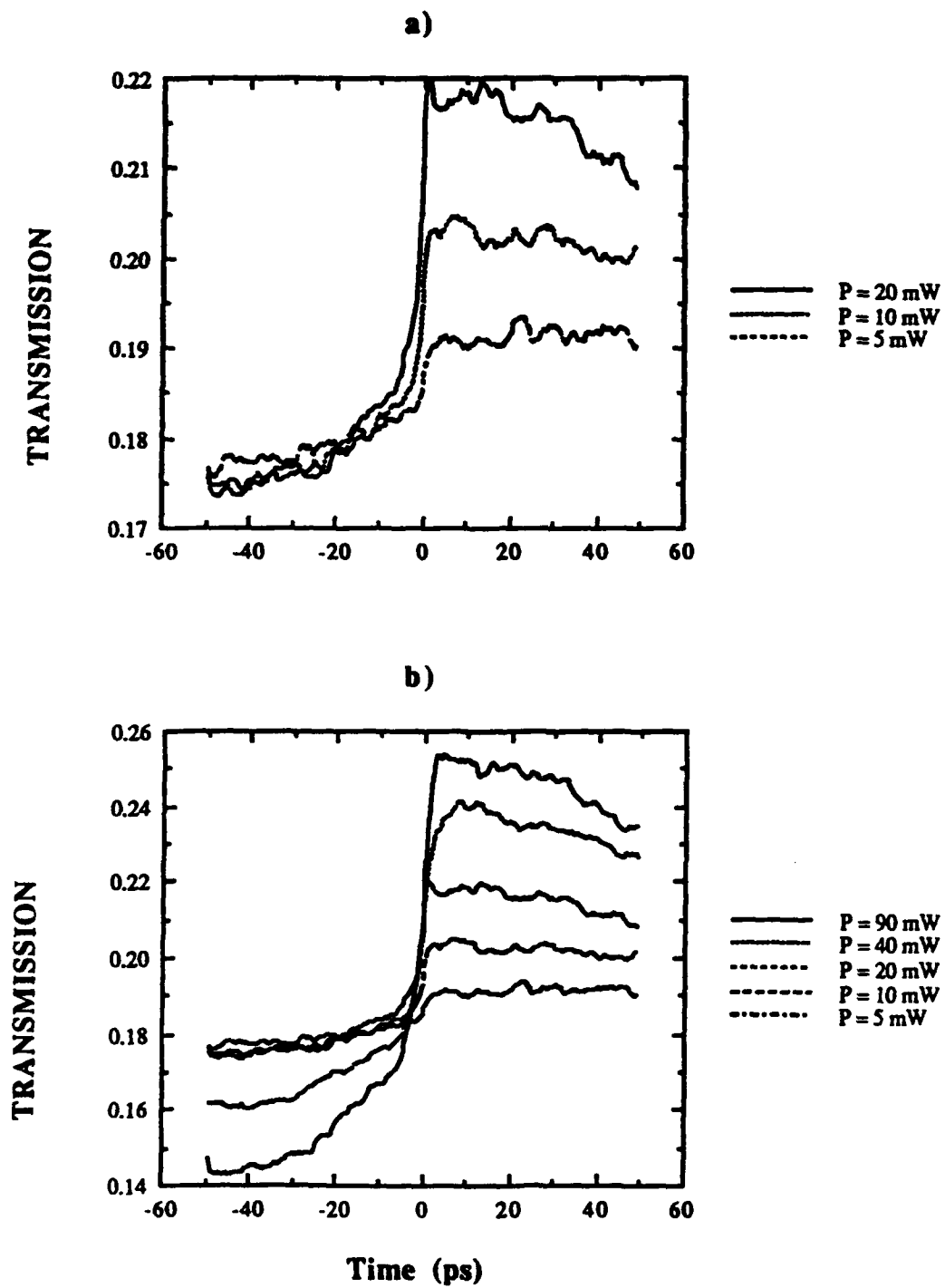
Figure 4.4 - Switching Characteristics for GaInAs Etalon.
