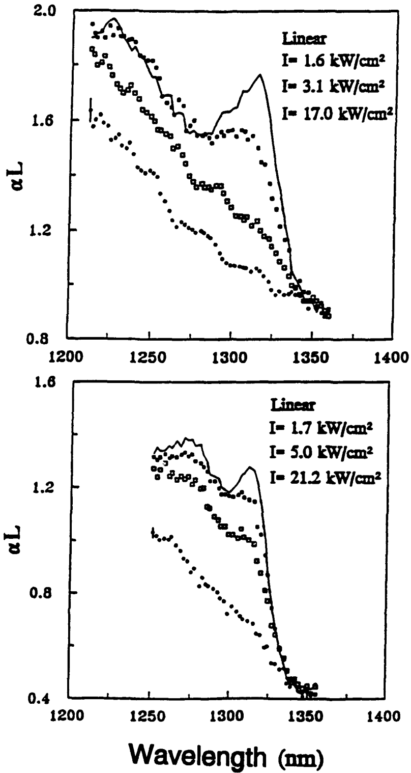
Figure 4.7 - Exciton Saturation in a) GaInAs and b) GaAlInAs MQWs.
