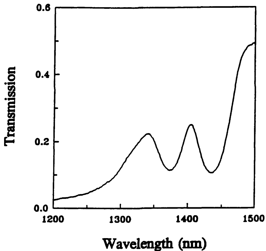
Figure 3.4 - White Light Transmission Spectrum for GaInAs Etalon.
