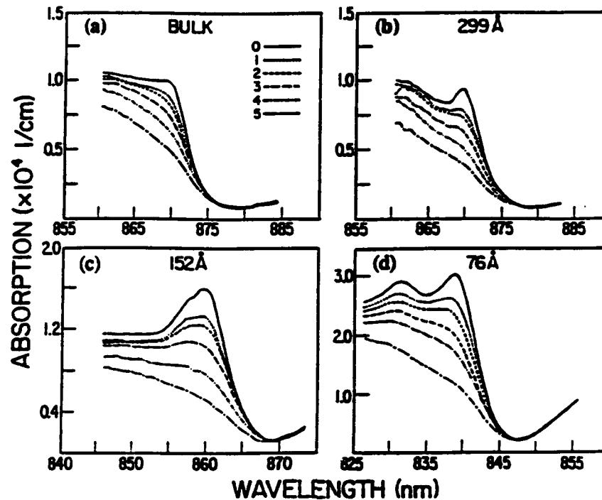
Figure 3.2 - Absorption Spectrum for GaAs MQWs as a Function of Well Width.
