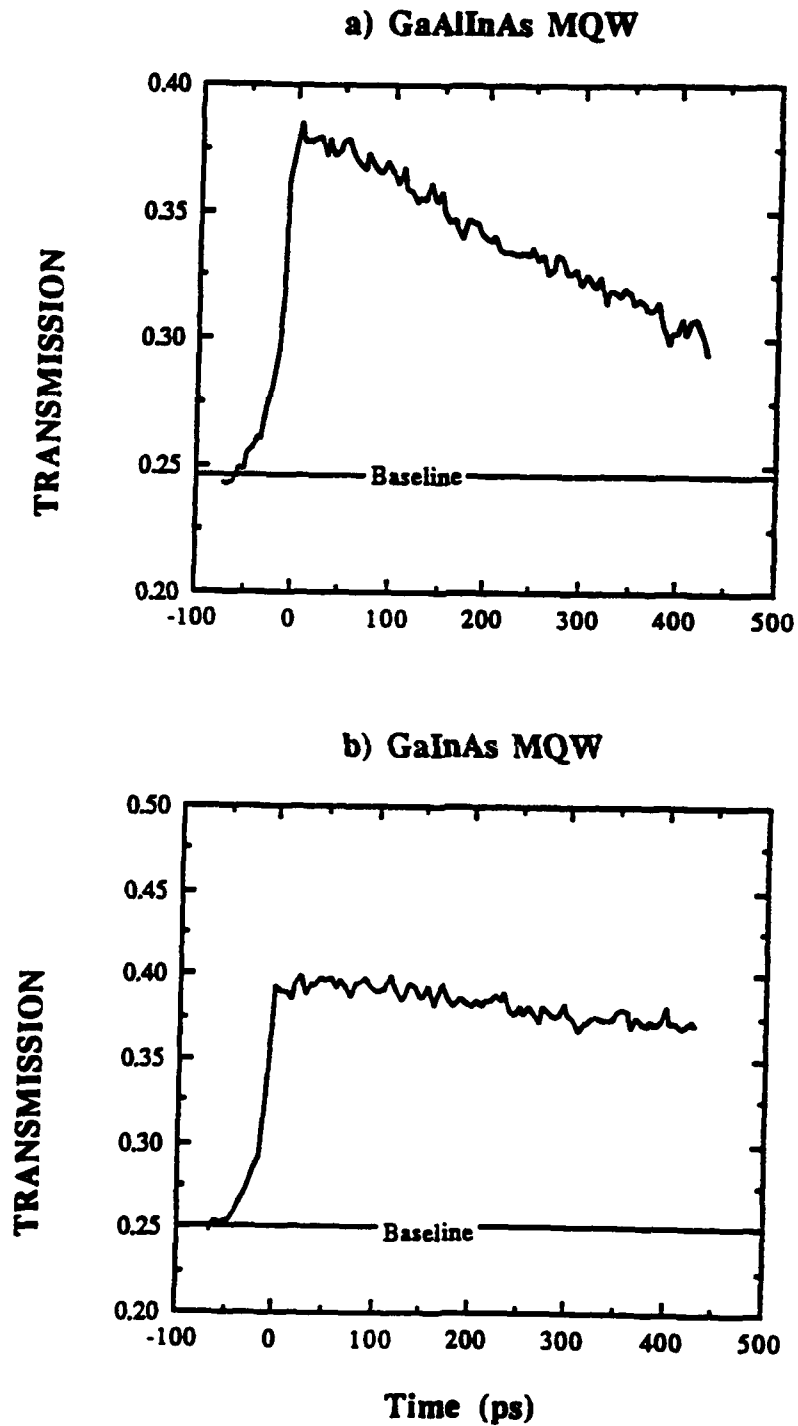
Figure 4.5 - Carrier Lifetimes for a) GaAlInAs and b) GaInAs.
