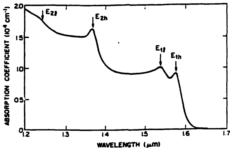
Figure 3.1 - Typical Shape of Room-Temperature Absorption Spectrum for MQWs.
