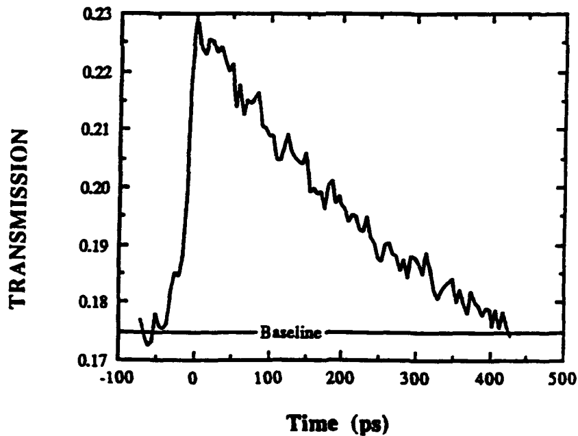
Figure 4.6 - Switching Recovery Time for a GaInAs Etalon.
