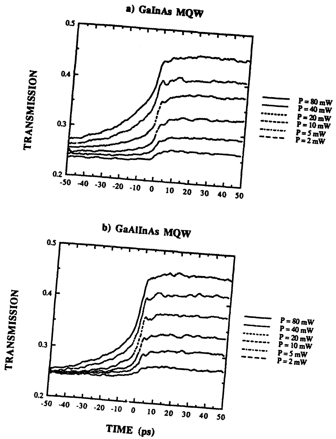
Figure 4.3 - Switching Characteristics for a) GaInAs and b) GaAlInAs MQWs.
