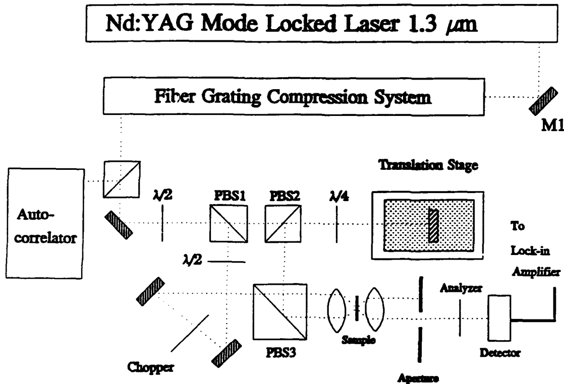
Figure 4.1 - Short Pulse Pump-Probe Experiment System.
