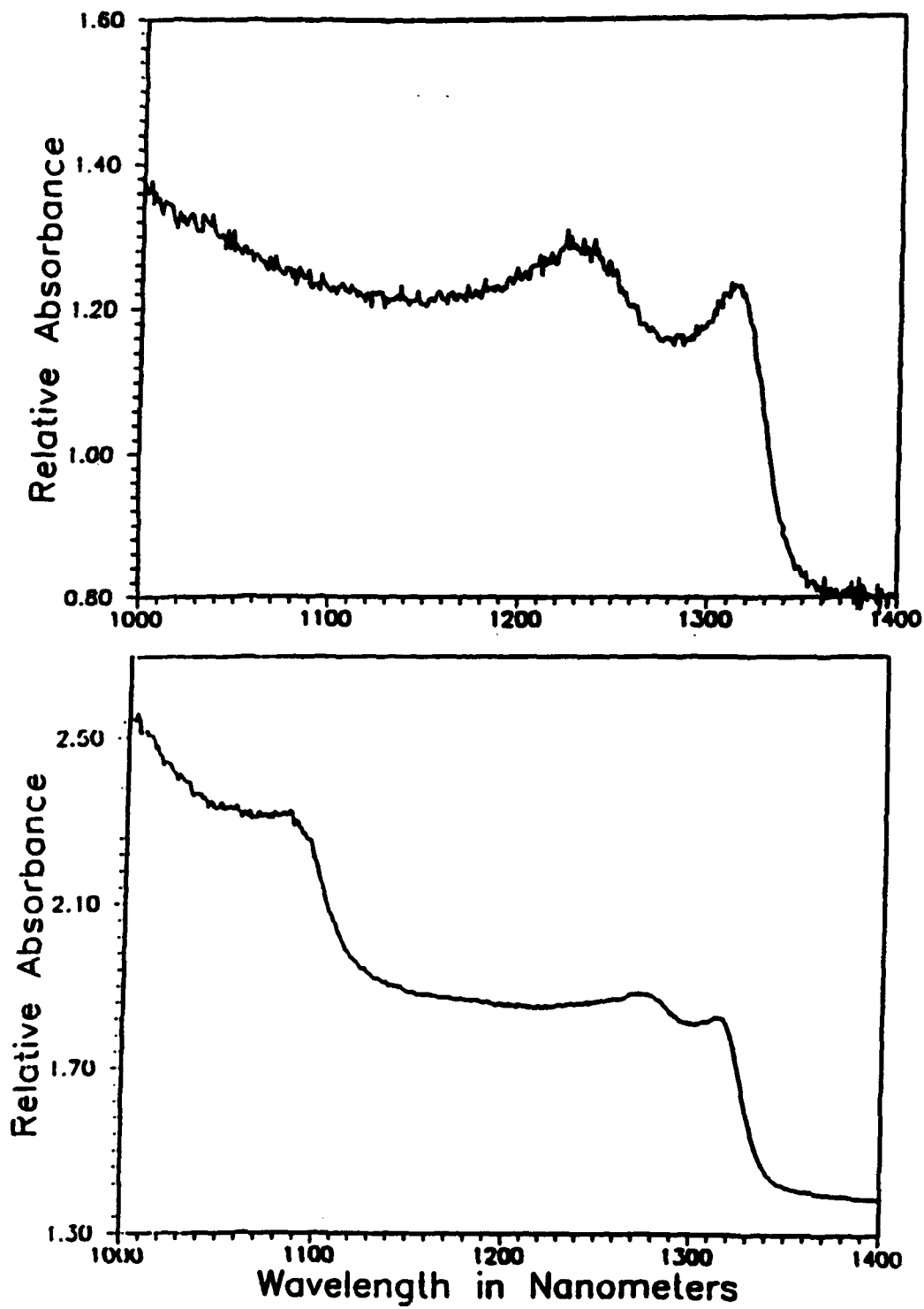
Figure 3.3 - White Light Absorption Spectrum for a) GaInAs and b) GaAlInAs MQWs.
