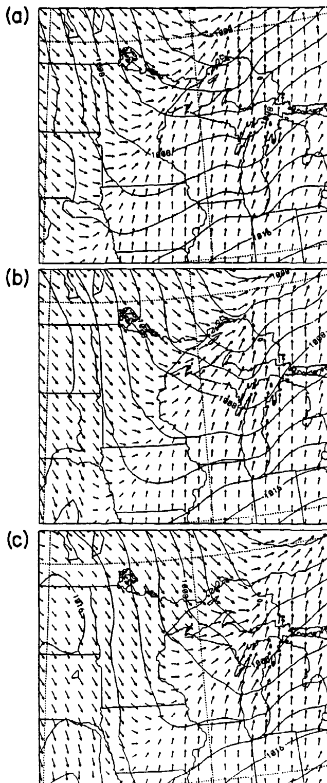
Figure 5.9: Sea level pressure and winds from the model 33km nested grid at (a) 1500 UTC, (b) 1800 UTC, (c) 2100 UTC.
