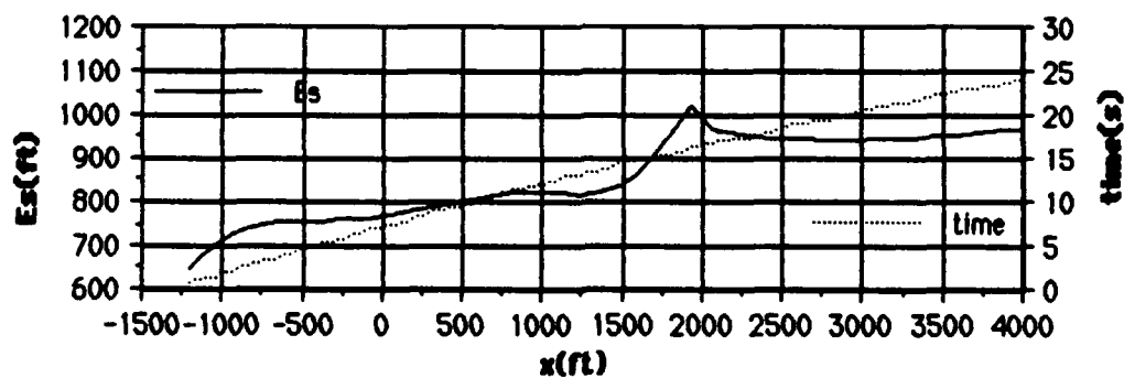
Figure G3. P-3 at 90,000lbs gross weight performing a constant 12 unit AOA maneuver during takeoff.
