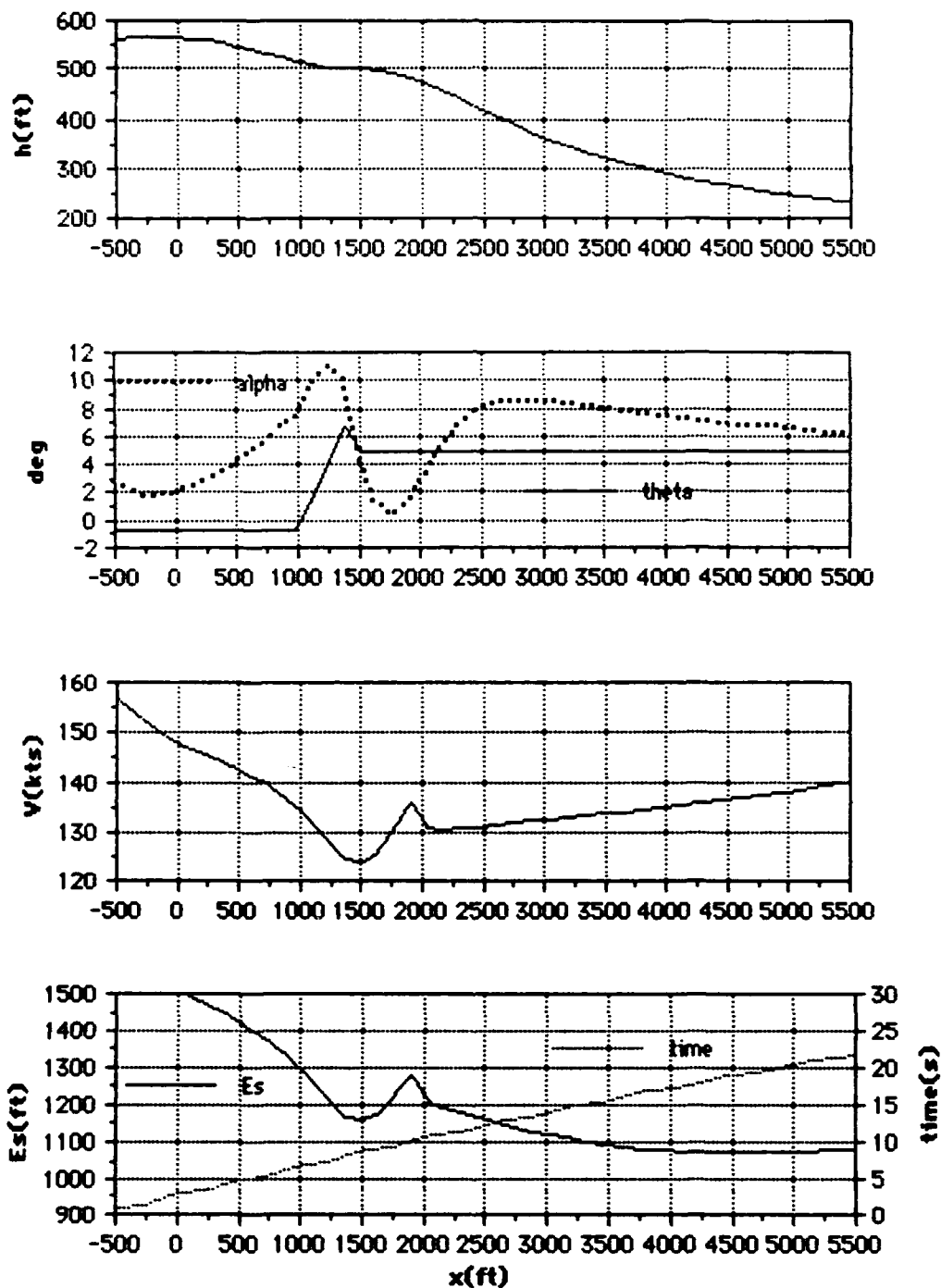
Figure F12. P-3 at 114,000lbs gross weight performing a constant 5° theta escape.
