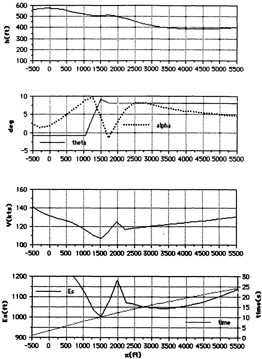
Figure F4. P-3 at 89,500lbs gross weight performing a constant 8° theta escape.
