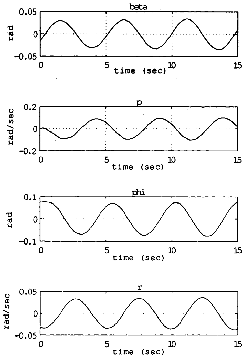
Figure 9. Dutch Roll Response at AOA = 10 degrees
