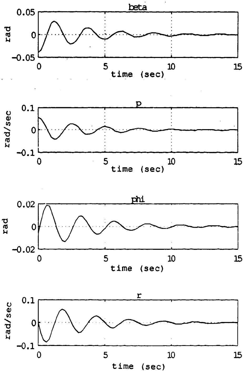
Figure 8. Dutch Roll Response at AOA = 0 degrees
