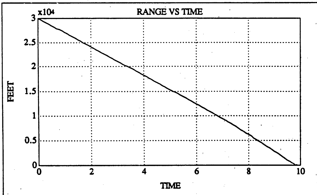
Figure 53. Scenario 3: Missile to Target Range
