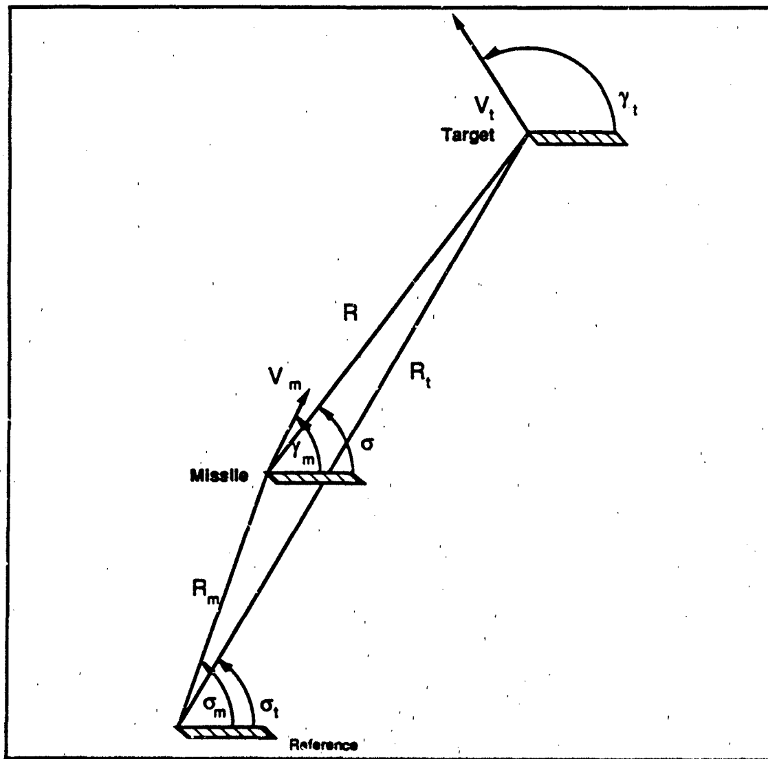
Figure 2. Missile/Target Geometry
