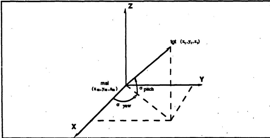
Figure 17. Pitch and Yaw Line of Sight Angle Definitions
