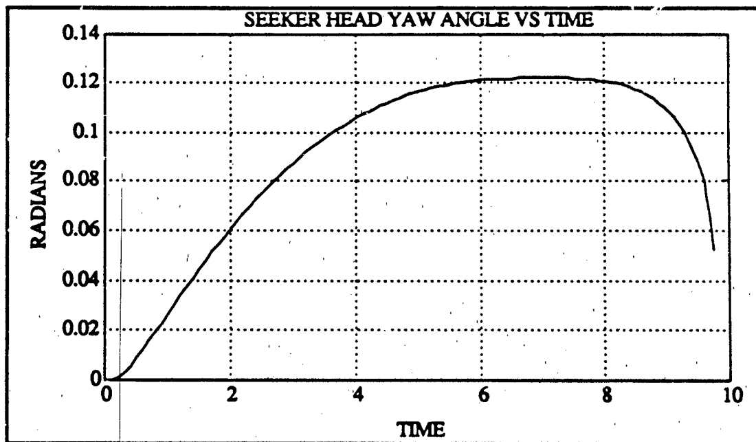
Figure 62. Scenario 3: Seeker Head Yaw Angle \beta_{yaw}
