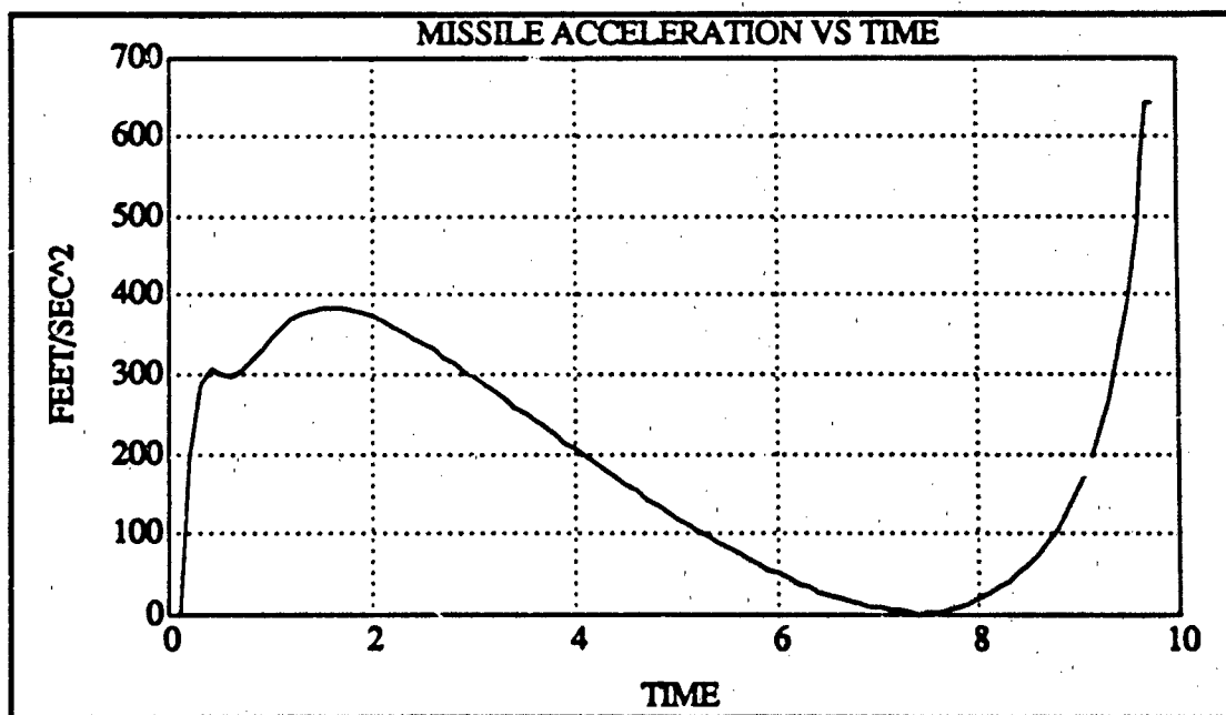
Figure 54. Scenario 3: Missile Acceleration |A_m|
