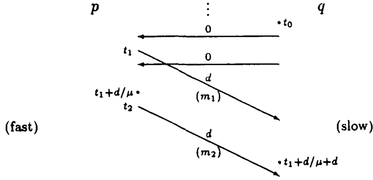
Figure 5.1: Execution \beta , the existence of which is proved by Lemma 5.1, takes the above form except that messages from p to q may be delayed more than d and messages may be sent by q at arbitrary times. The events of p ( q ) are on the left (right), with time represented by the vertical dimension. An arrow represents a message labelled with its delay, with its tail at the time of the send event and its tip at the time of the receive event.
