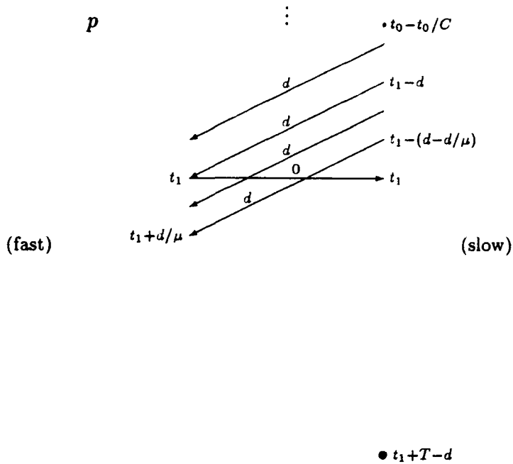
Figure 5.2: In the region of interest, execution \alpha' is simply \alpha with events of processor q occurring earlier in time by d . Because p fails at time t_1 , q detects the failure of p by time t_1 + T - d , denoted by the circle.
