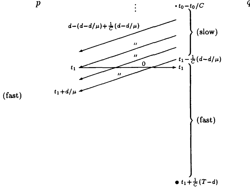
Figure 5.3: Execution \alpha'' is constructed from \alpha' by mapping the interval [t_1 - (d - d/\mu), t_1 + (T - d)] of \alpha' to the interval [t_1 - \frac{1}{C}(d - d/\mu), t_1 + \frac{1}{C}(T - d)] of \alpha'' and appropriately shifting the rest of q 's events.
