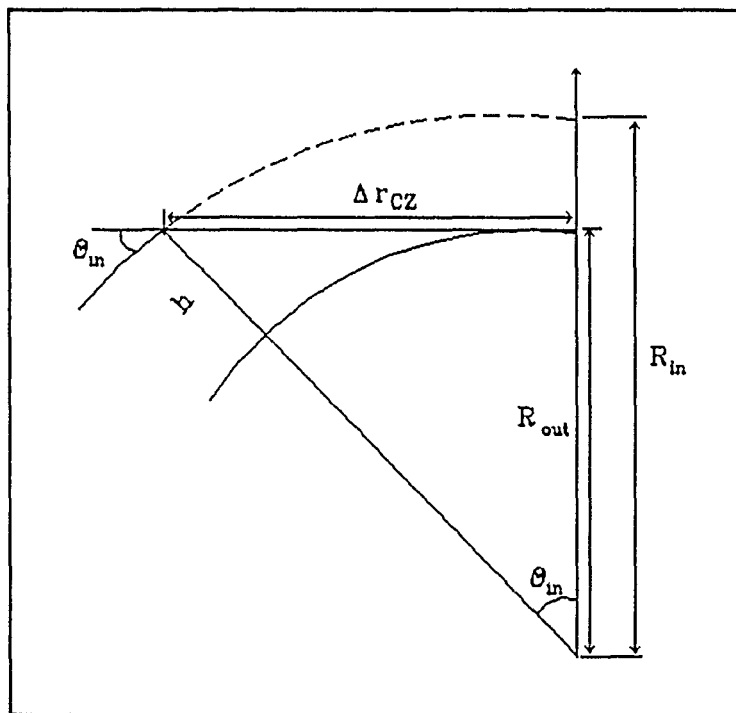
Figure 4 - CZ reference area (cross section)
