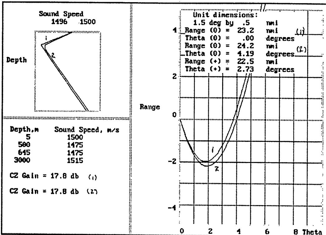
Figure 7 - CZGAIN Display Depiction
