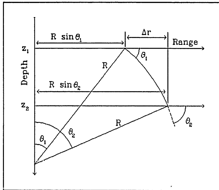
Figure 1 - Horizontal Distances
