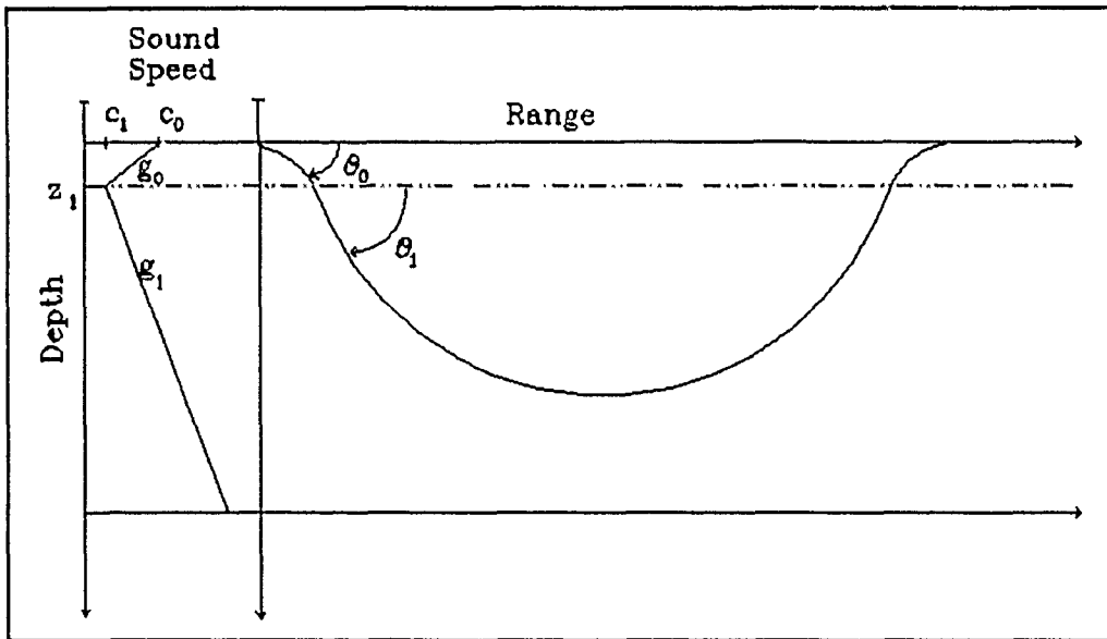
Figure 5 - Reference diagram for subscript conventions.
