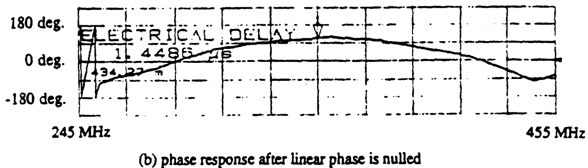
Figure 4.8: Phase response after the optical window is inserted into the Presort Processor
