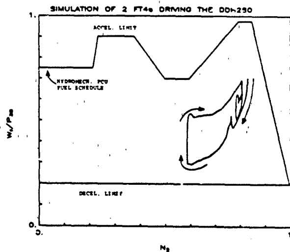
Figure 12: W_t/P_{3s} vs N_2 Transient for Ship Crashback with ECM
