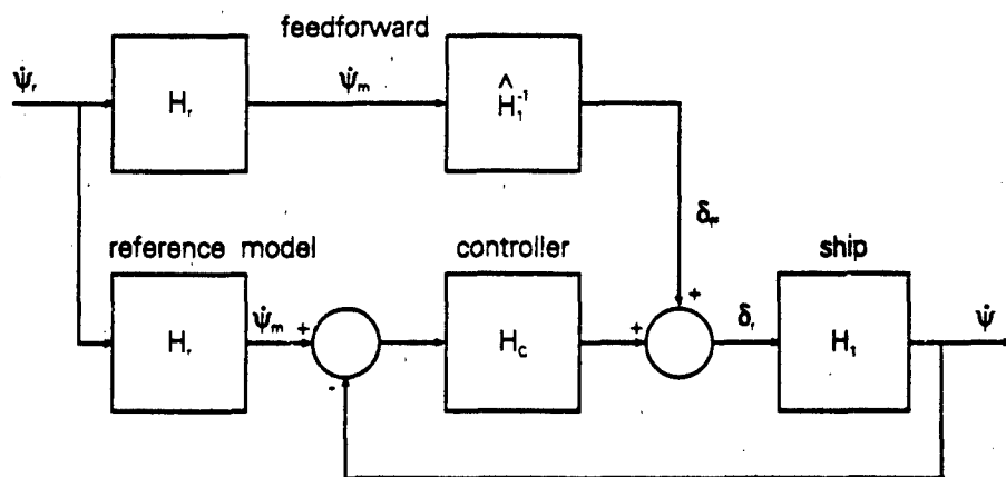
Figure 4. Rate-of-Turn Control Loop
