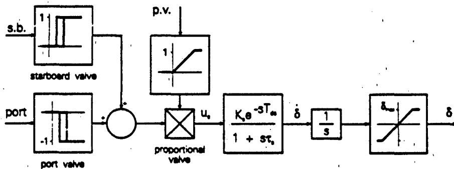
Figure 2. Steering Machine
