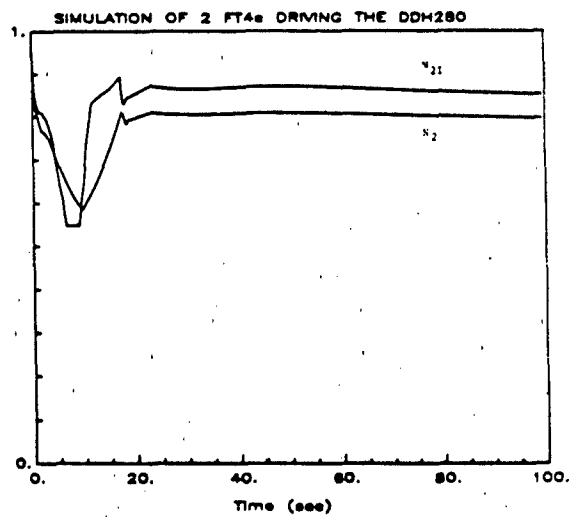
Figure 10: Engine Performance for Ship Crashback with ECM
