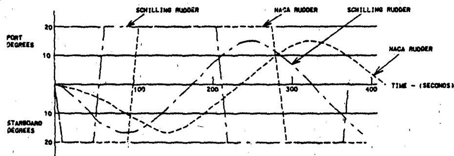
Figure 8. Slow Steaming Ability - 6 Knot Zigzag Manoeuvre Model Test for 175 M Twin Screw Ferry (Vienna Model Basin) 20°/10° Zigzag Test
