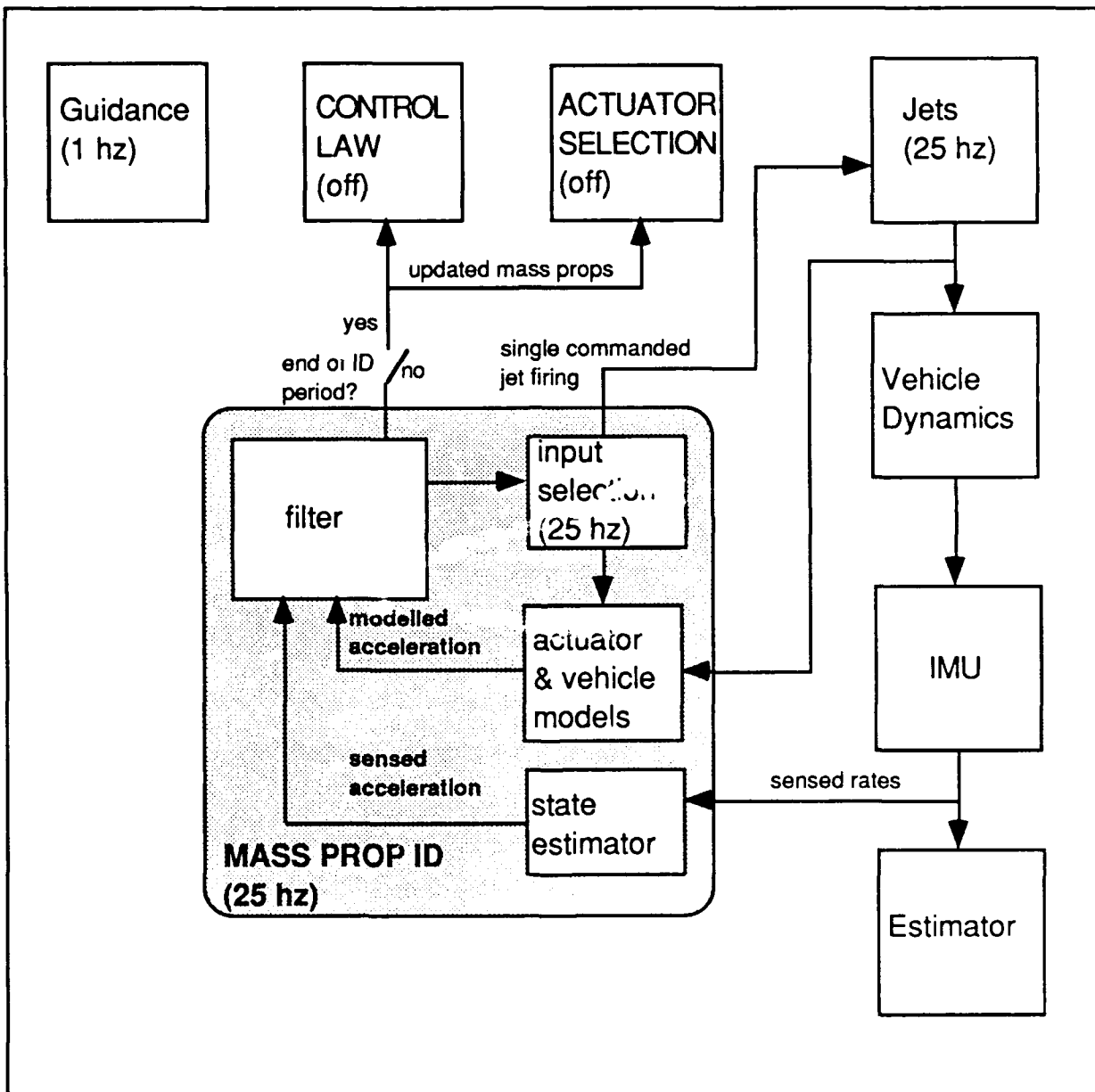
Figure 6.4. Dedicated Mass Property Identification Period (First 0.5 sec)
