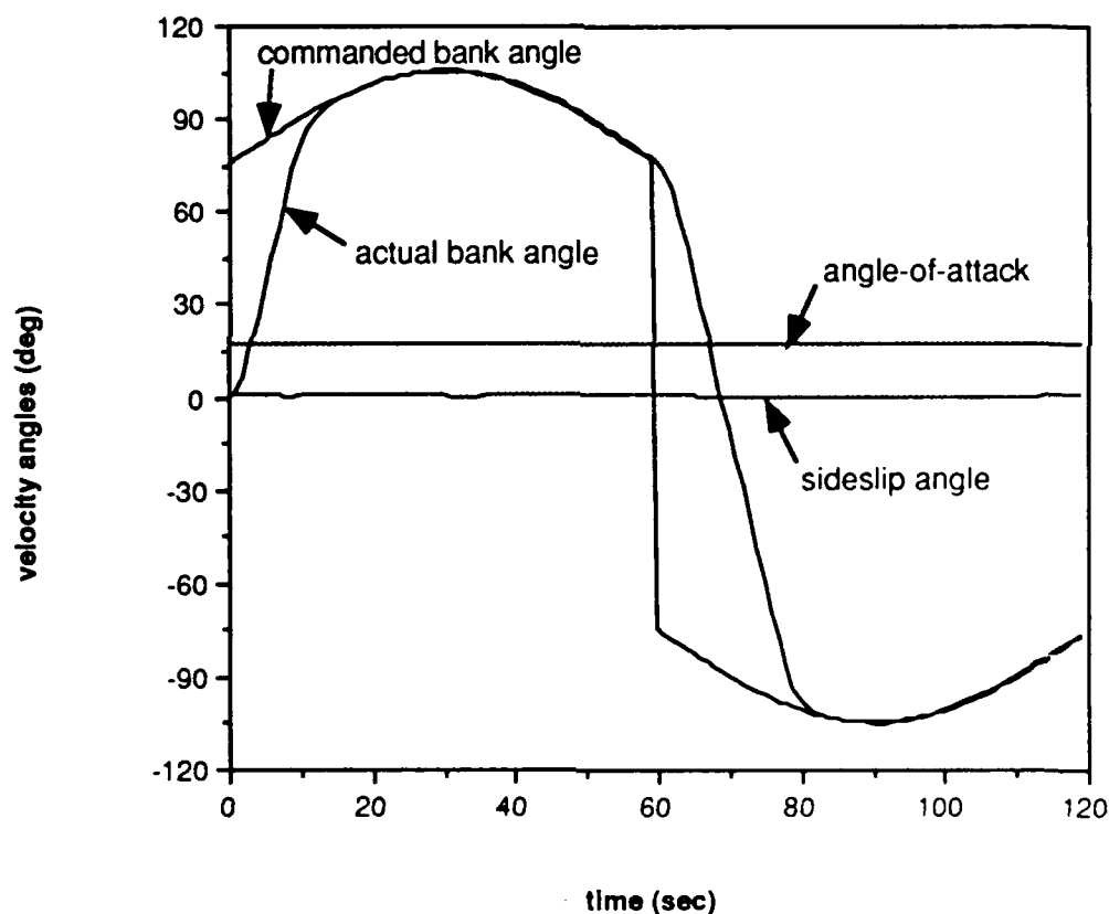
Figure 7.4. Velocity Angle Response - New Design (Nominal Mass Properties)
