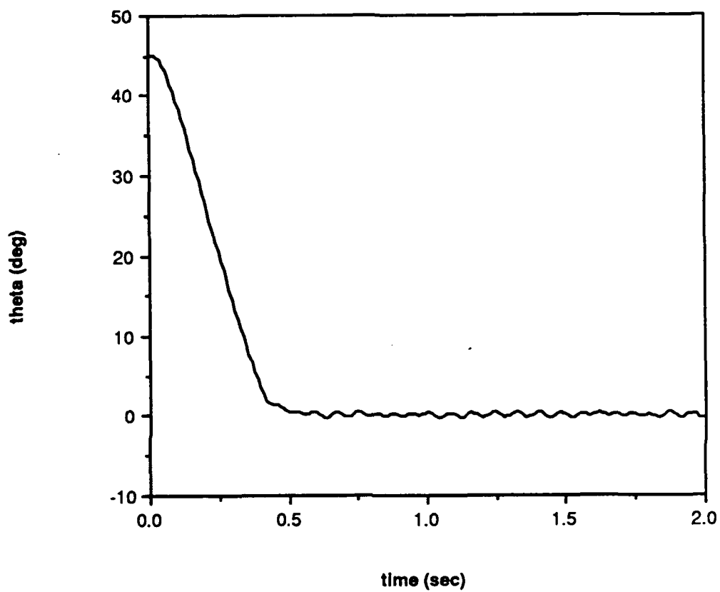
Figure 3.6. Pendulum Trajectory with \theta_d = 0 (Switching Control Law)
