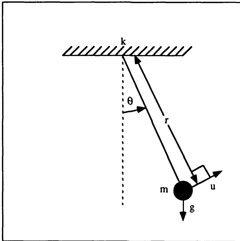
Figure 3.2. Controlled Pendulum
