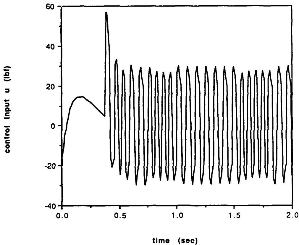
Figure 3.9. Control Activity (Switching Control Law)
