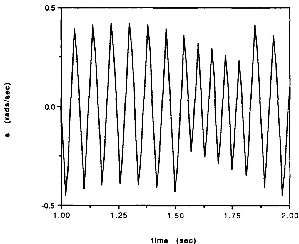
Figure 3.8. Sliding Variable vs. Time (Expanded View)
