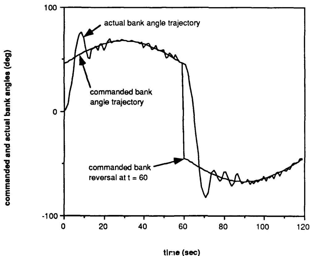
Figure 6.1. Bank Angle Tracking (\lambda_i = 5.0, \eta_i = 1.0)
