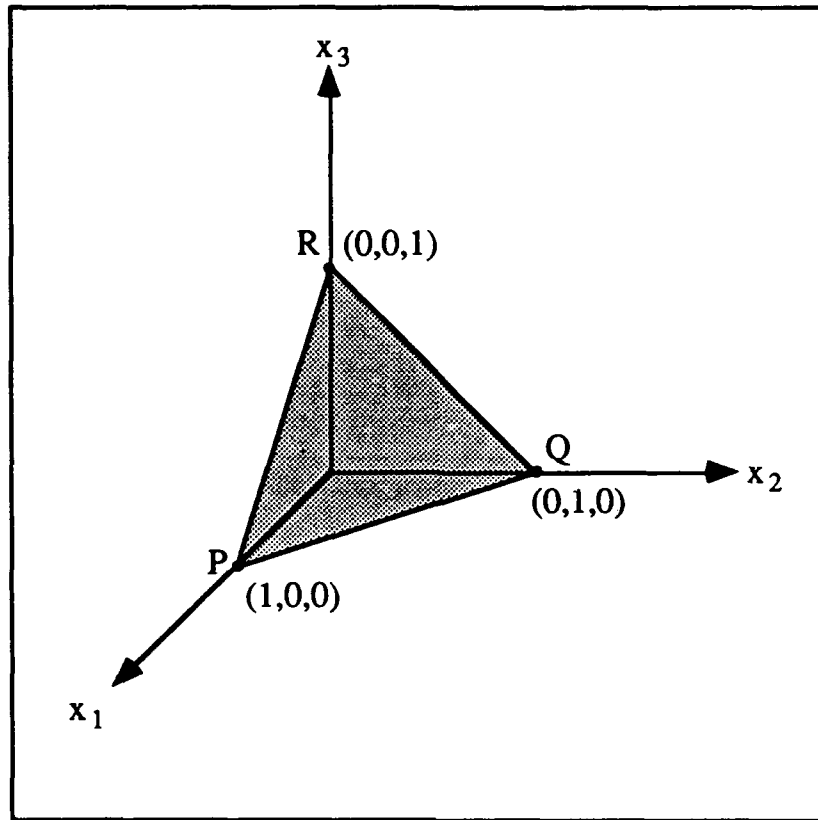
Figure 4.3. 3-D Feasible Set for Example Problem
