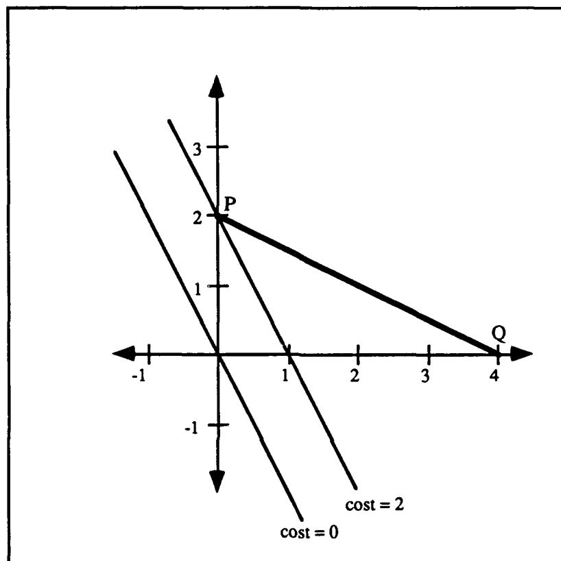
Figure 4.2. Feasible Set and Cost Curves
