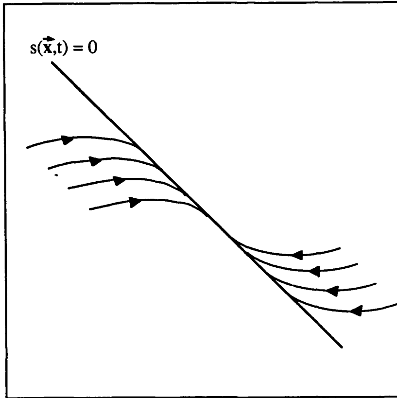
Figure 3.4. Attractive Sliding Surface
