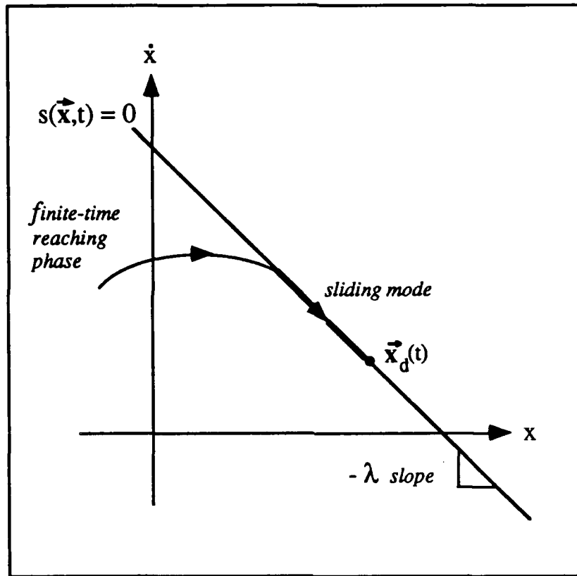
Figure 3.5. Typical State Trajectory
