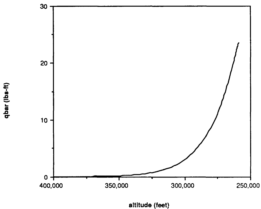
Figure B.1. Dynamic Pressure vs. Altitude
