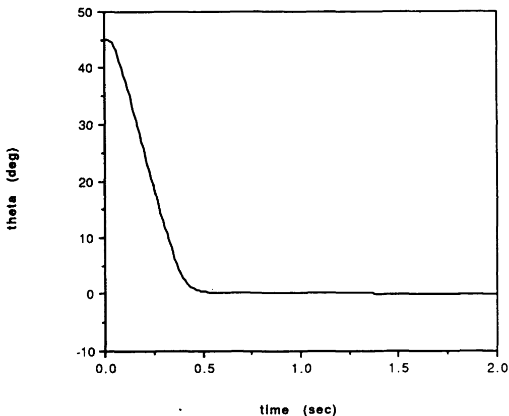
Figure 3.11. Pendulum Trajectory with \theta_d = 0 (Continuous Control Law)
