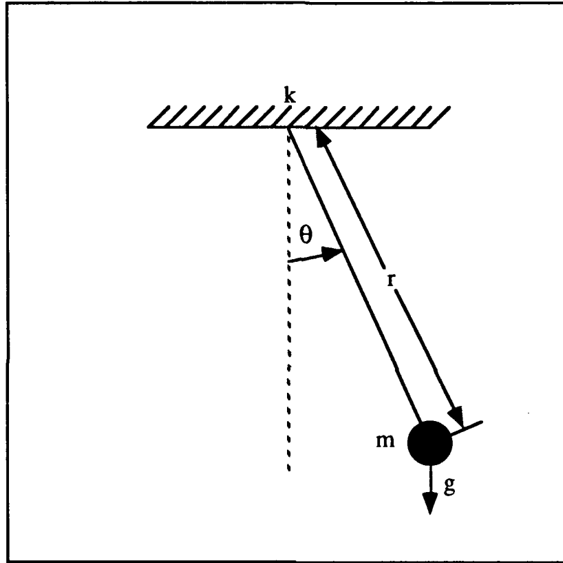
Figure 3.1. Simple Pendulum
