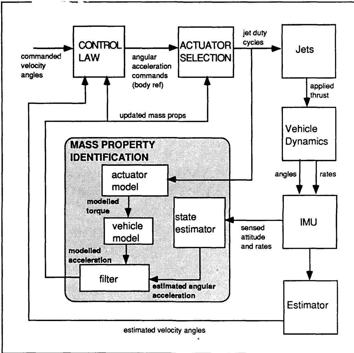
Figure 2.1. Aerocapture Control System Structure
