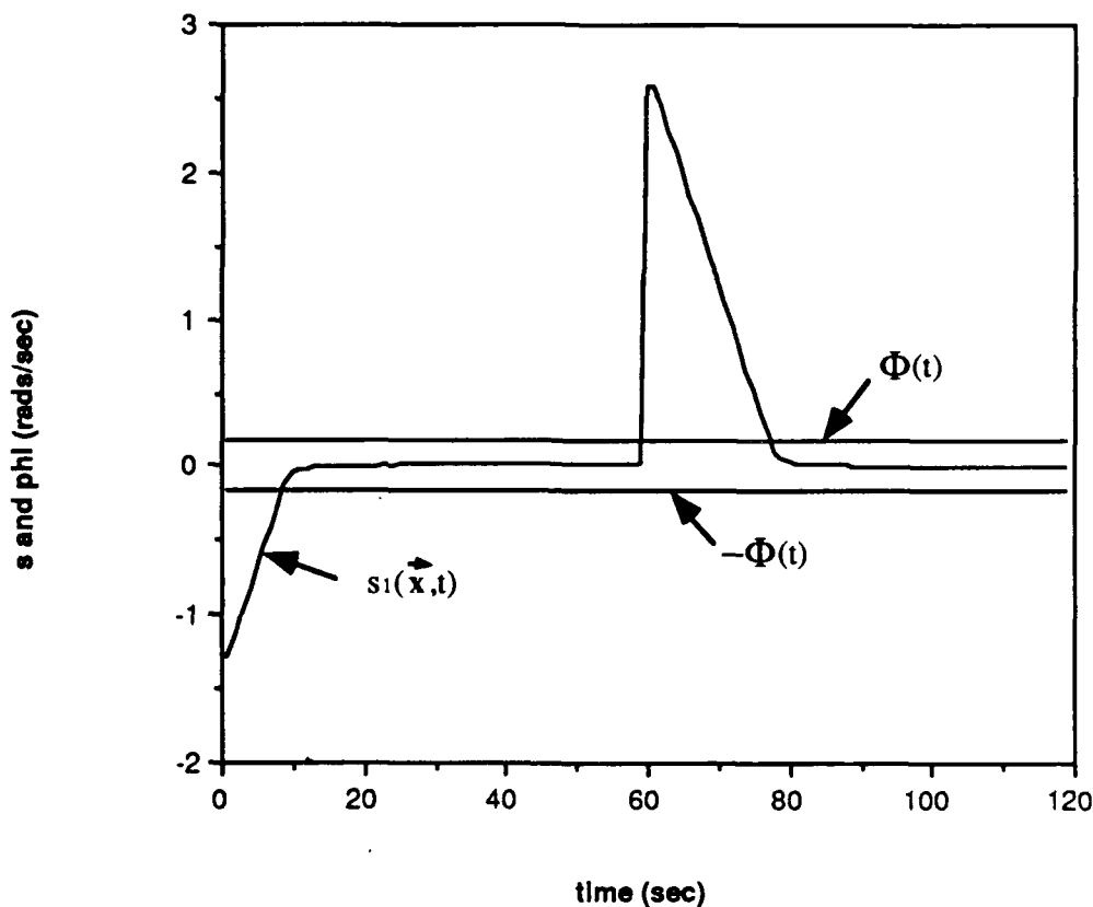
Figure 7.5. Sliding Variable and Boundary Layer (Nominal Mass Properties)
