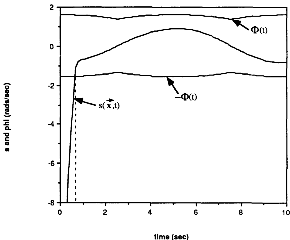
Figure 3.16. Sliding Variable and Boundary Layer vs. Time
