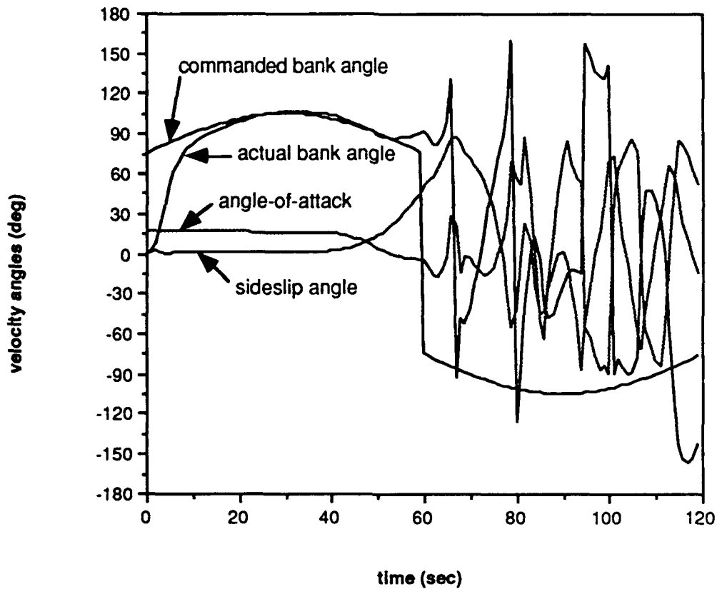
Figure 7.8. Velocity Angle Response - AFE DAP (Large Step Changes in Mass Properties)
