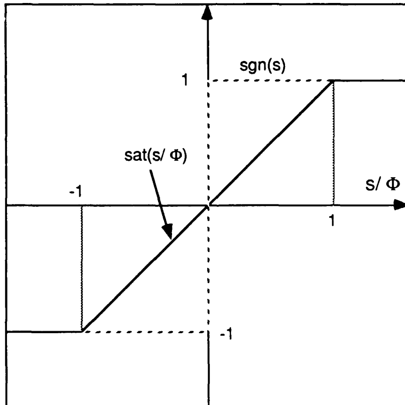
Figure 3.10. Saturation Function, \text{sat}(s/\Phi)
