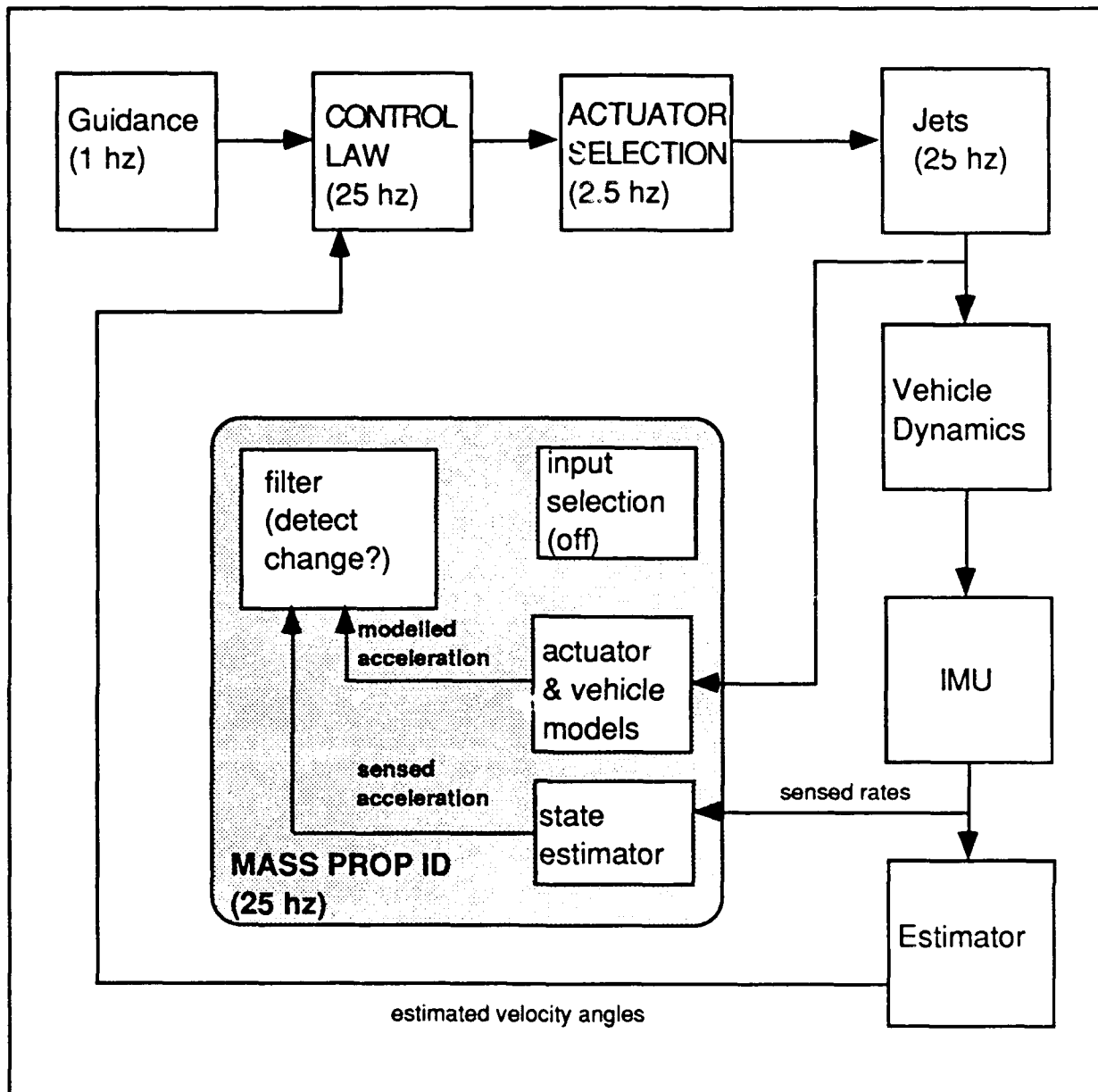
Figure 6.5. Normal Control System Operation
