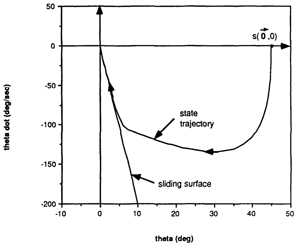
Figure 3.14. State Trajectory in Phase Plane (Continuous Control Law)
