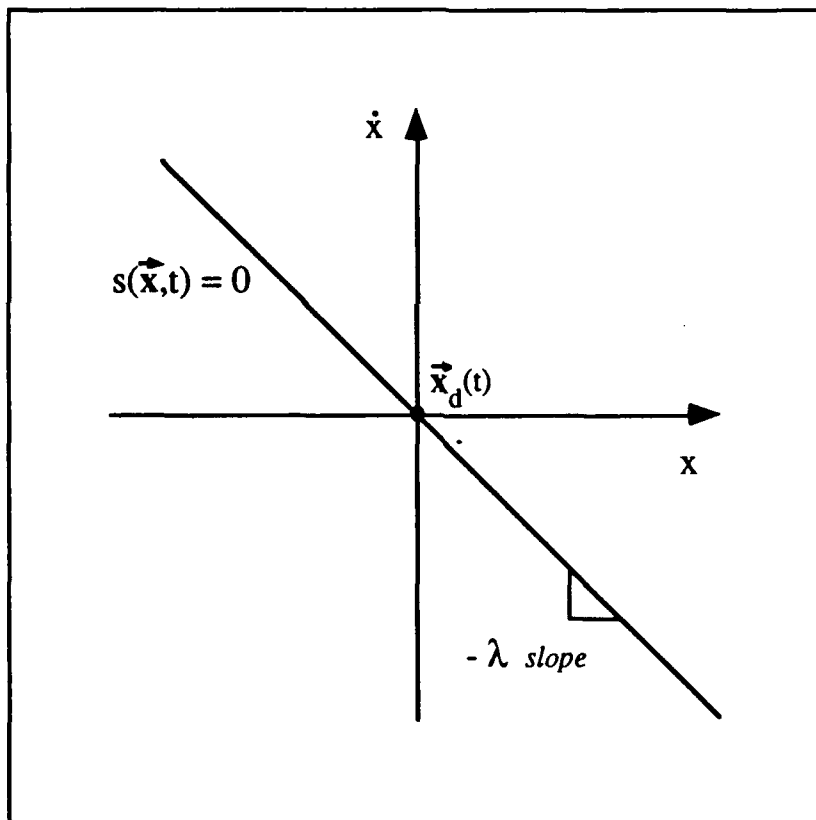
Figure 3.3. Sliding Surface Through Origin
