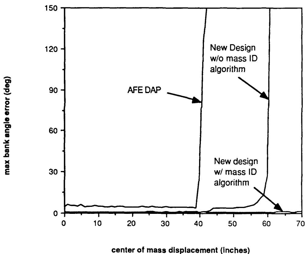
Figure 7.3. Max Bank Angle Error vs. Center of Mass Displacement
