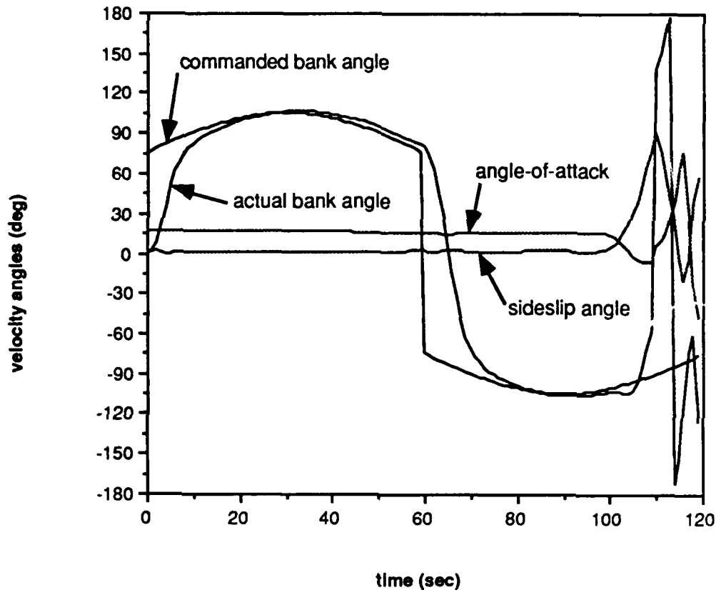
Figure 7.10. Velocity Angle Response - AFE DAP (Slow, Continual Mass Property Changes)
