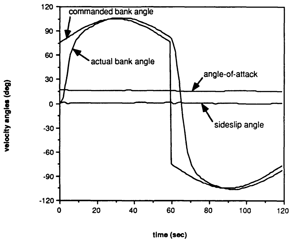
Figure 7.6. Velocity Angle Response - AFE DAP (Nominal Mass Properties)
