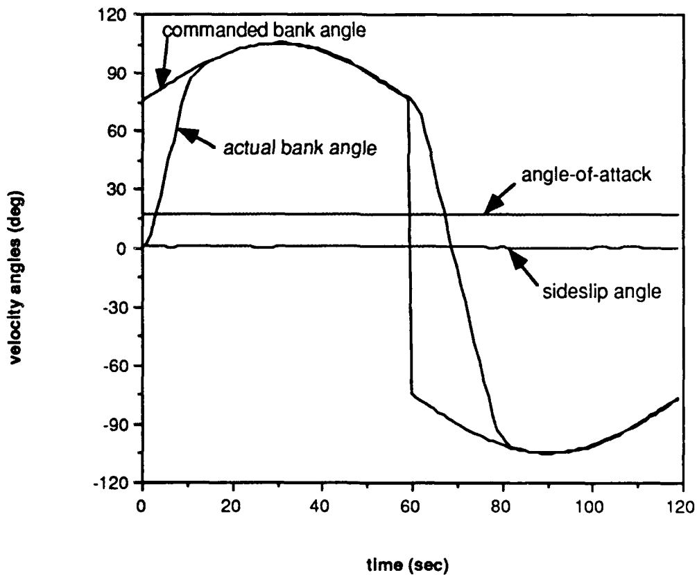
Figure 7.9. Velocity Angle Response - New Design (Slow, Continual Mass Property Changes)
