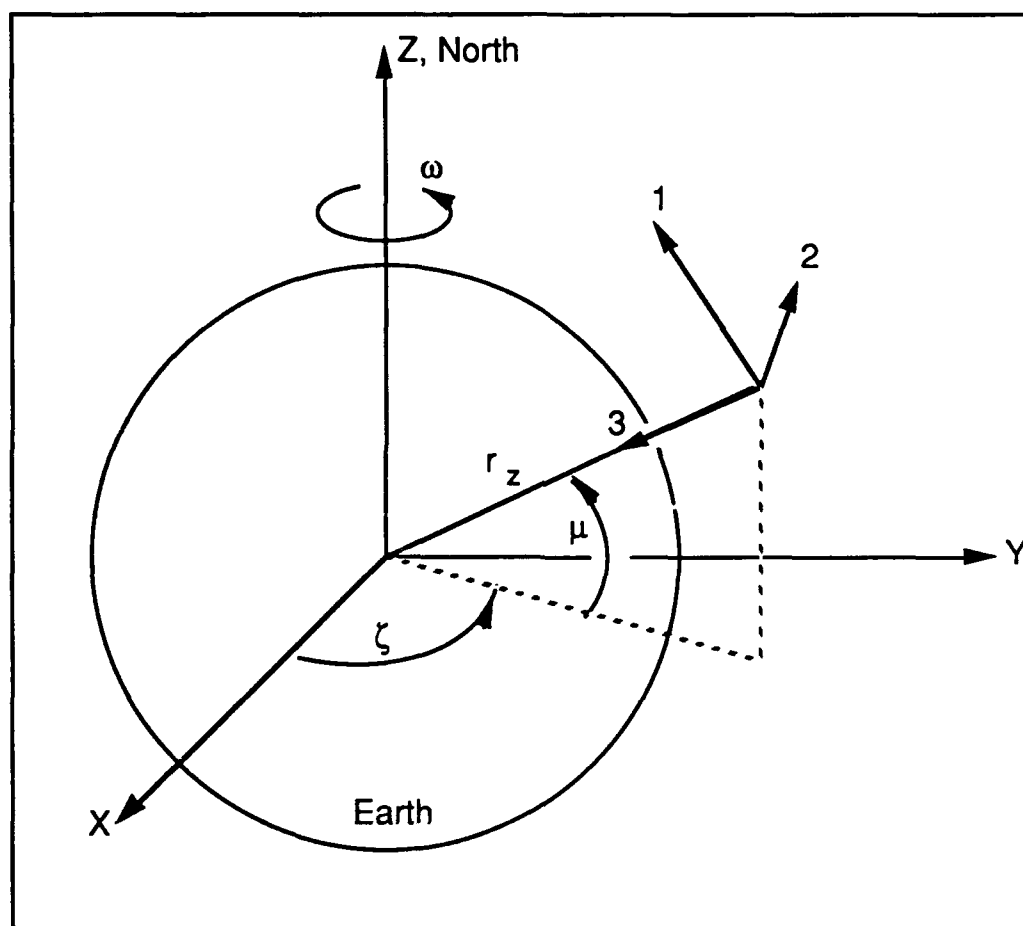
Figure A.1 123 Reference System
