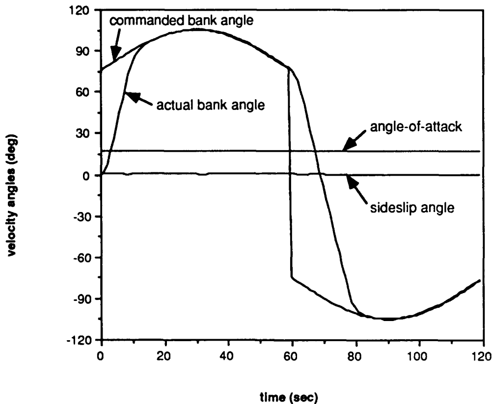
Figure 7.7. Velocity Angle Response - New Design (Large Step Changes in Mass Properties)
