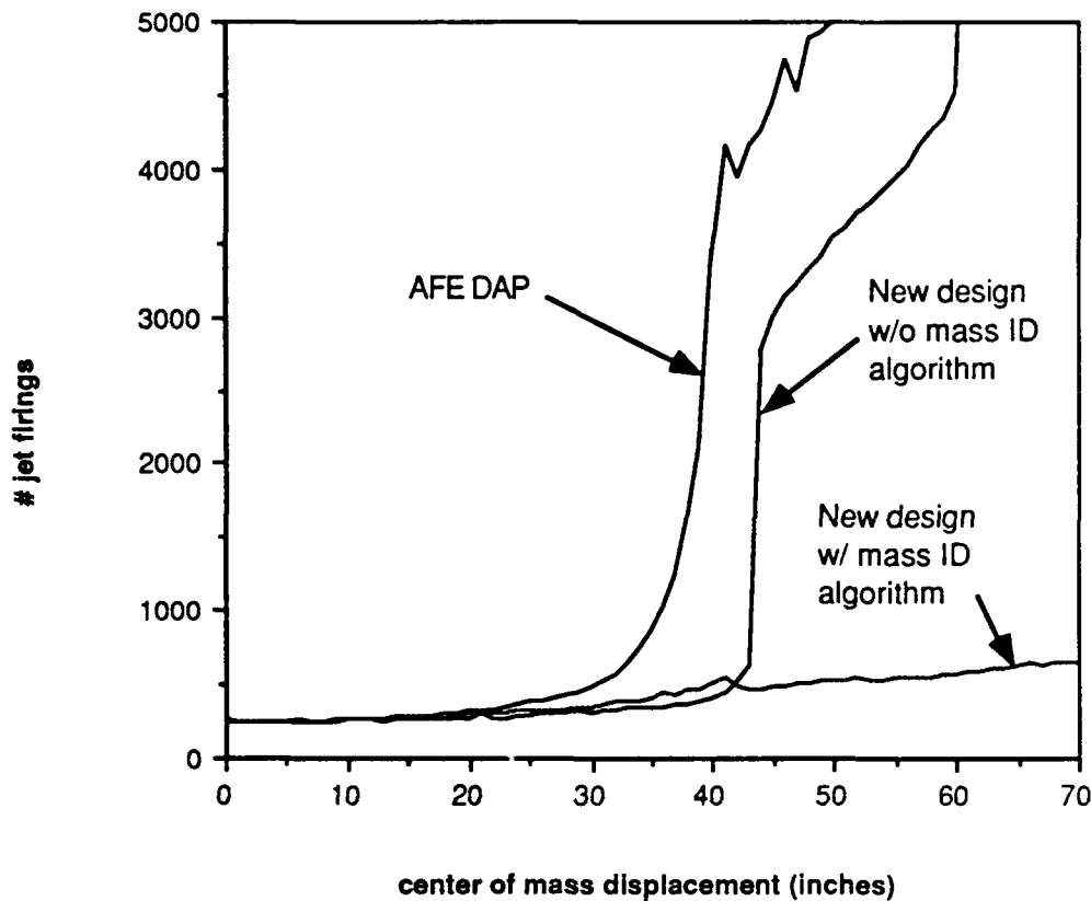
Figure 7.2. Jet Firings vs. Center of Mass Displacement
