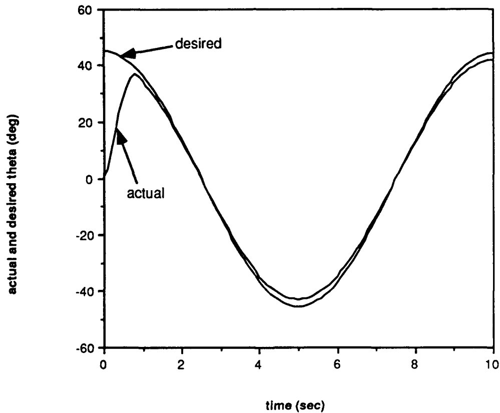
Figure 3.15. Pendulum Trajectory with Varying \theta_d (Continuous Control Law)
