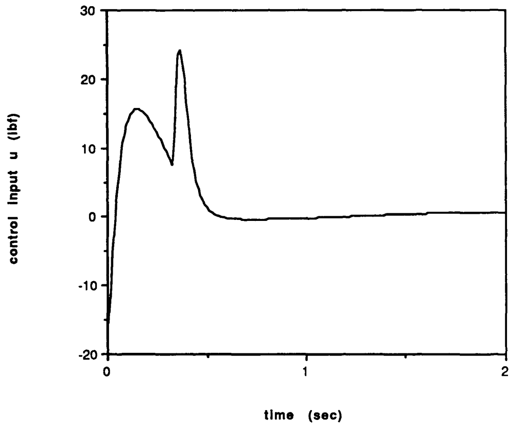
Figure 3.13. Control Activity (Continuous Control Law)
