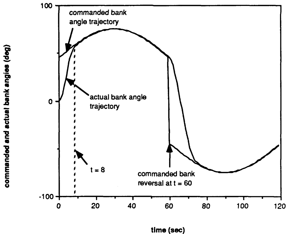
Figure 6.2. Bank Angle Tracking (\lambda_i = 1.0, \eta_i = 0.1)
