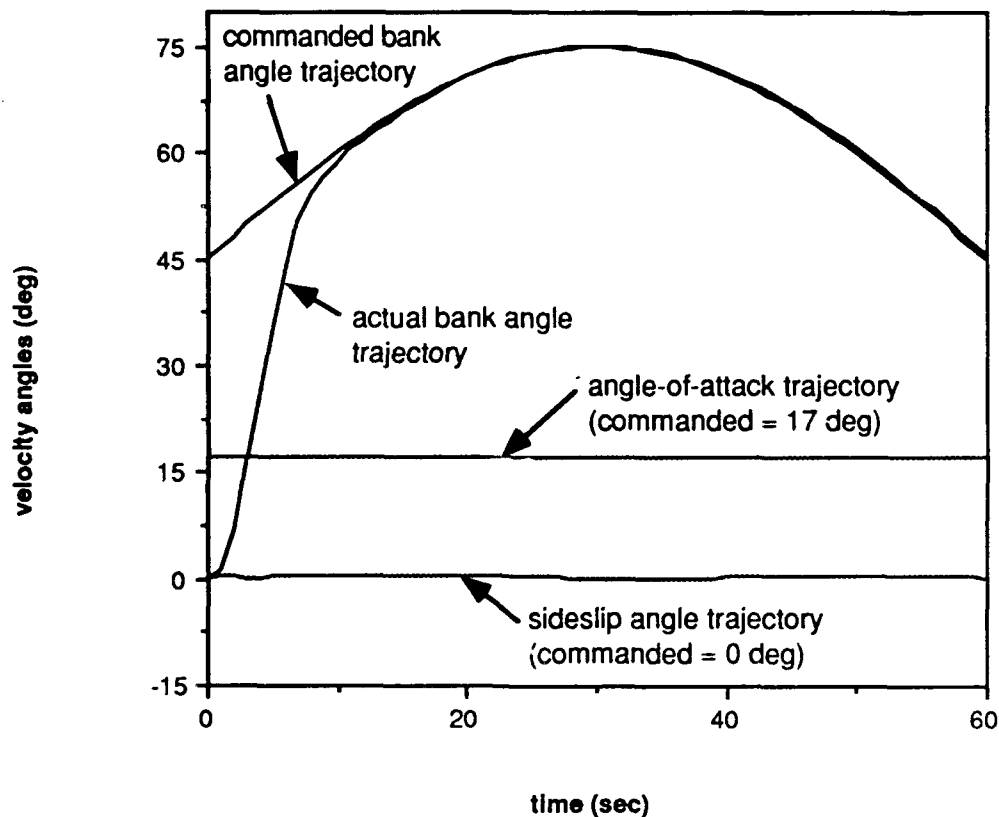
Figure 7.1. Velocity Angle Response of Typical 60 Sec Simulation
