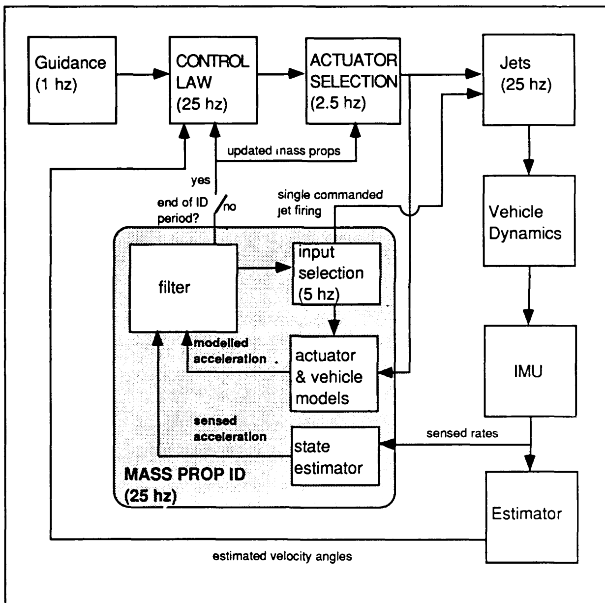
Figure 6.6. Operation After Detection of Mass Property Change
