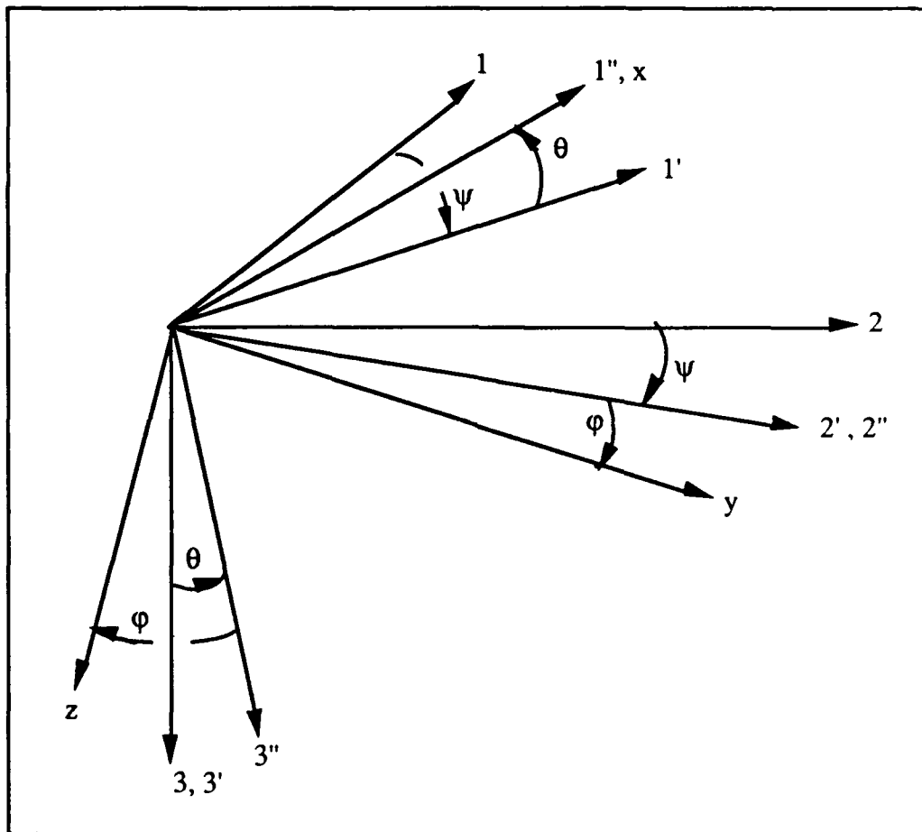
Figure A.2. Euler Angles
