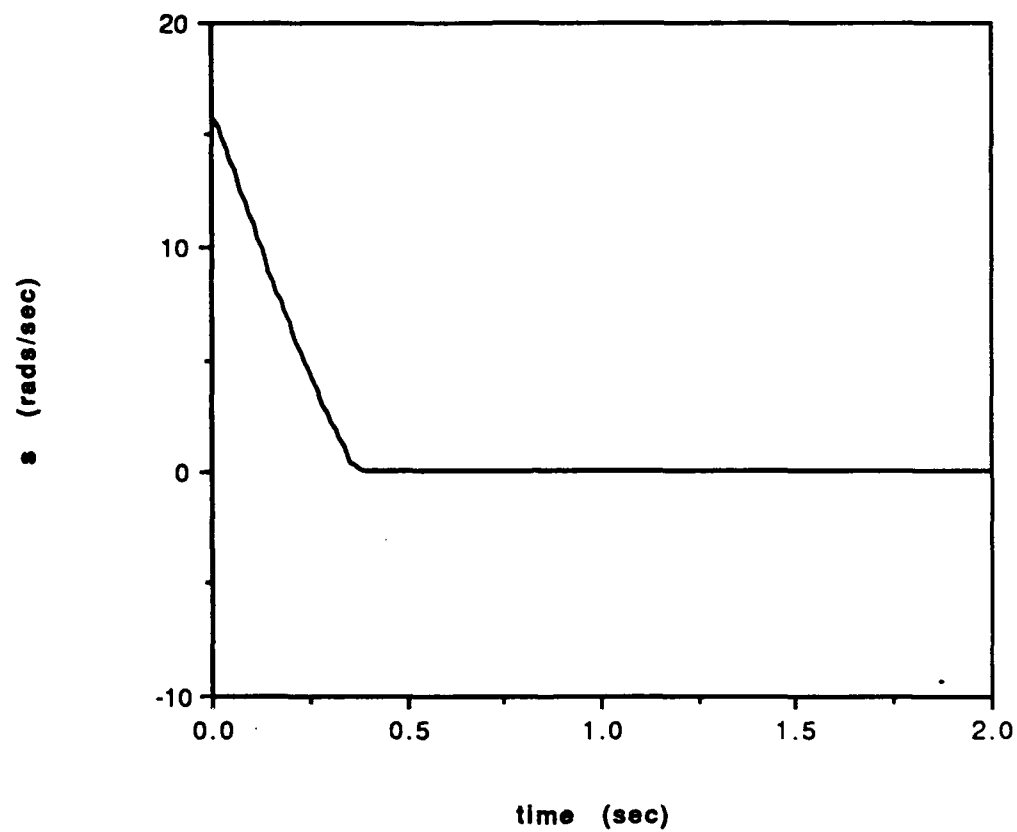
Figure 3.12. Sliding Variable vs. Time (Continuous Control Law)
