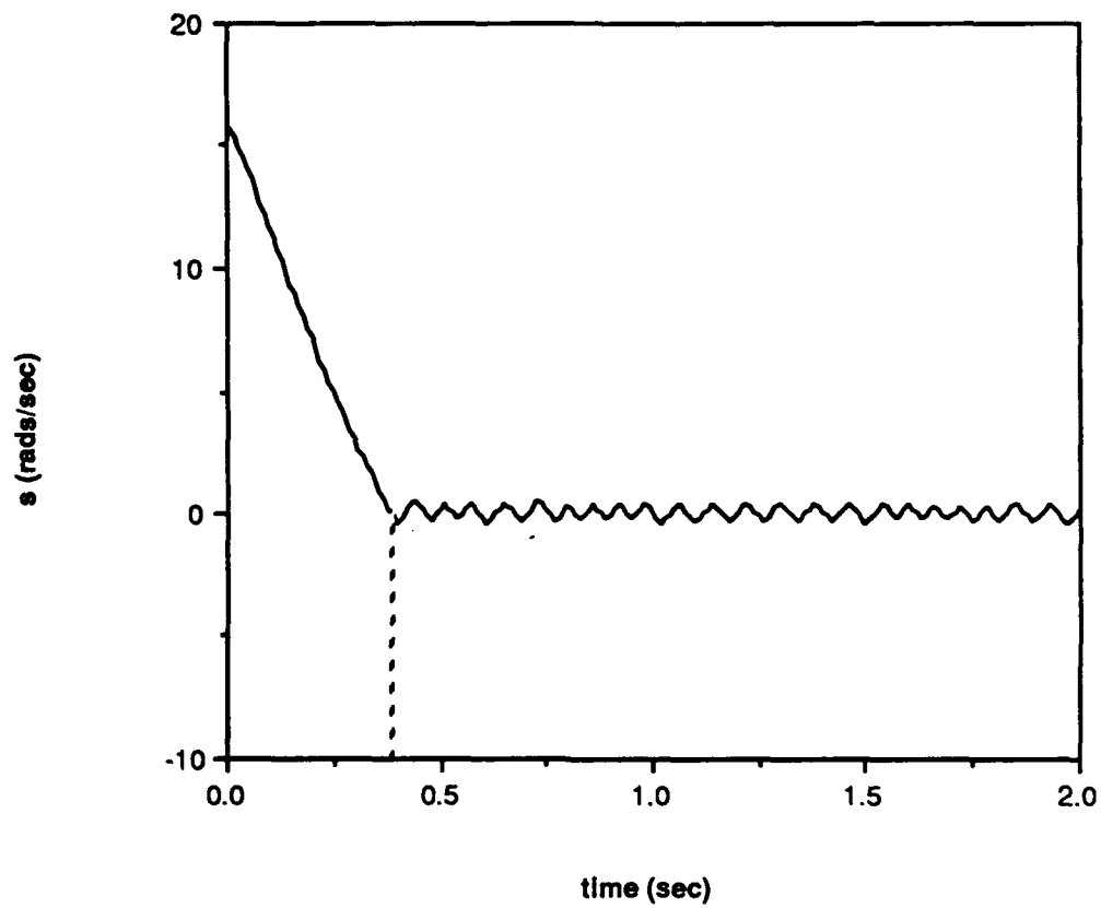
Figure 3.7. Sliding Variable vs. Time (Switching Control Law)
