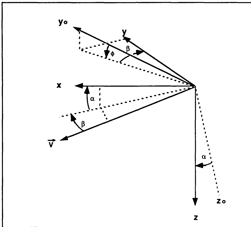
Figure A.3. Velocity Angles
