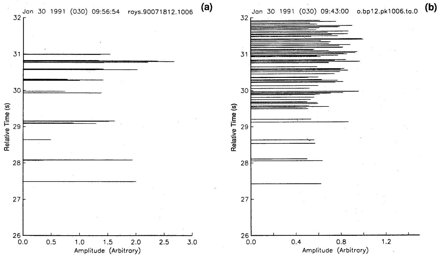
Figure 16. (a) predicted arrival times and (b) measured arrival pattern for path 1006 on day 199. All times are relative.
