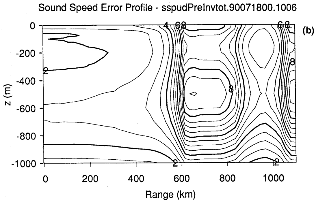
Figure 24. Sound speed error section (a) from OTIS and (b) after increasing the errors.
