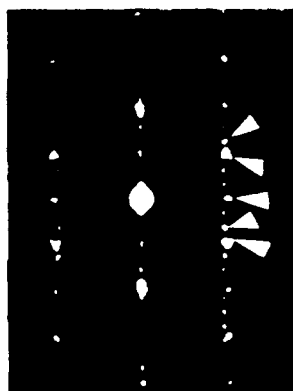
Figure 9. Selected area diffraction patterns of annealed (700°C for 20 min.) Ti/SiC interface region in cross-section. Ti deposited on (0001) 6H-SiC at room temperature. z = [11\bar{2}0] SiC = [11\bar{2}0] Ti = [45\bar{1}0] \text{Ti}_5\text{Si}_3 = [011] TiC "1" = \text{Ti}_5\text{Si}_3 "2" = TiC.
