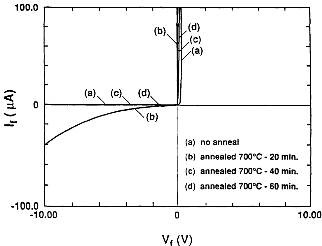
Figure 1. Current-voltage characteristics of Ti deposited on (0001) 6H-SiC epitaxial layer. ( 2.0 \times 10^{-3} \text{ cm}^2 contact area).
