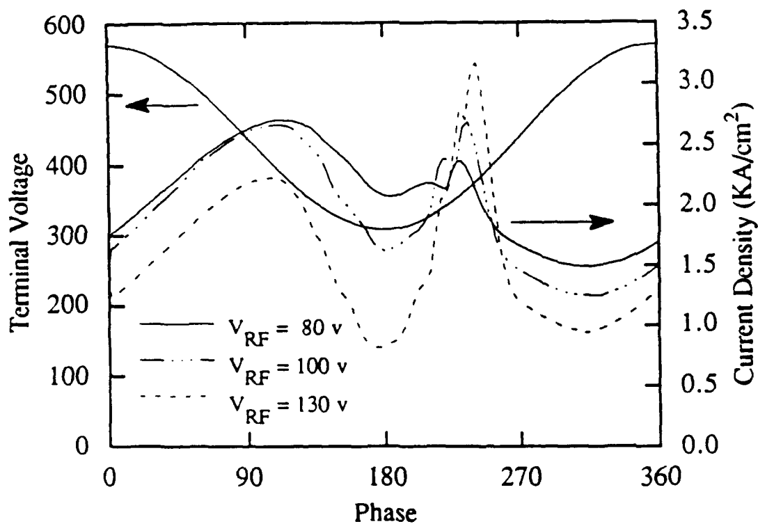
Figure 4. The terminal current vs. phase for a 44 GHz SiC IMPATT for RF voltages of 80, 100, and 130 volts. The terminal voltage waveform for 80 volts is included.
