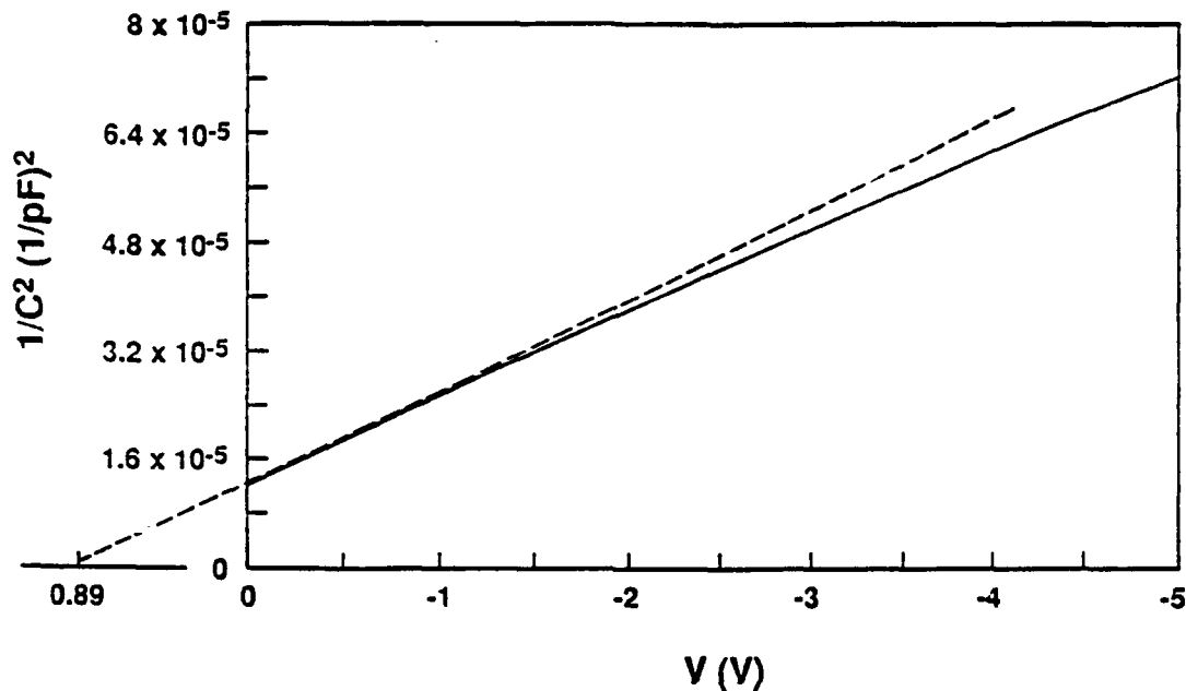
Figure 14. Differential capacitance-voltage measurements for as-deposited Pt/SiC plotted as 1/C^2 vs. V . \Phi_B \cong 1.02 \text{ V} .
