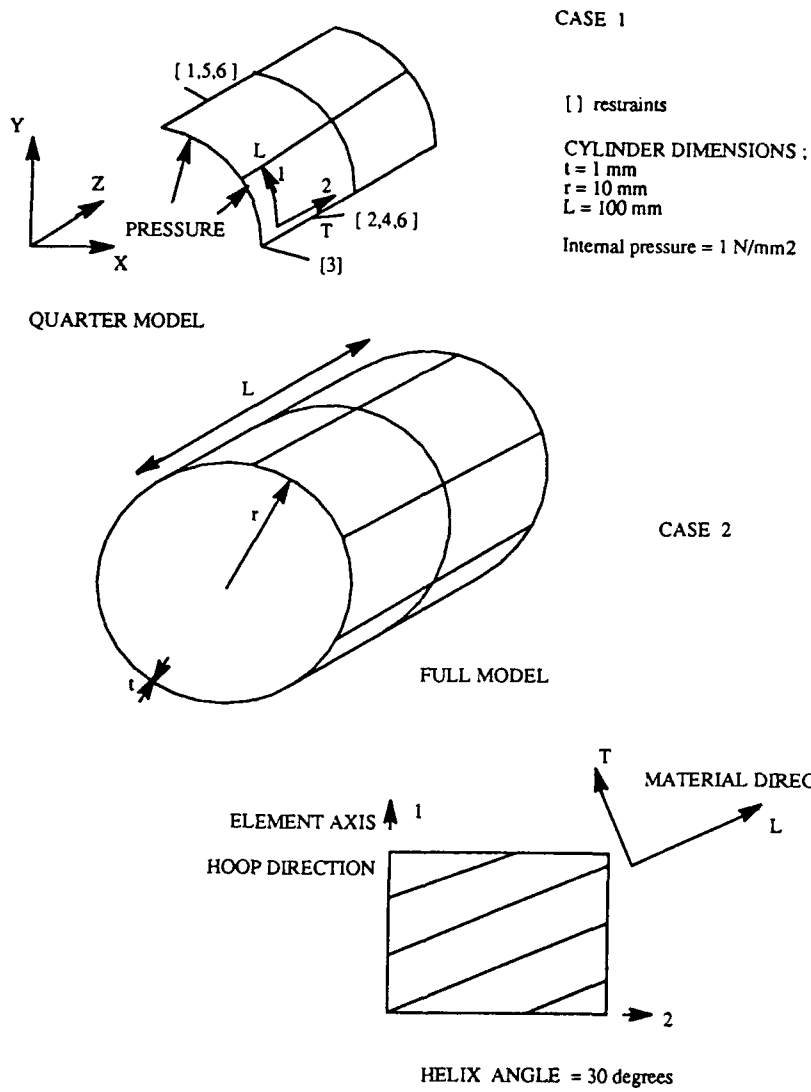
EXAMPLE A MEMBRANE RESPONSE OF COMPOSITE CYLINDERS FIGURE 2
