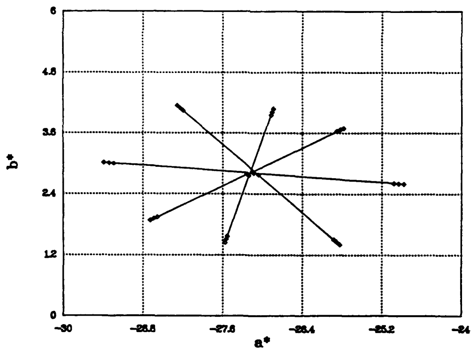
FIGURE 15. Green Color Center Vector Tolerances
