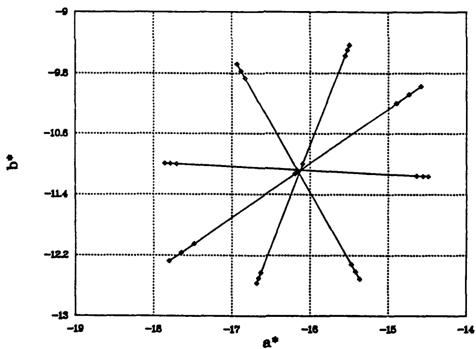
FIGURE 13. Cyan Color Center Vector Tolerances
