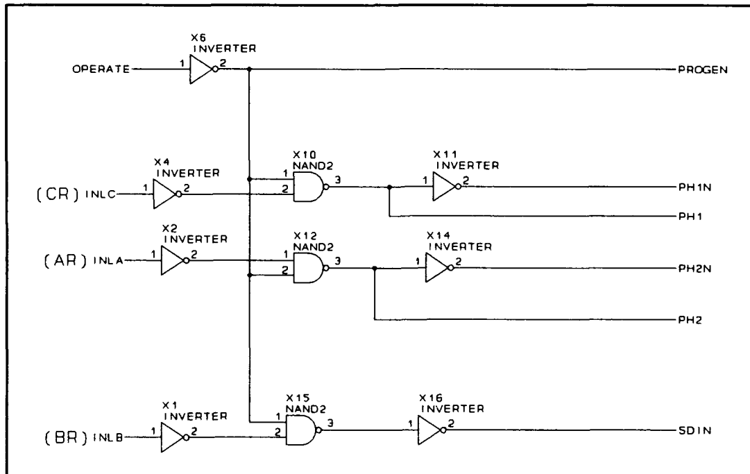
Figure 10. Operate/Program Select Logic.
