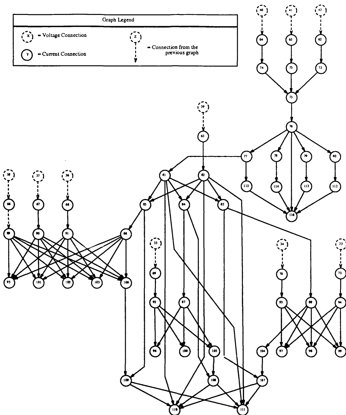
Figure 12. Connections Dependency Graph - Part 2 (Load)
