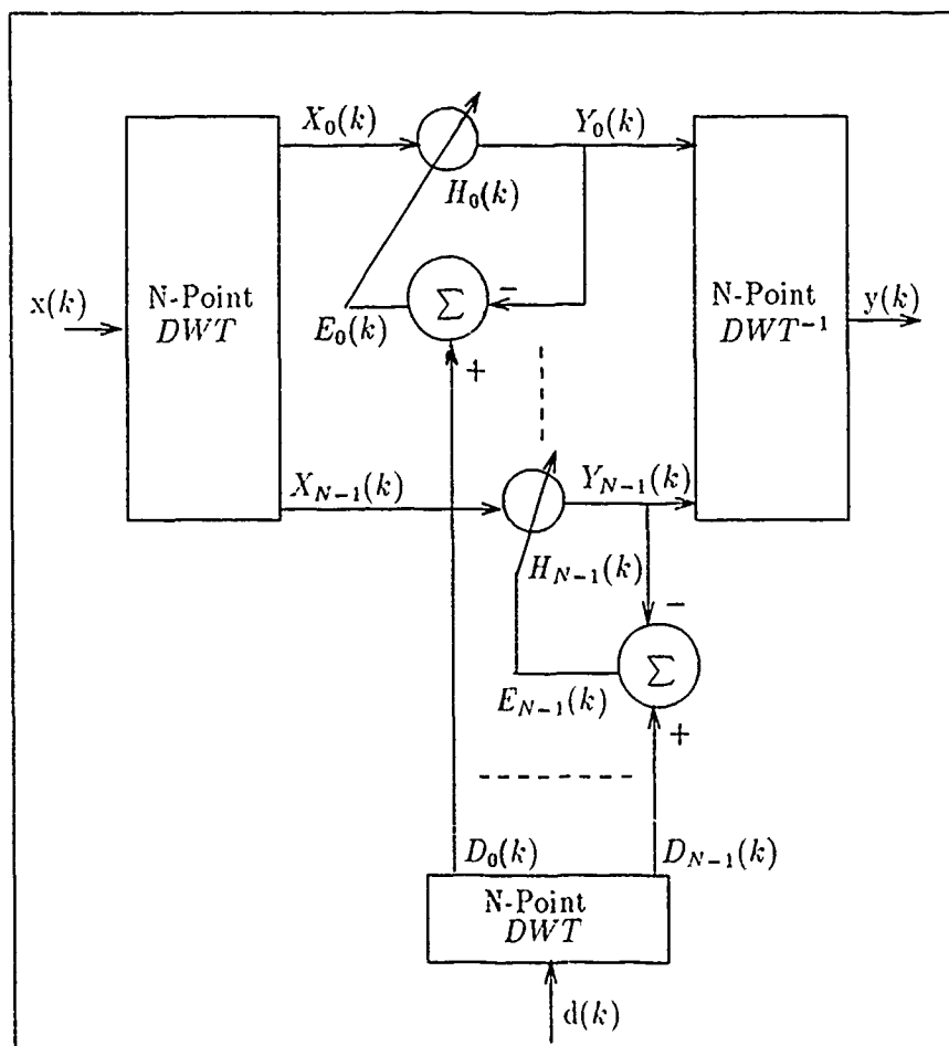
Figure 3.1. Walsh-domain Adaptive Filter 1 (WDF1)
