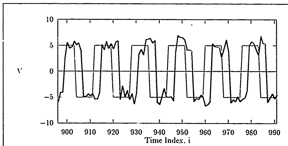
Figure 5.22. Signal Test 2: 3 - shift filter inputs. This is the last 96 samples of the noisy 3 - shift rectangular input and desired signal.
