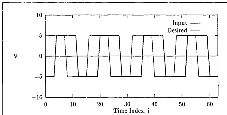
Figure 5.12. Signal Test 1: 4-shift filter inputs. This is the noiseless 4-shift rectangular input and desired signal.
