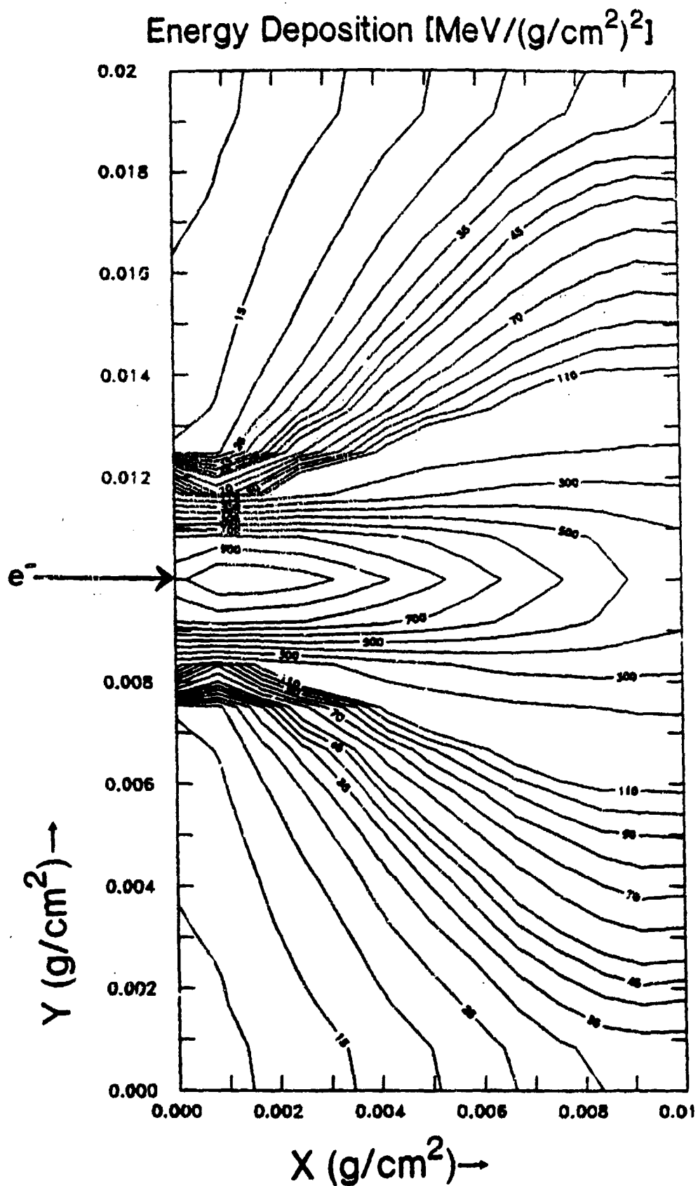
Figure 21. Energy deposition (isodose) contour plots for a 0.2 MeV electron beam normally incident on Al rectangle of dimension 0.02 g/cm 2 x 0.01 g/cm 2 (Ref. 22).
