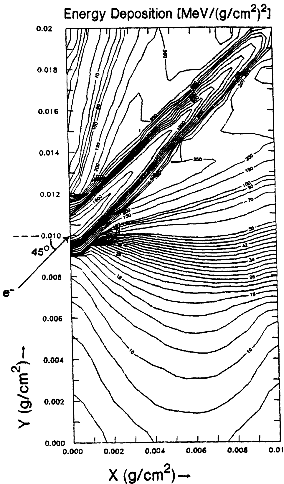
Figure 22. Energy deposition (isodose) contour plots for a 0.2 MeV electron beam incident at a 45° angle on Al rectangle of dimension 0.02 \text{ g/cm}^2 \times 0.01 \text{ g/cm}^2 (Ref. 22).
