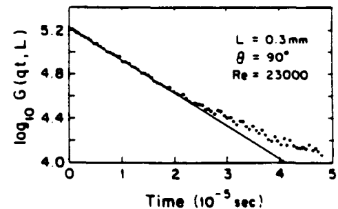
Fig. 5. A plot of \log[G(qt, L)] versus t in pipe flow at indicated parameters.
